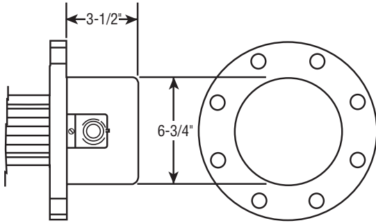
E1 GENERAL PURPOSE ENCLOSURE FOR UP TO 5" FLANGE
