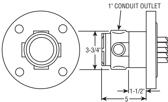
E4 MOISTURE RESISTANT ENCLOSURE WITH GASKET UP TO 5" FLANGE
