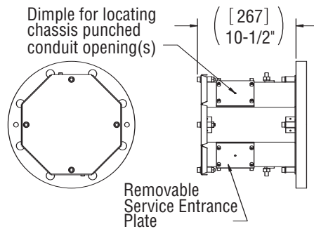
E4 MOISTURE RESISTANT ENCLOSURE WITH GASKET 6" AND LARGER FLANGE
