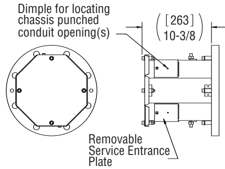
E1 GENERAL PURPOSE ENCLOSURE FOR 6" AND LARGER FLANGE
