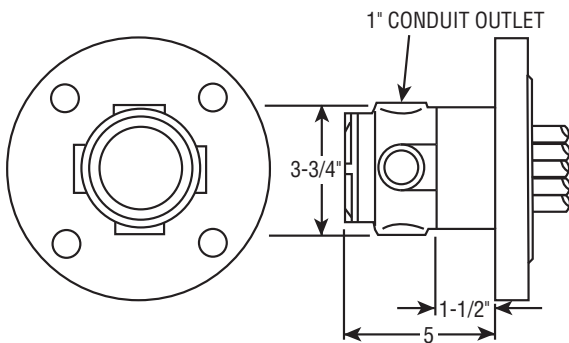
E2 EXPLOSION RESISTANT ENCLOSURE FOR UP TO 5" FLANGE
