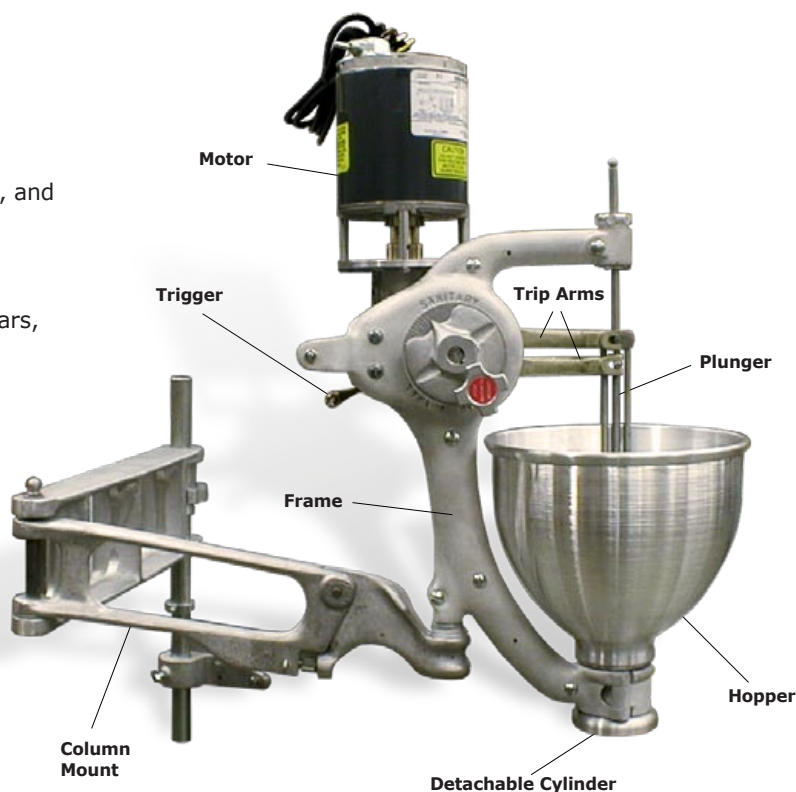
Top: Belshaw Type F (with optional plunger, cylinder, and column mount)
