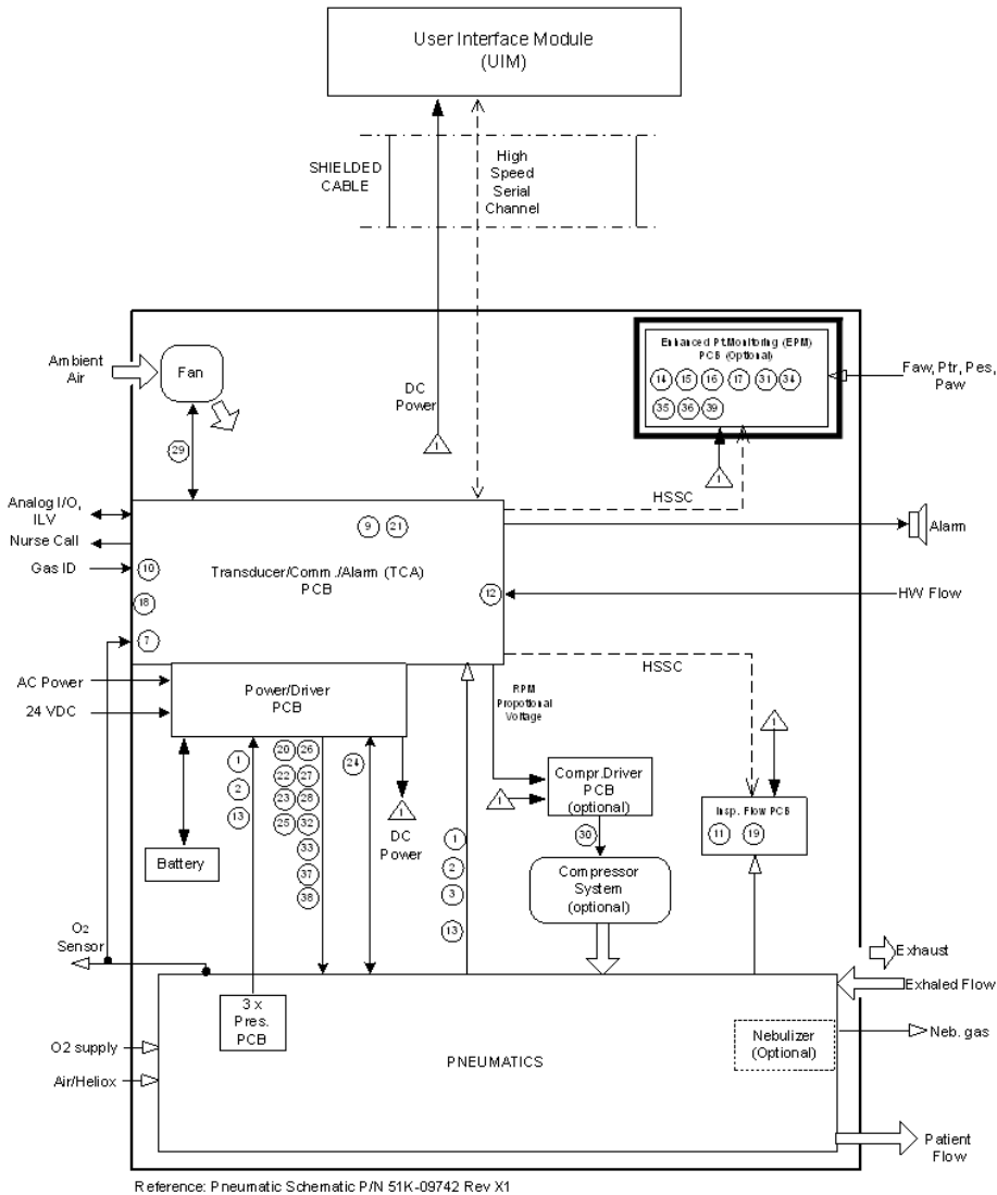
Figure 2.3 Pneumatics Module Block Diagram
