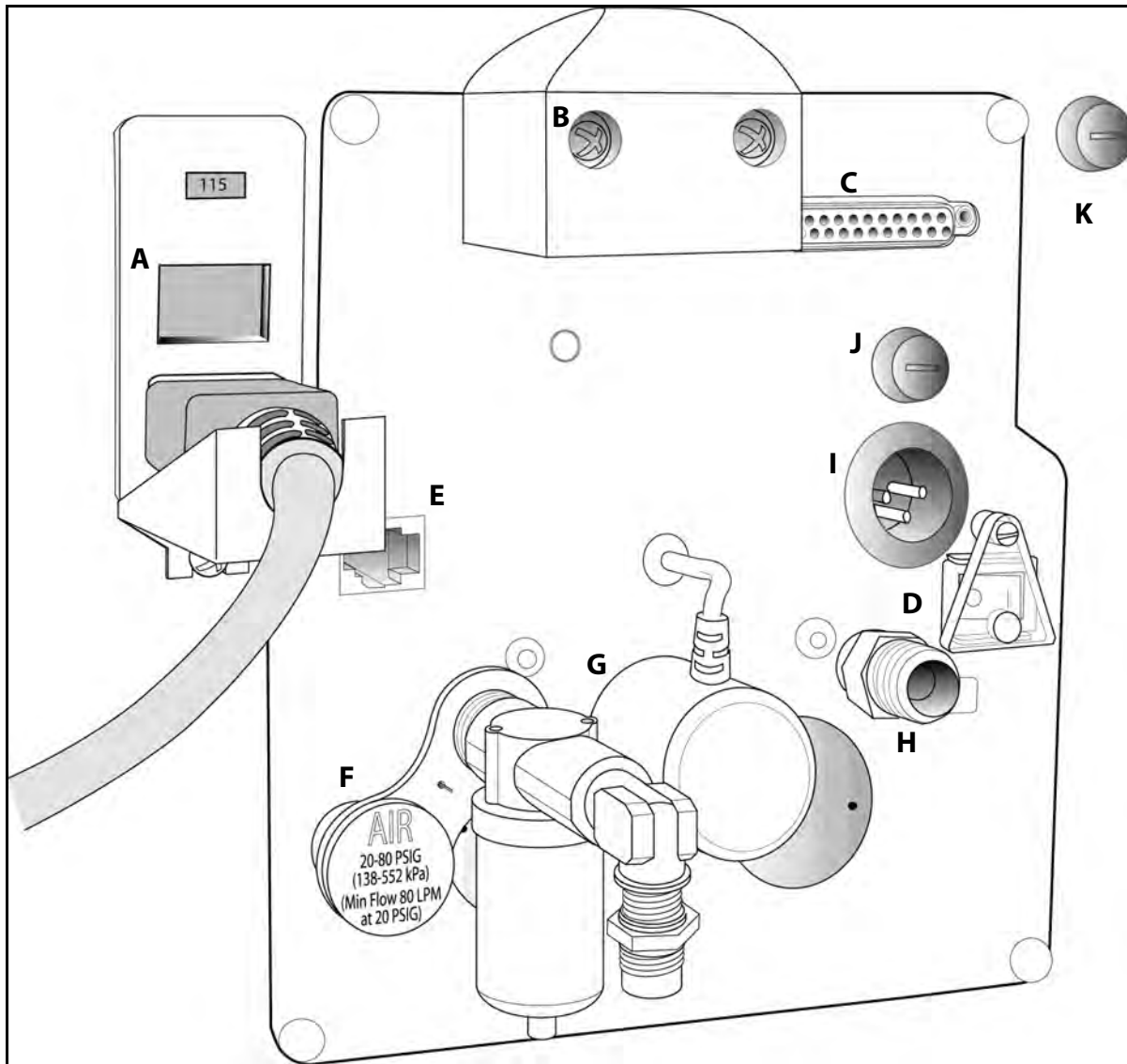
Figure 11.3 Rear Panel
