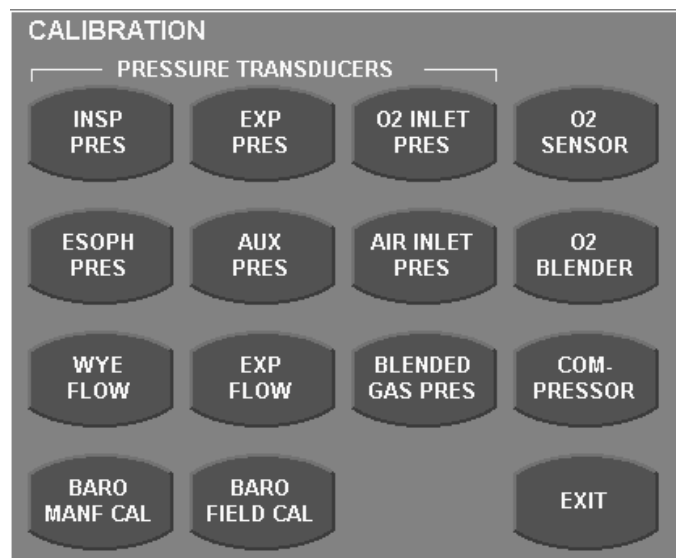
Figure 7.38 Calibration screen
