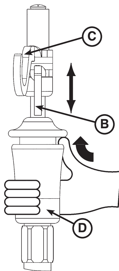
Figure 47: I.V. Pole Grip Detail
