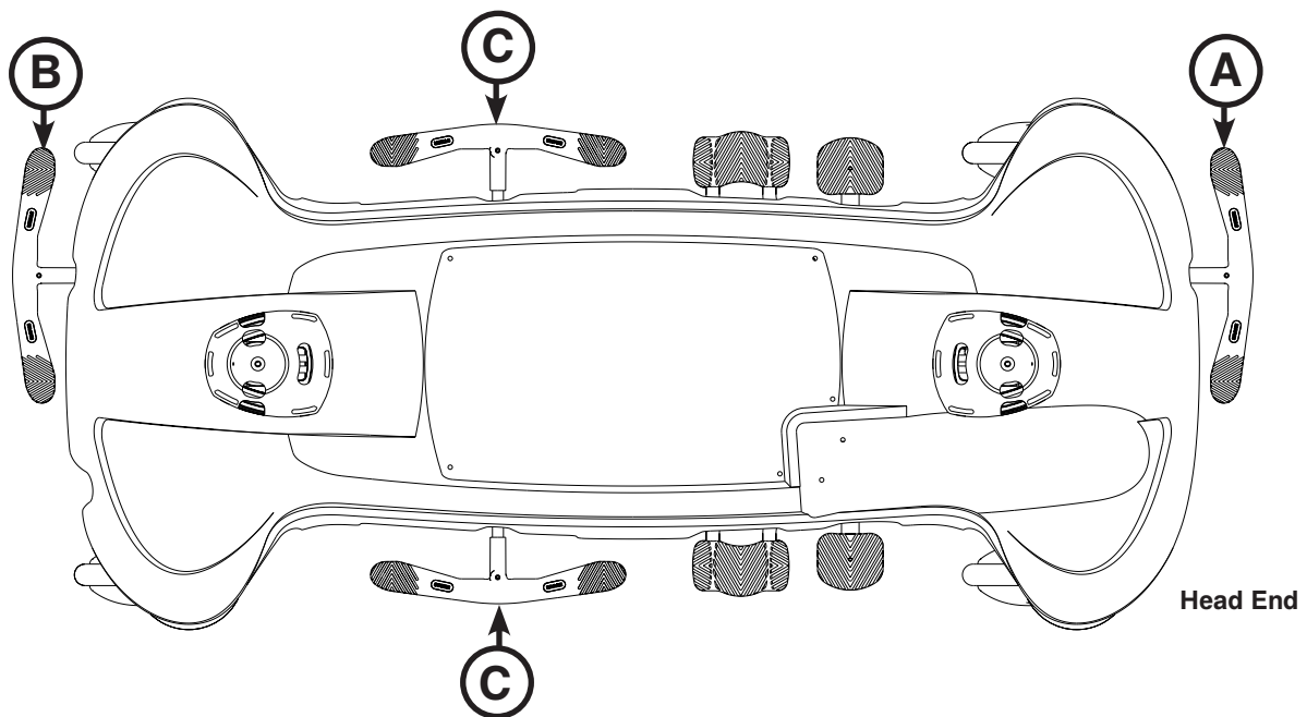
Figure 5: Steer/Brake Pedals
