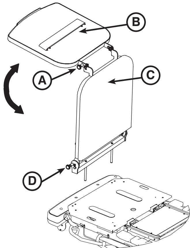
Figure 38: Foot Extension/ Defibrillator Tray - Foot End
