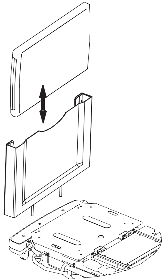
Figure 51: Serving Tray - Foot End
