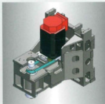
Belt Drive Spindle.
