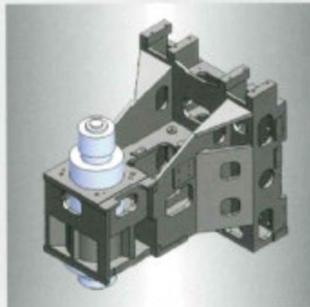
Built-In Drive-Spindle.
