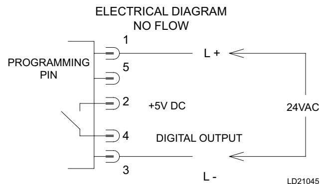
Figure 13: Wiring of Thermal Dispersion Flow Switch
