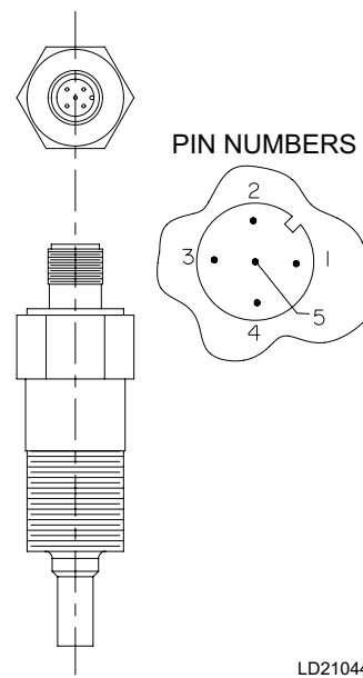
Figure 12: Thermal Dispersion Flow Switch
