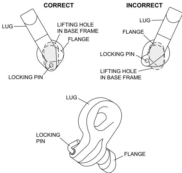
Figure 8: Lifting lugs
