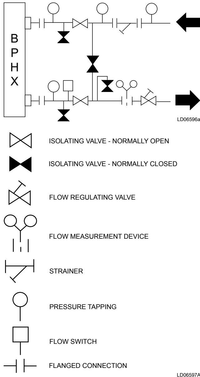
Figure 9: Chilled liquid system
