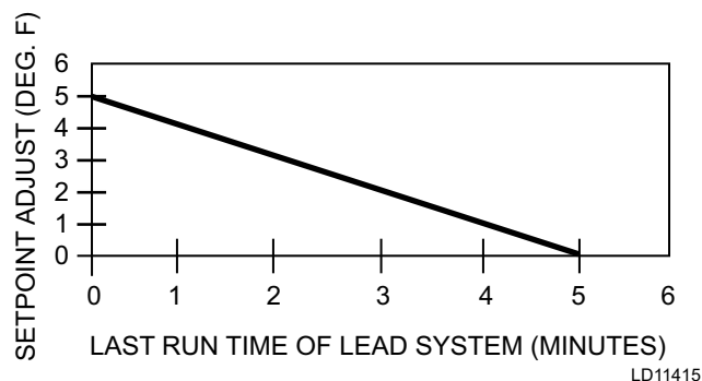
Figure 49: Setpoint Adjust
