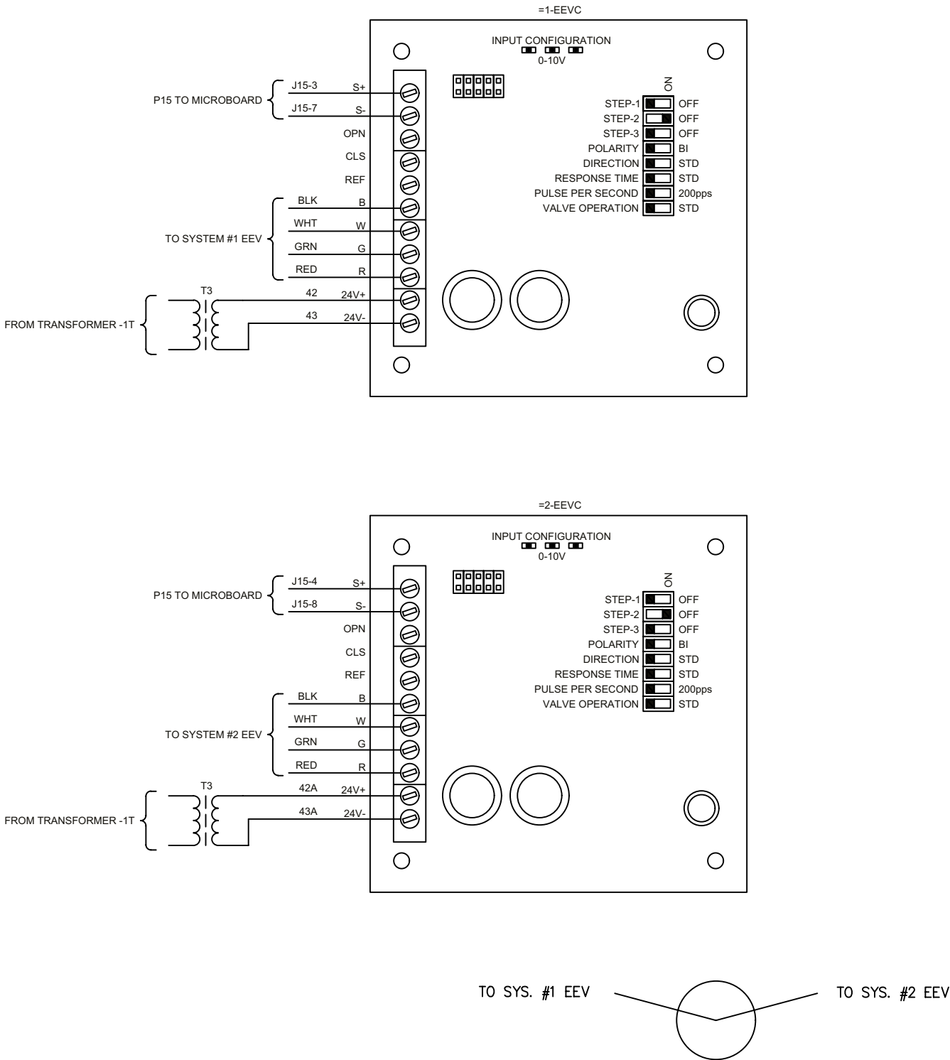
Figure 21: EEV Controller Elementary Diagram
