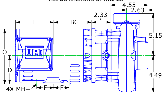
DRAWING DEPICTS JM14-18 ODP MOTOR ALL DIMENSIONS IN INCHES
