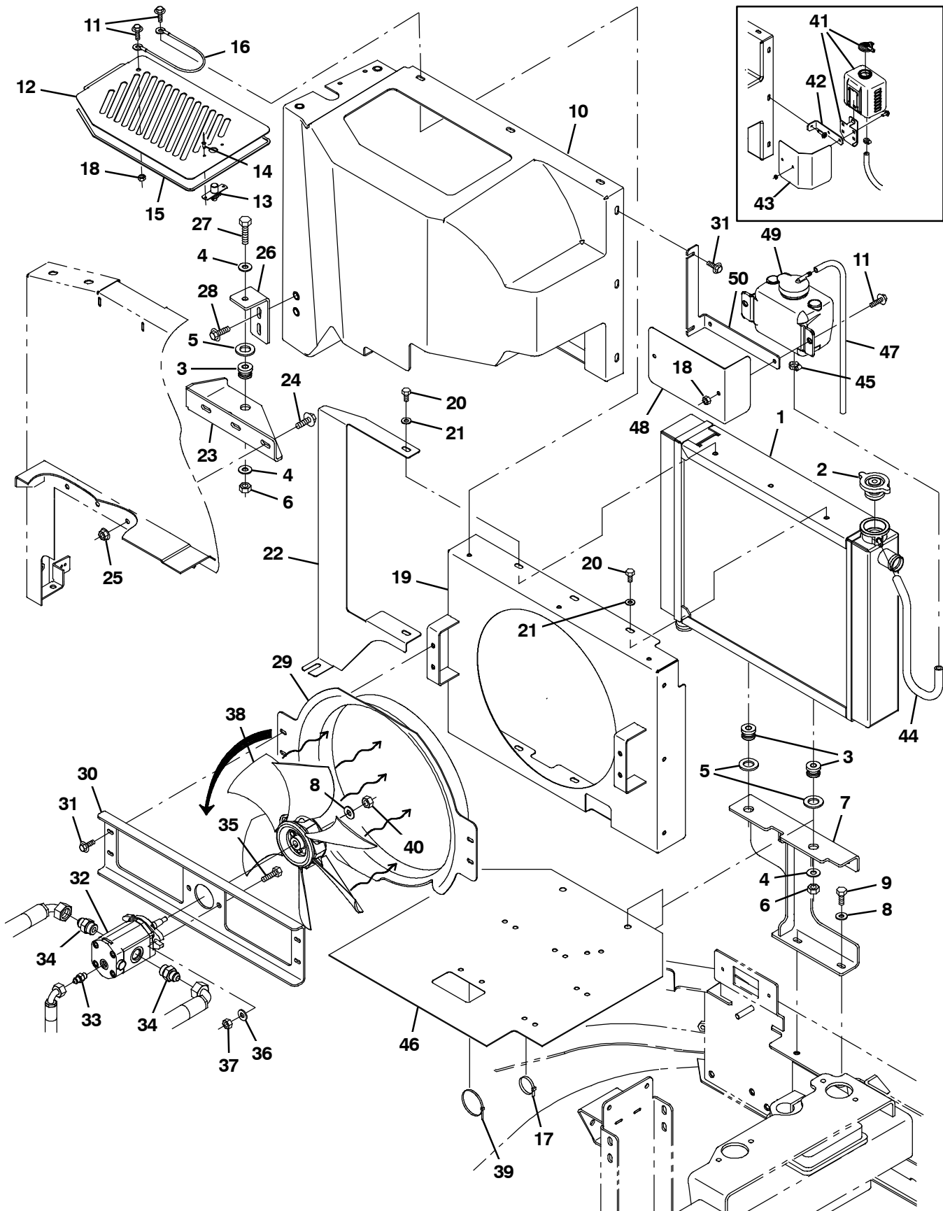
Fig. 26 - Engine Radiator Mount and Fan Group (000000-002099)
