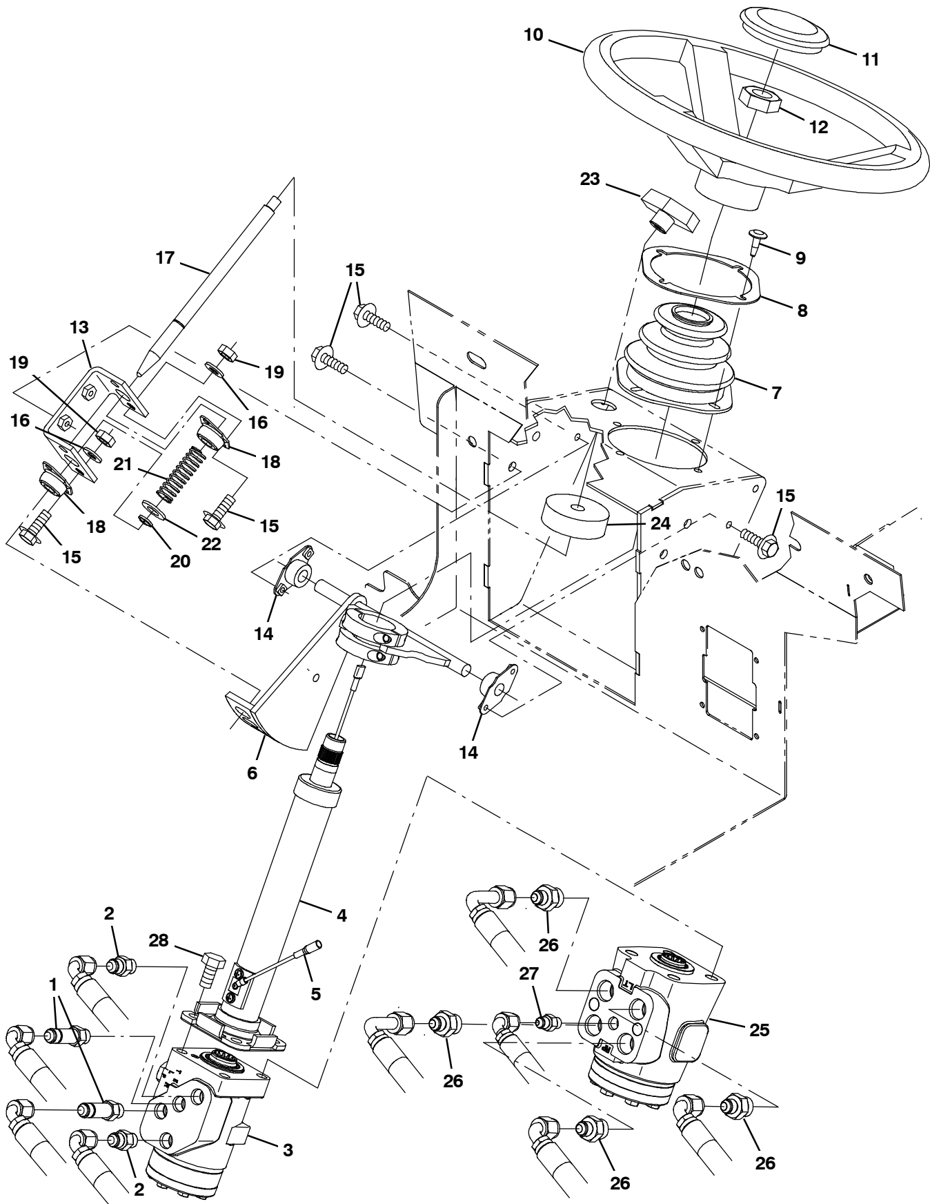
Fig. 17 - Steering Group (002100- )
