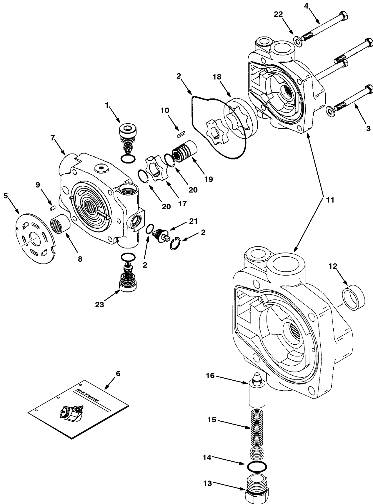
Fig. 12 - Hydraulic Piston Pump Breakdown, 1029255
