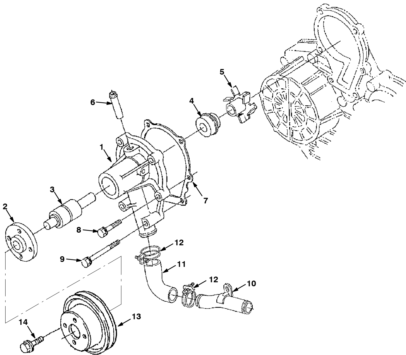
Fig. 5 - Water Pump Group
