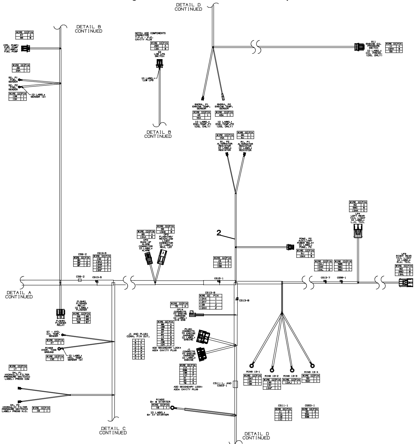
Fig. 79 - Electrical Wire Harnesses Group
