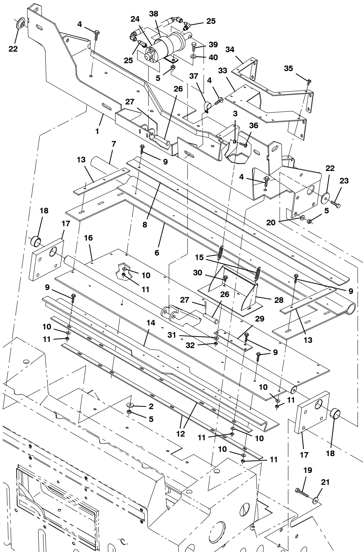
Fig. 41 - Hopper Cylinder and Dump Door Group, Plastic
