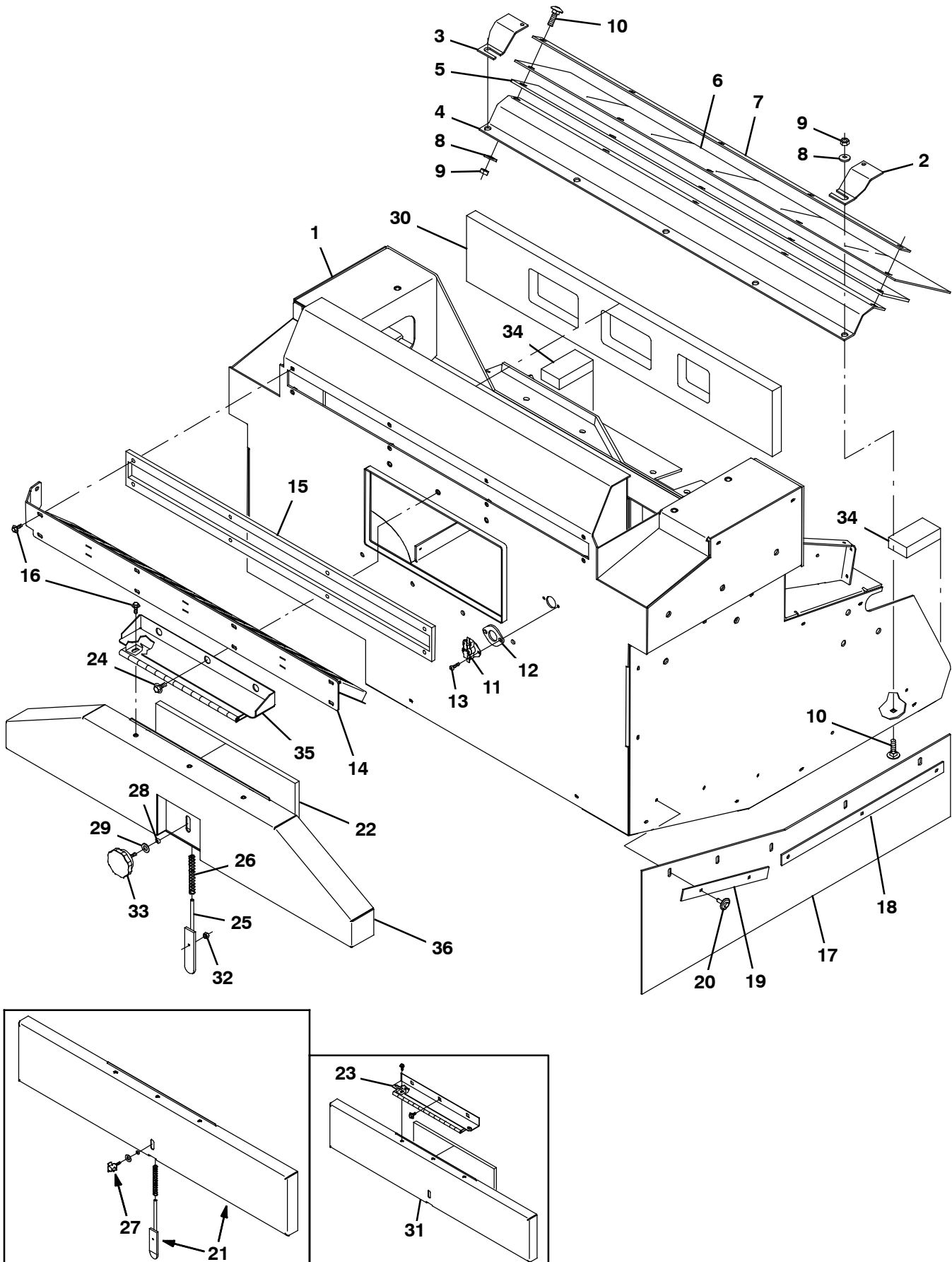
Fig. 40 - Hopper Group, Steel
