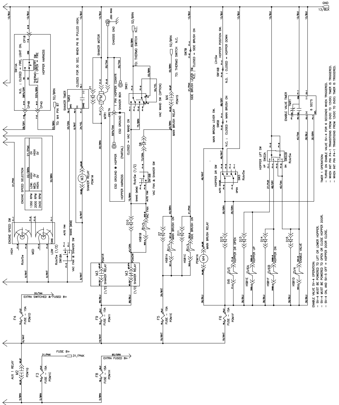
Fig. 74 - Electrical Schematic, S30 (000000-005699) (2 of 4)
