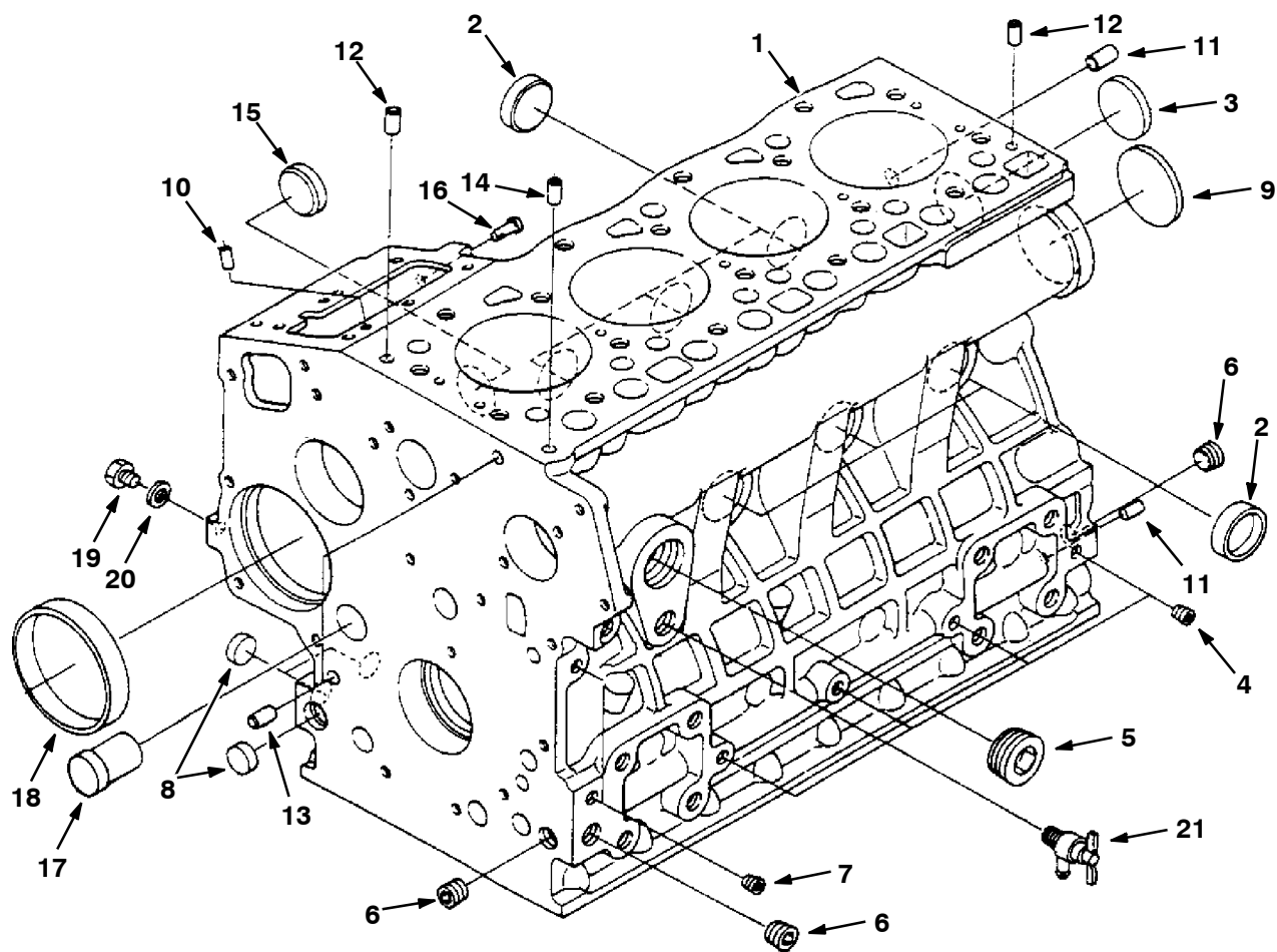
Fig. 1 - Crankcase Group
