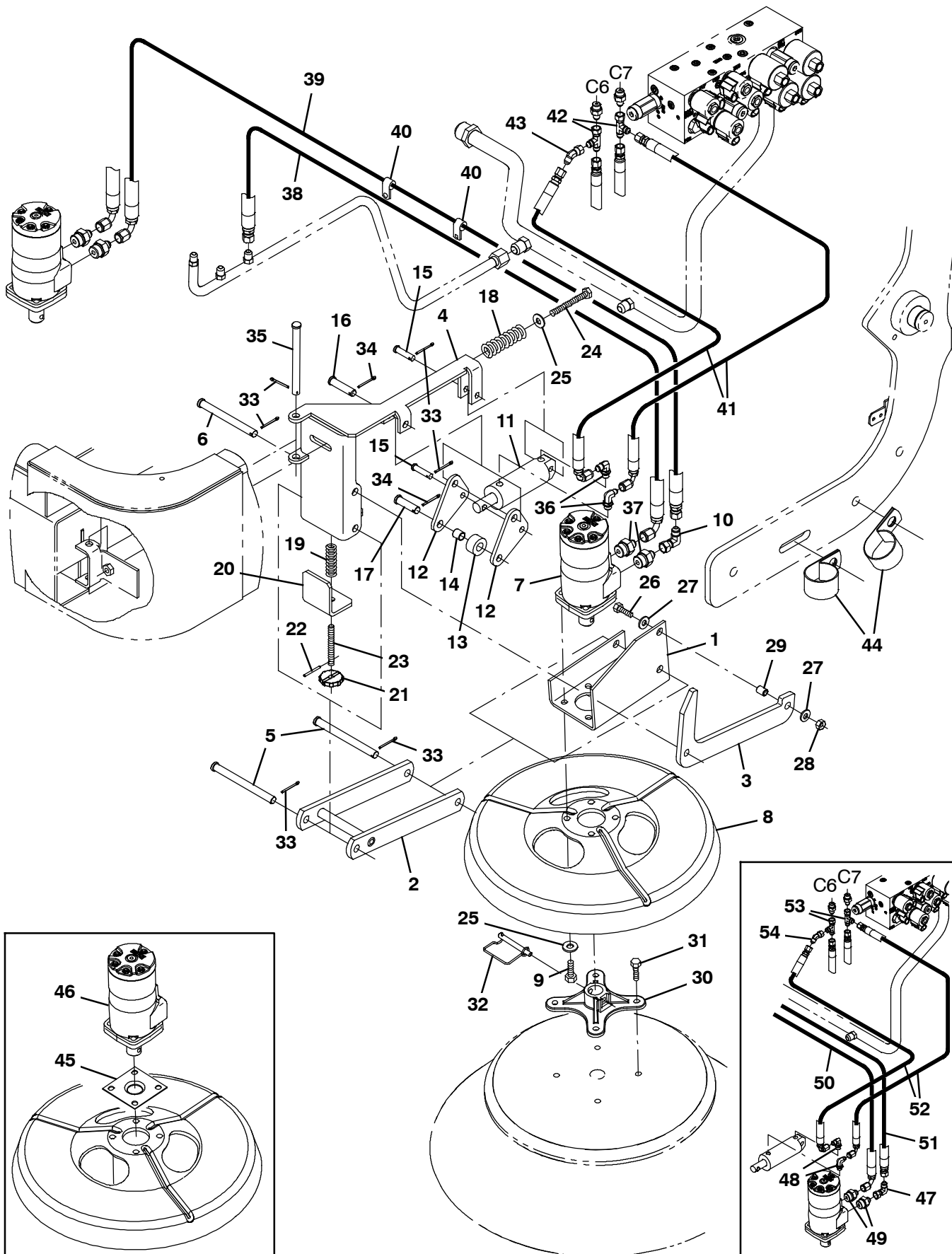
Fig. 5 - Left Hand Side Brush Kit, S30 XP and X4
