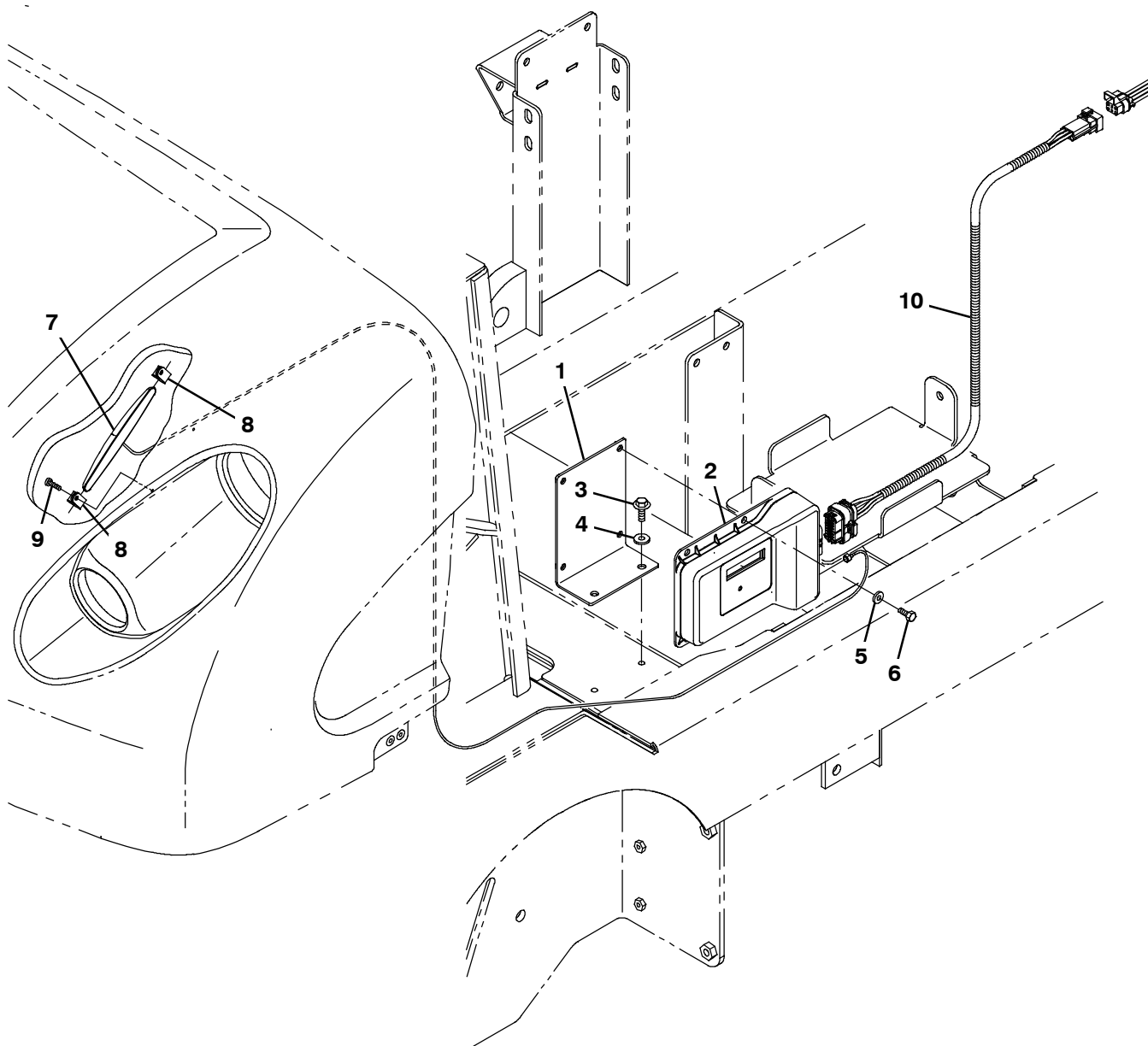
Fig. 20 - Telemetry Group
