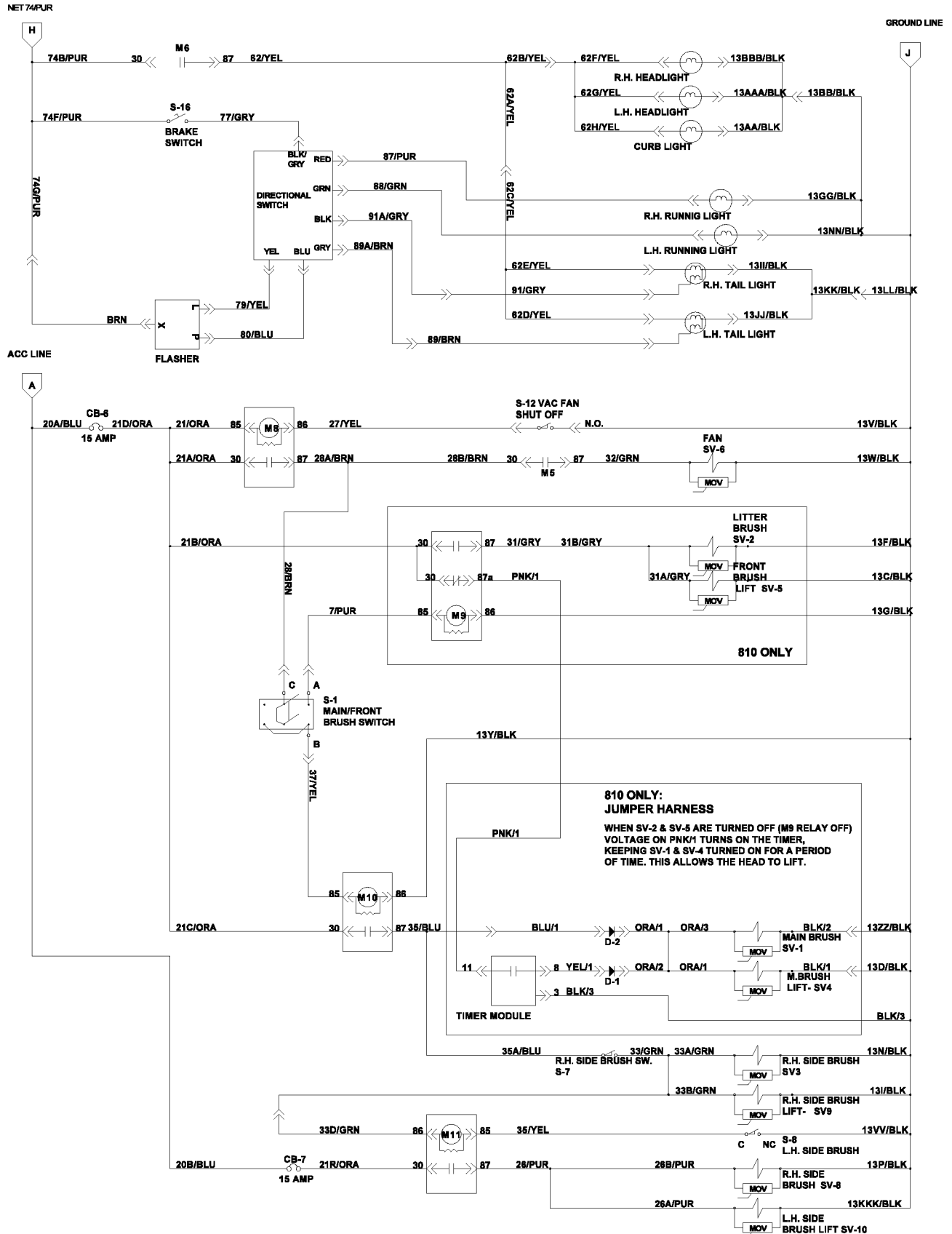
Fig. 93 - Electrical Schematic (004937-005999)
