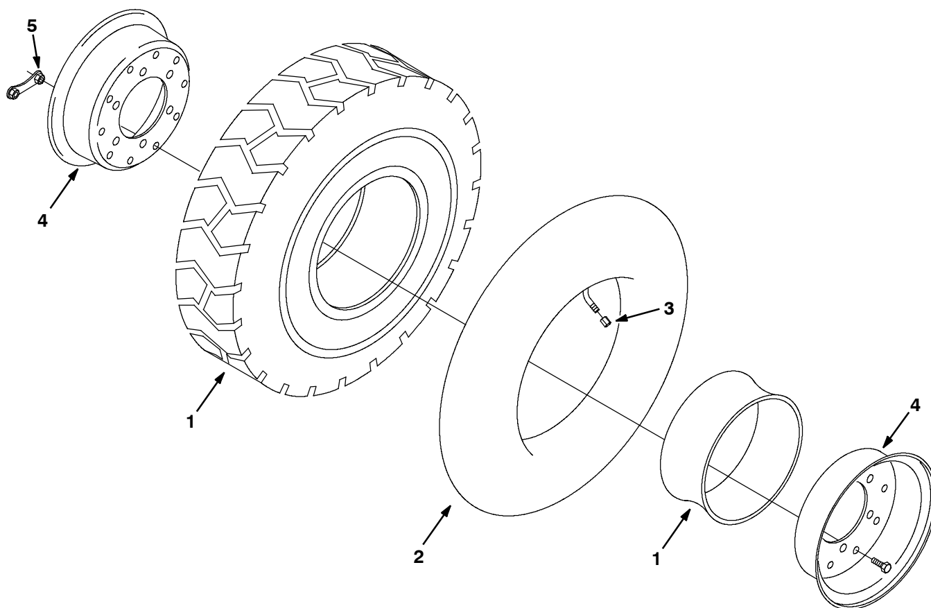
Fig. 70 - Wheel Assembly
