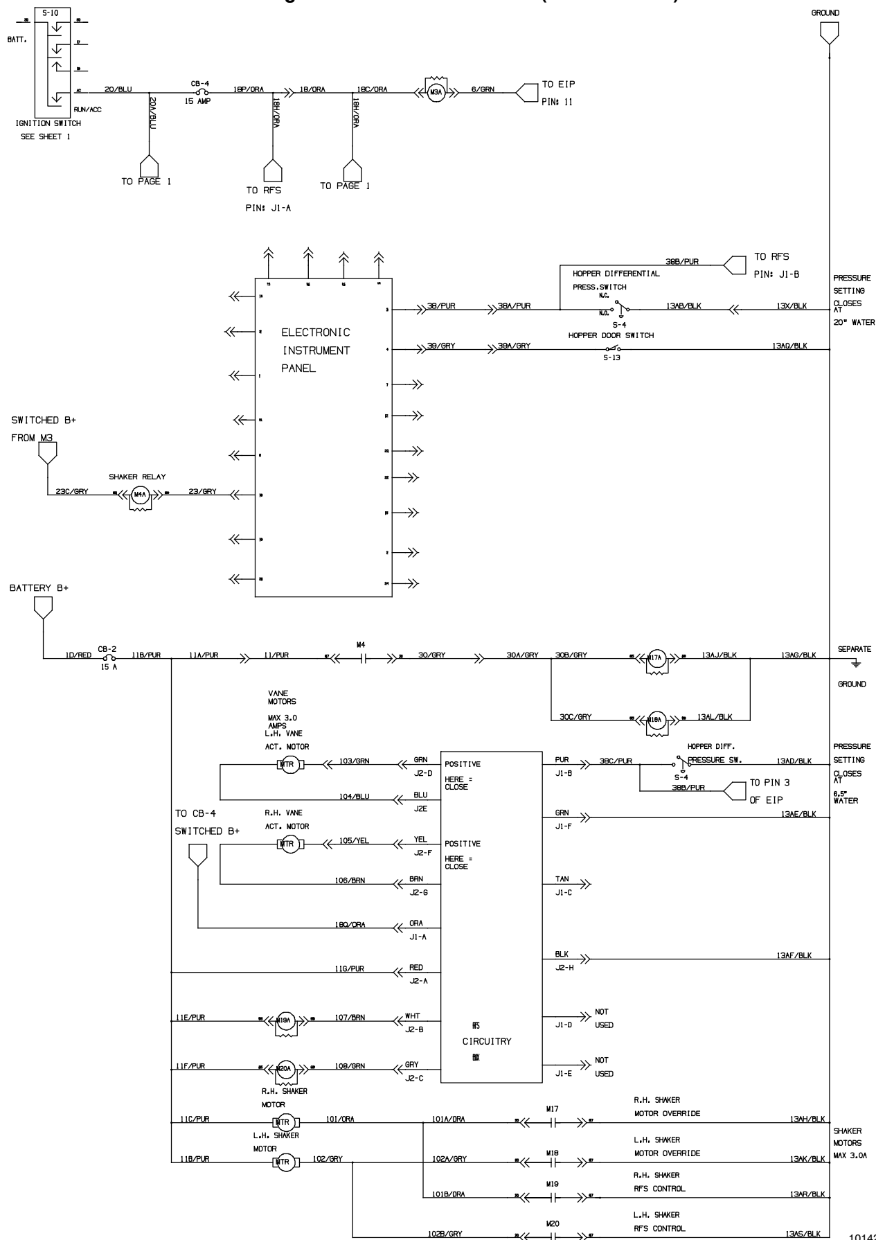
Fig. 94 - Electrical Schematic (006000- )
