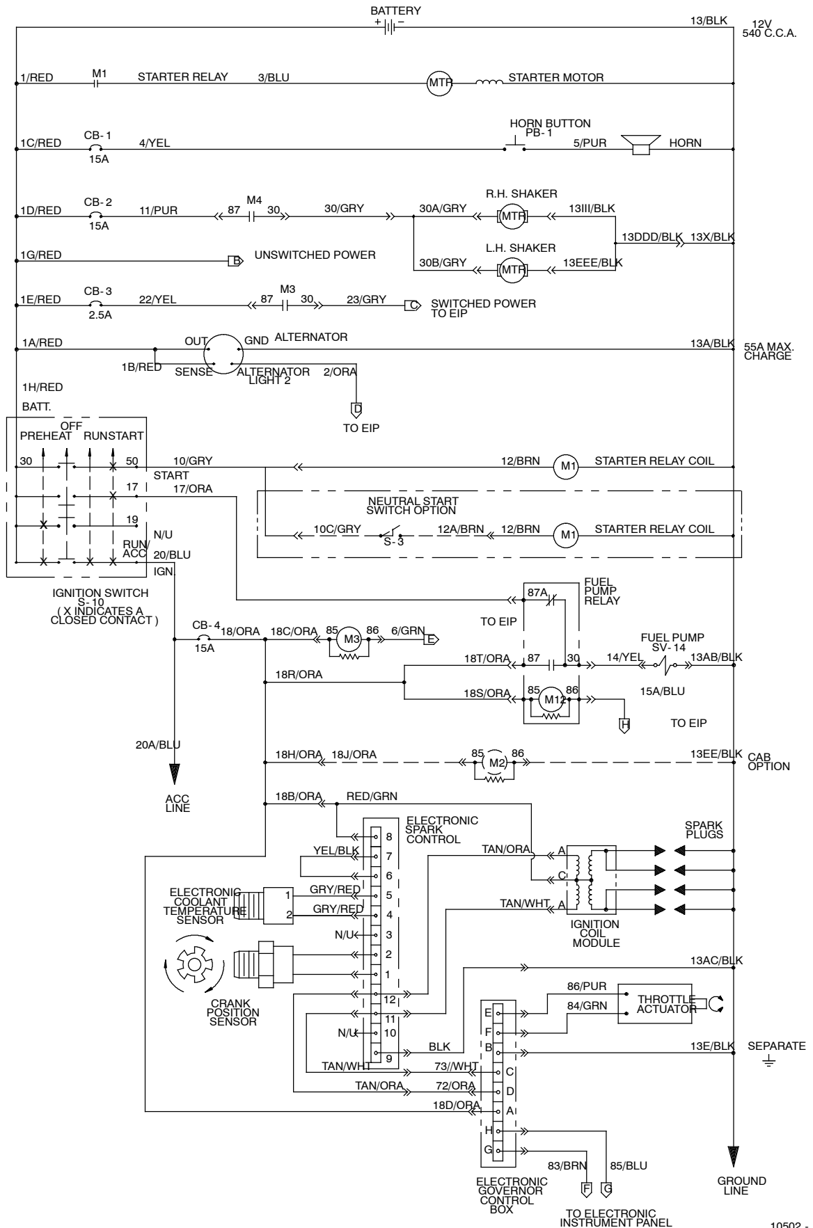
Fig. 92 - Electrical Schematic (004000-004936)
