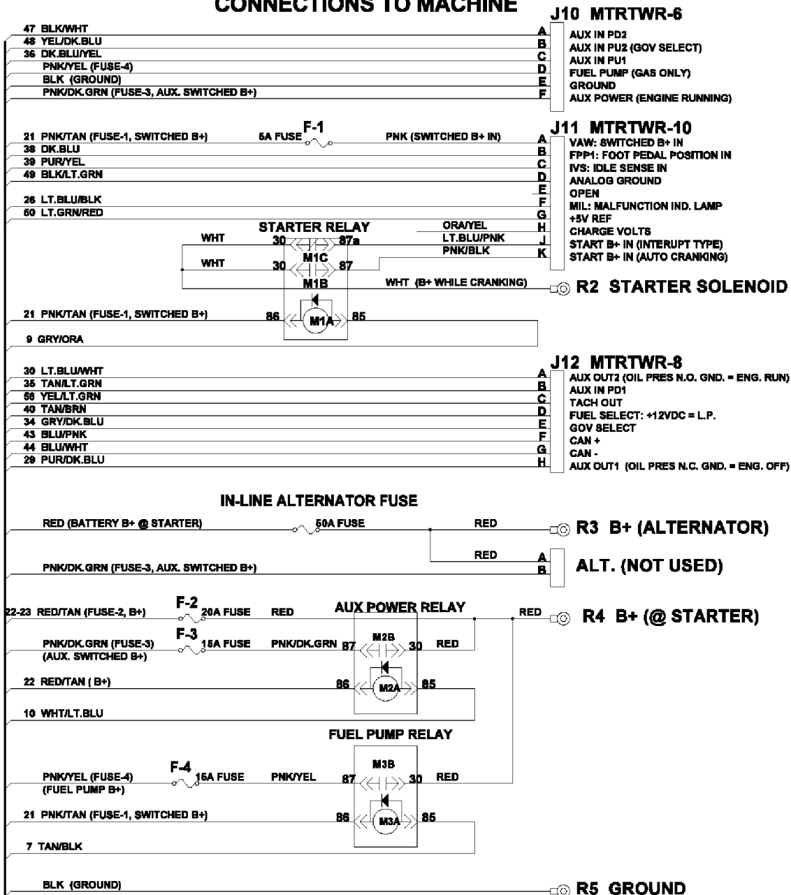
Fig. 94 - Electrical Schematic (006000- )
