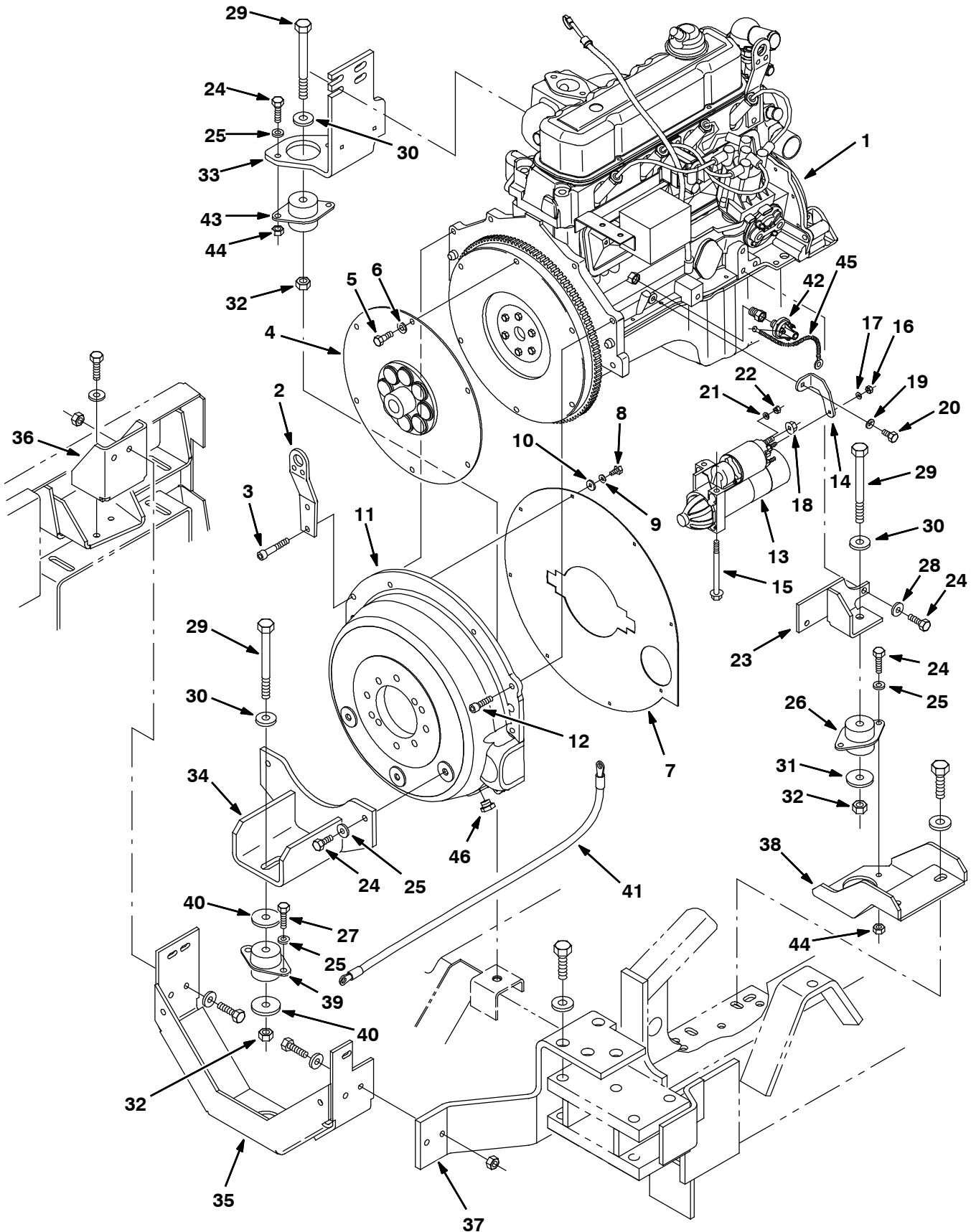
Fig. 23 - Engine Group (006000-006999)
