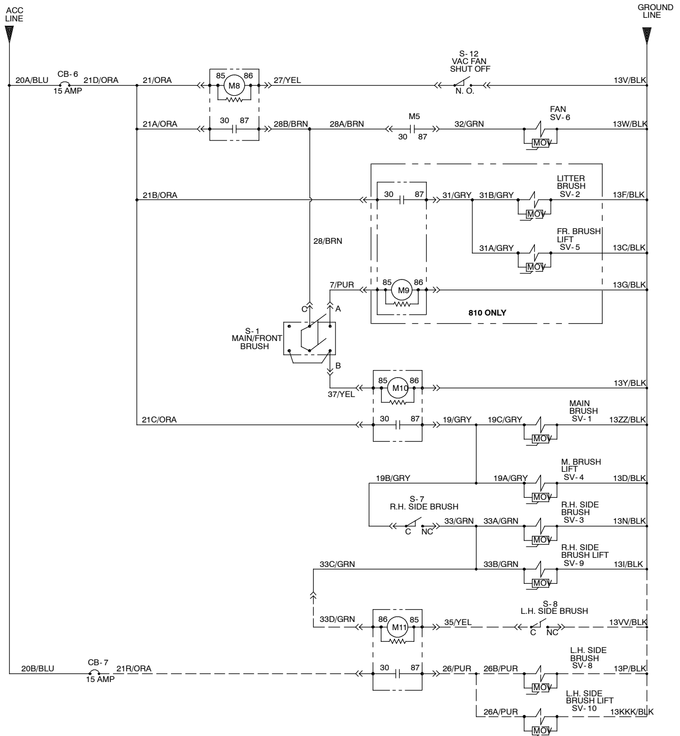
Fig. 92 - Electrical Schematic (004000-004936)
