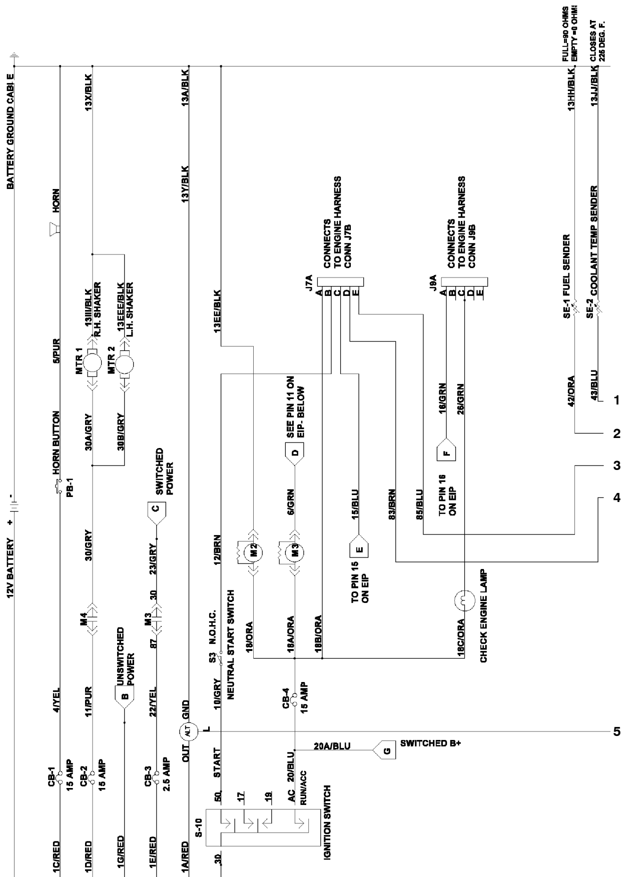
Fig. 93 - Electrical Schematic (004937-005999)
