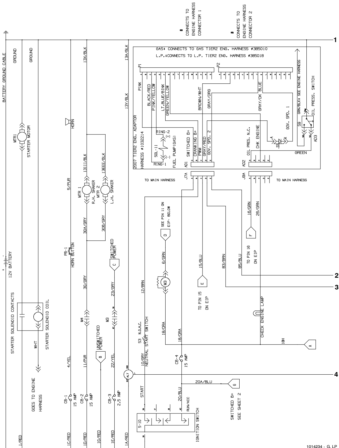
Fig. 94 - Electrical Schematic (006000- )
