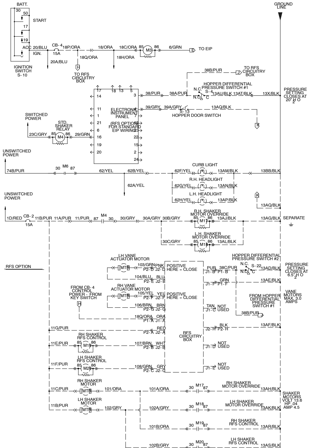
Fig. 92 - Electrical Schematic (004000-004936)
