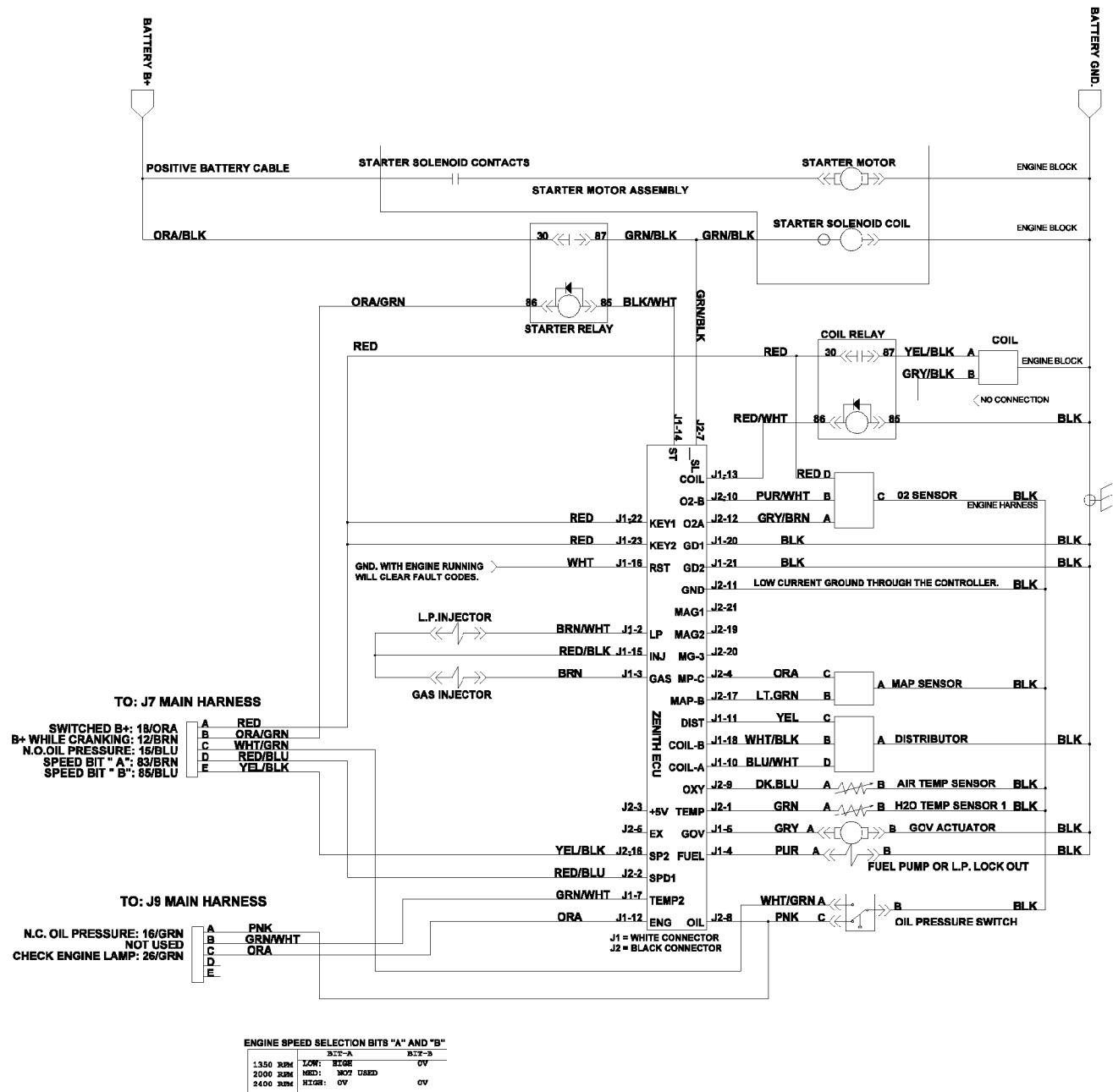
Fig. 93 - Electrical Schematic (004937-005999)
