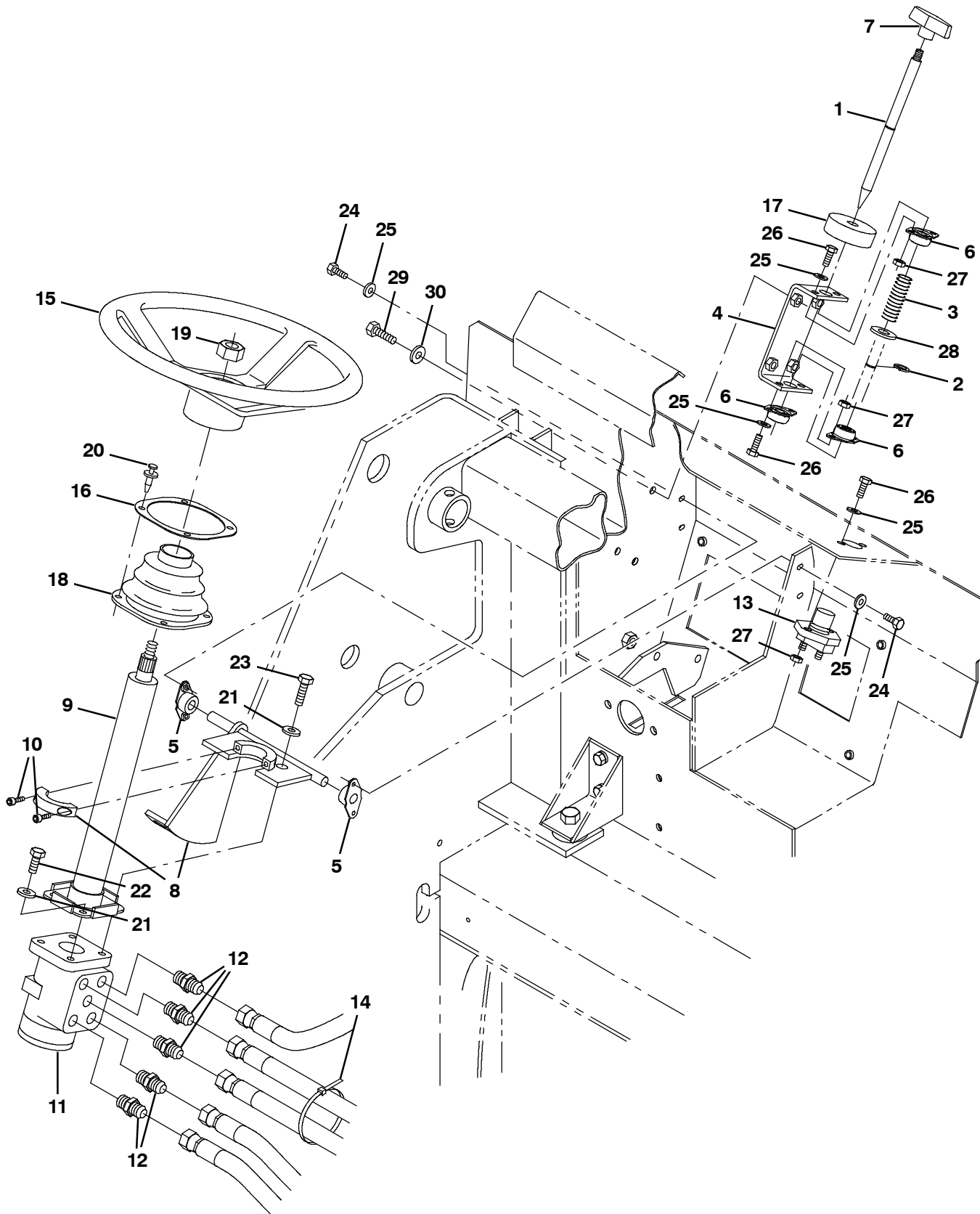
Fig. 89 - Steering Group
