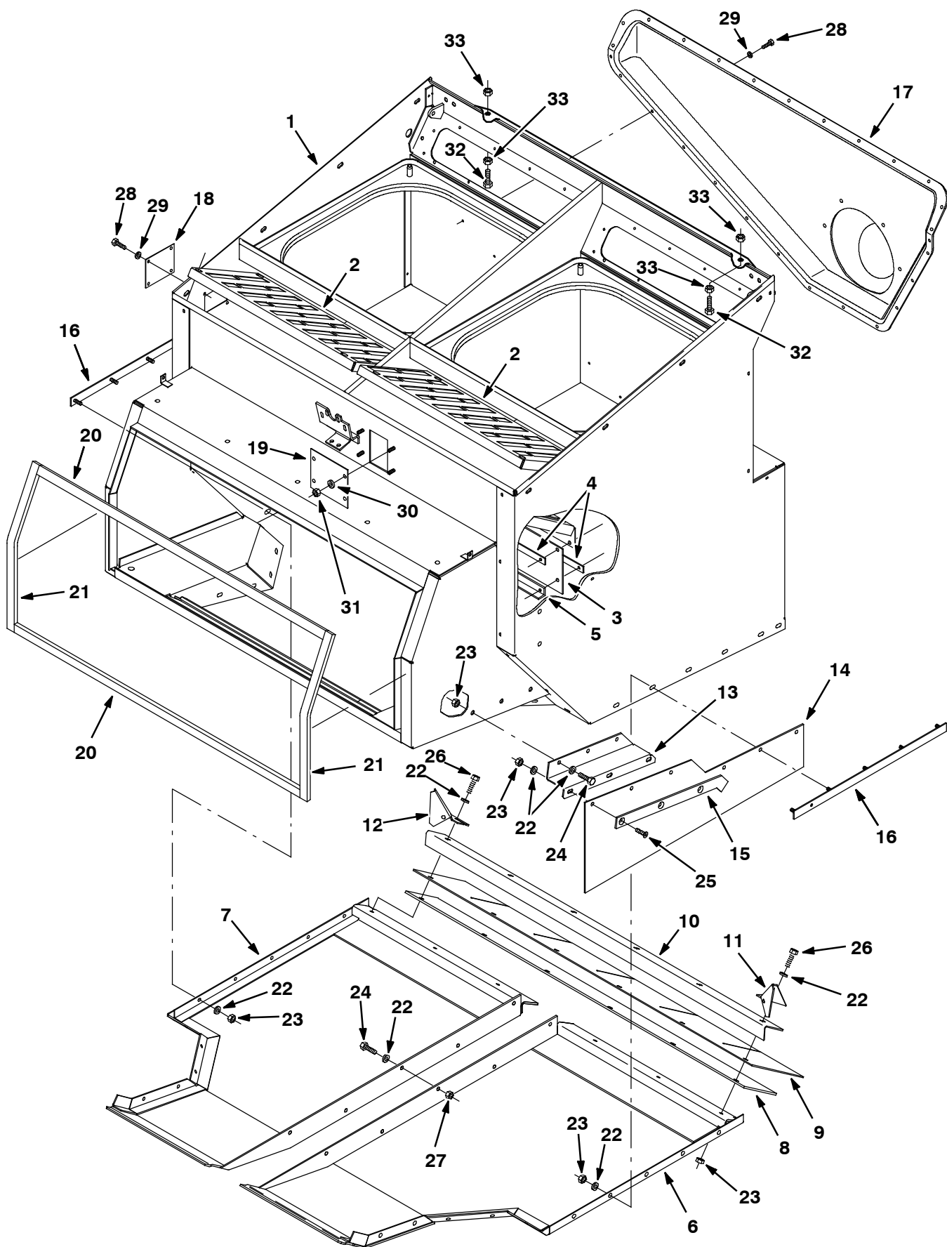
Fig. 14 - Hopper Group
