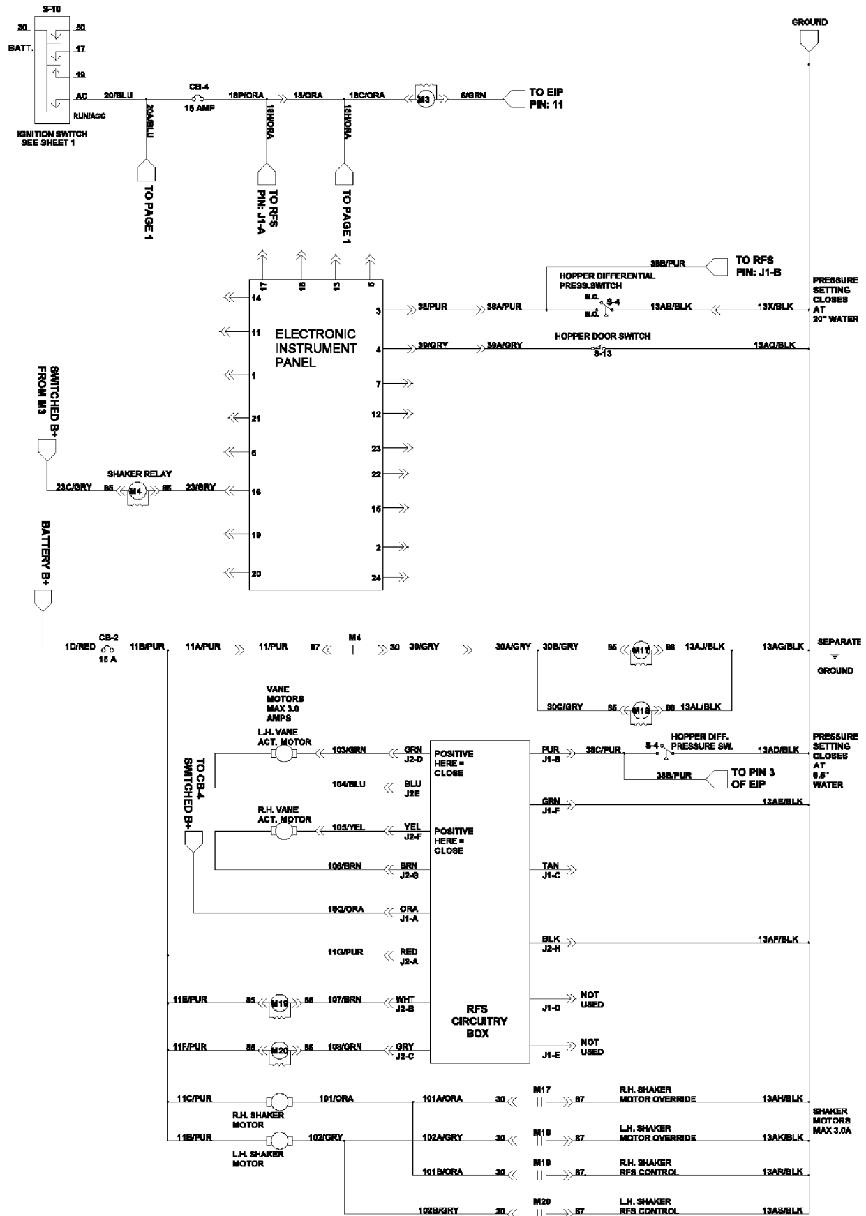
Fig. 93 - Electrical Schematic (004937-005999)
