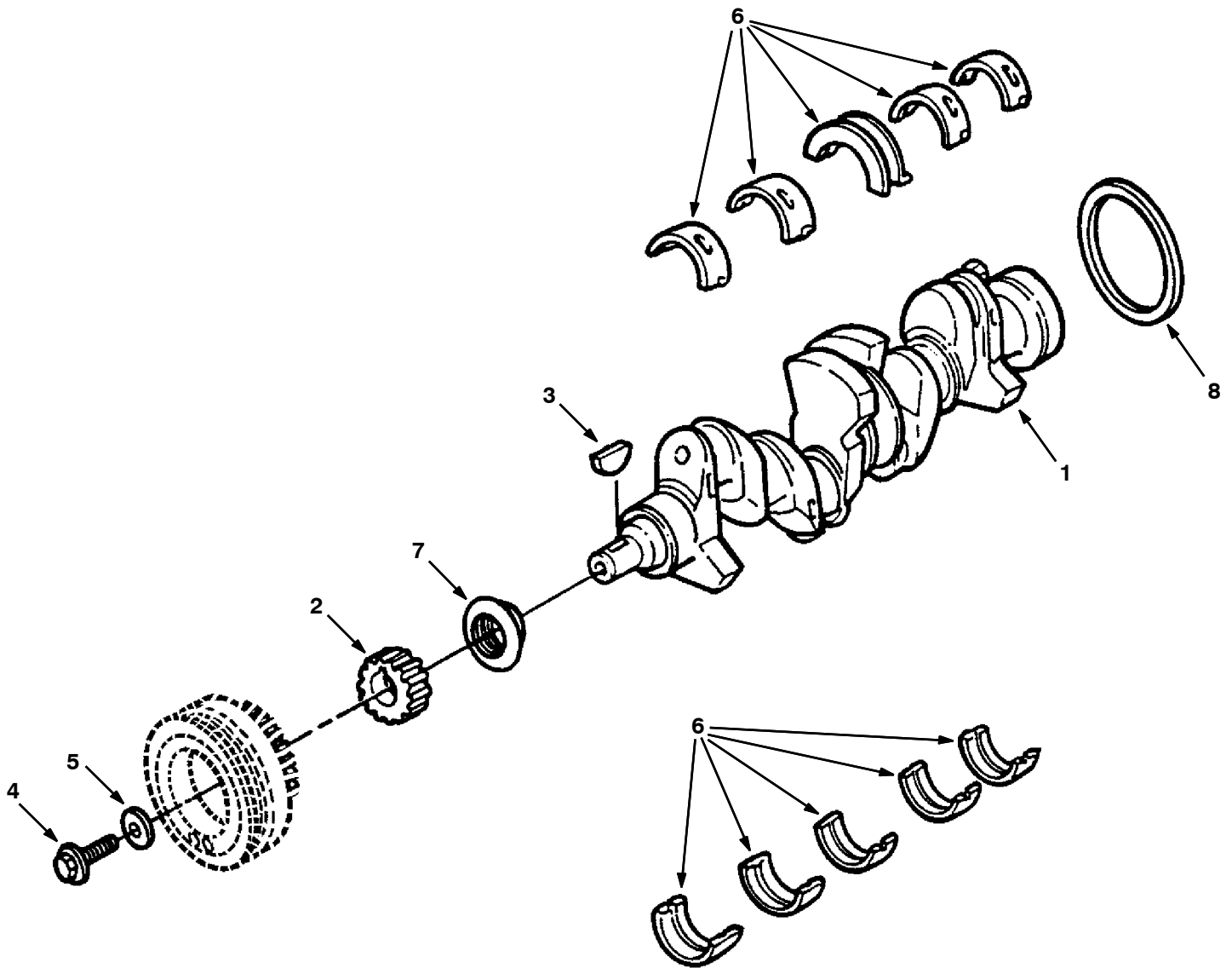
Fig. 7 - Crankshaft Group
