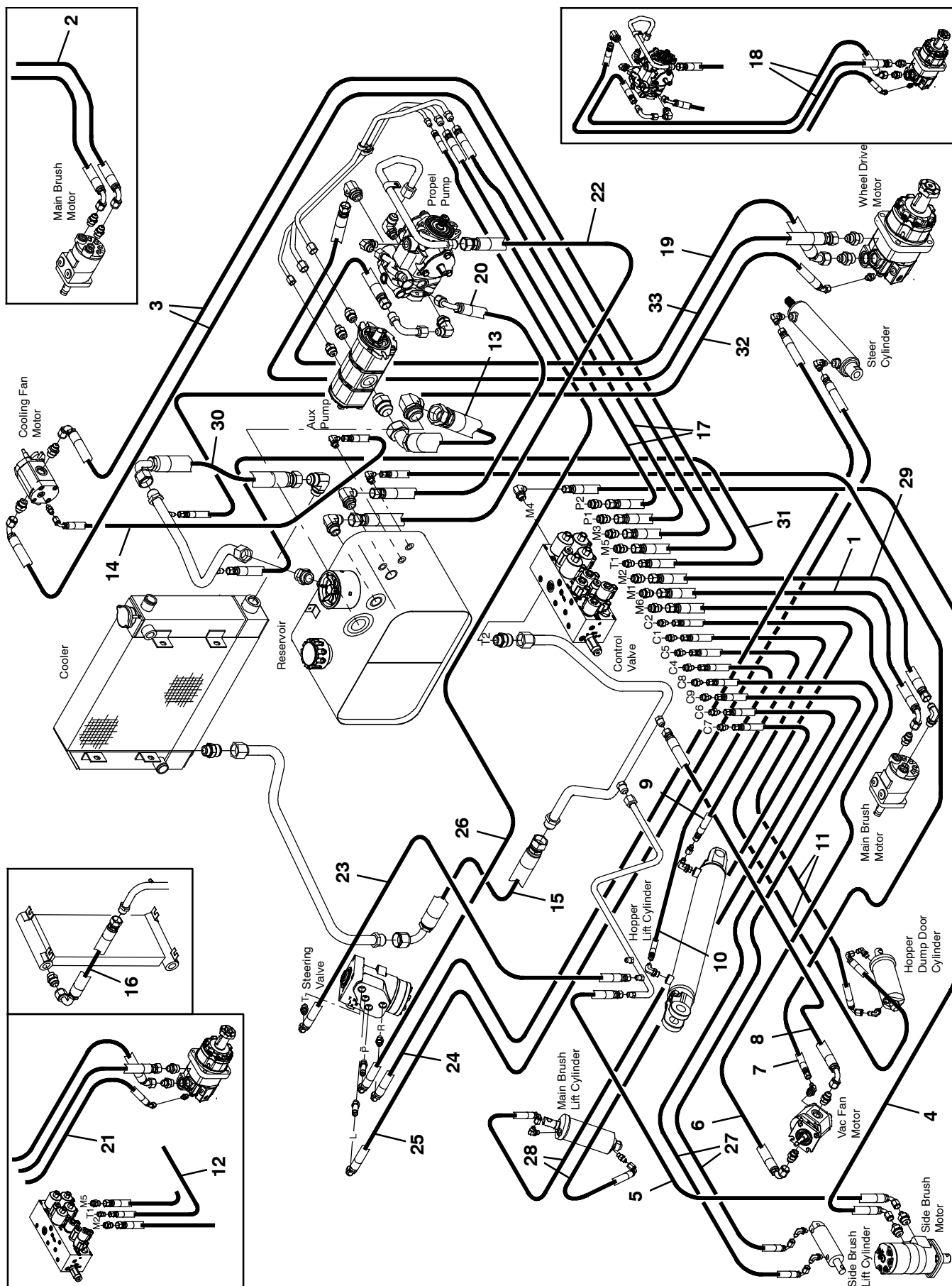
Fig. 72 - Hydraulic Hose Group, S30 XP (000000-002999)
