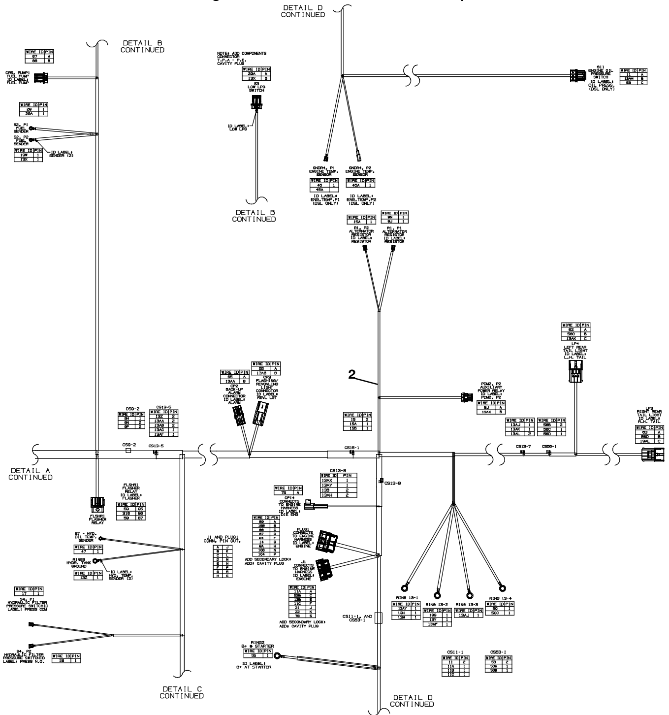
Fig. 88 - Electrical Wire Harnesses Group
