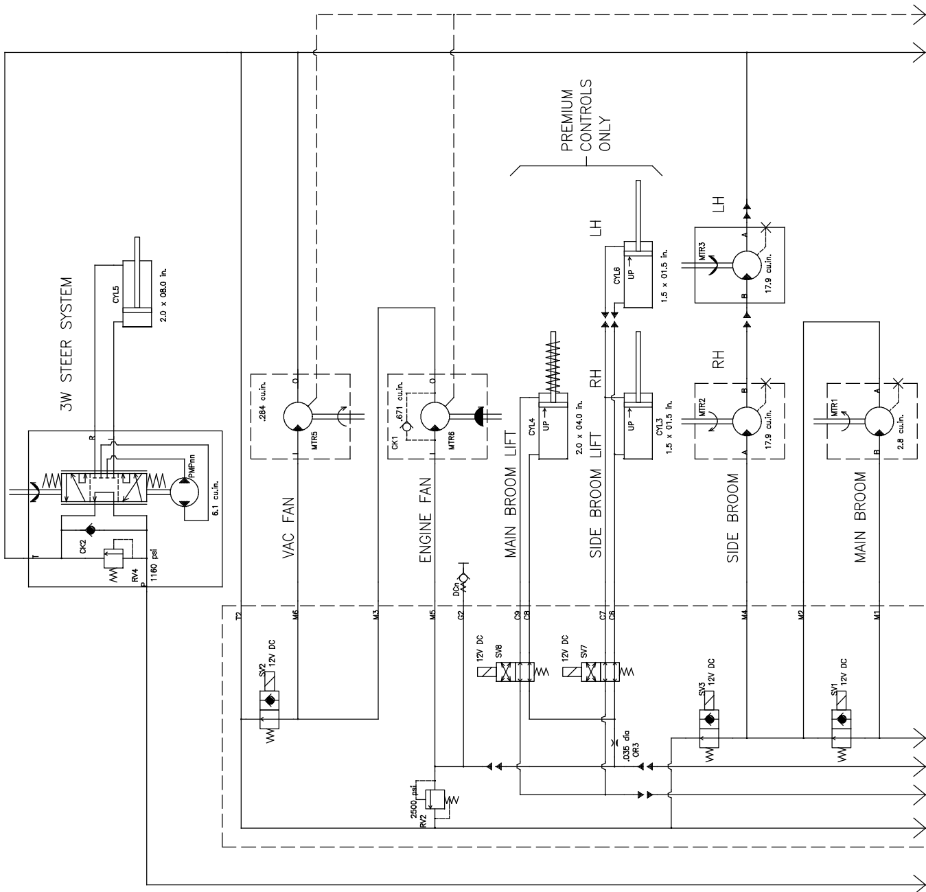
Fig. 69 - Hydraulic Schematic
