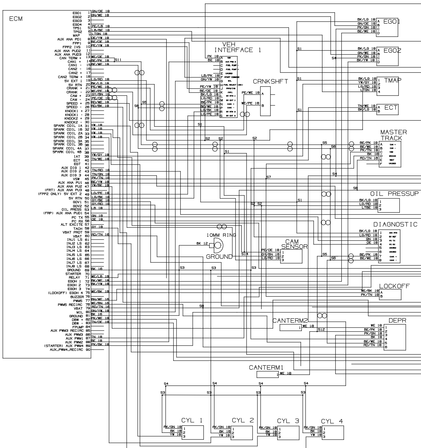
Fig. 87 - Electrical Schematic, LPG Engine Harness, Mitsubishi (005700- ) (1 of 2)
