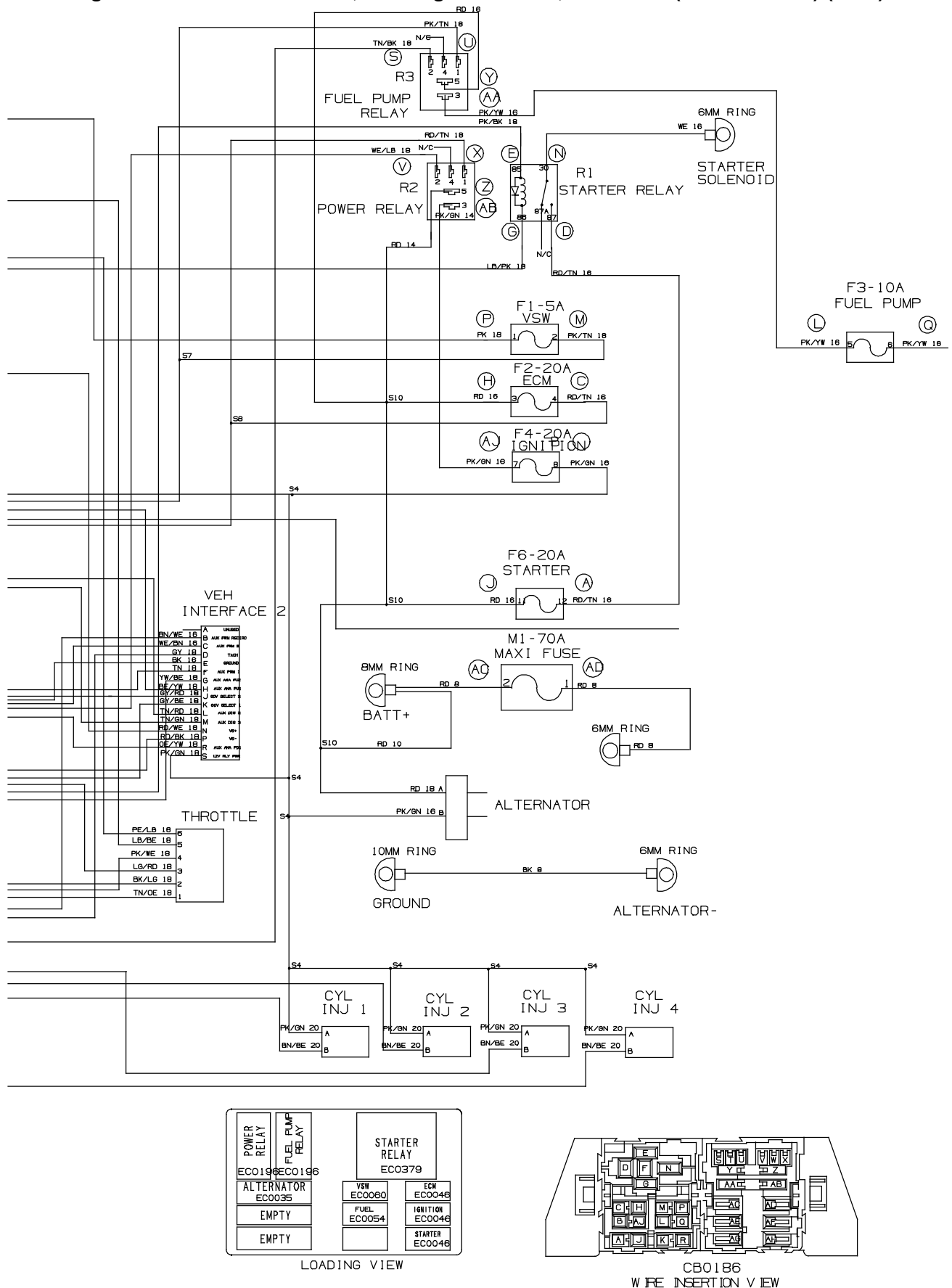
Fig. 85 - Electrical Schematic, Gas Engine Harness, Mitsubishi (005700- ) (2 of2)
