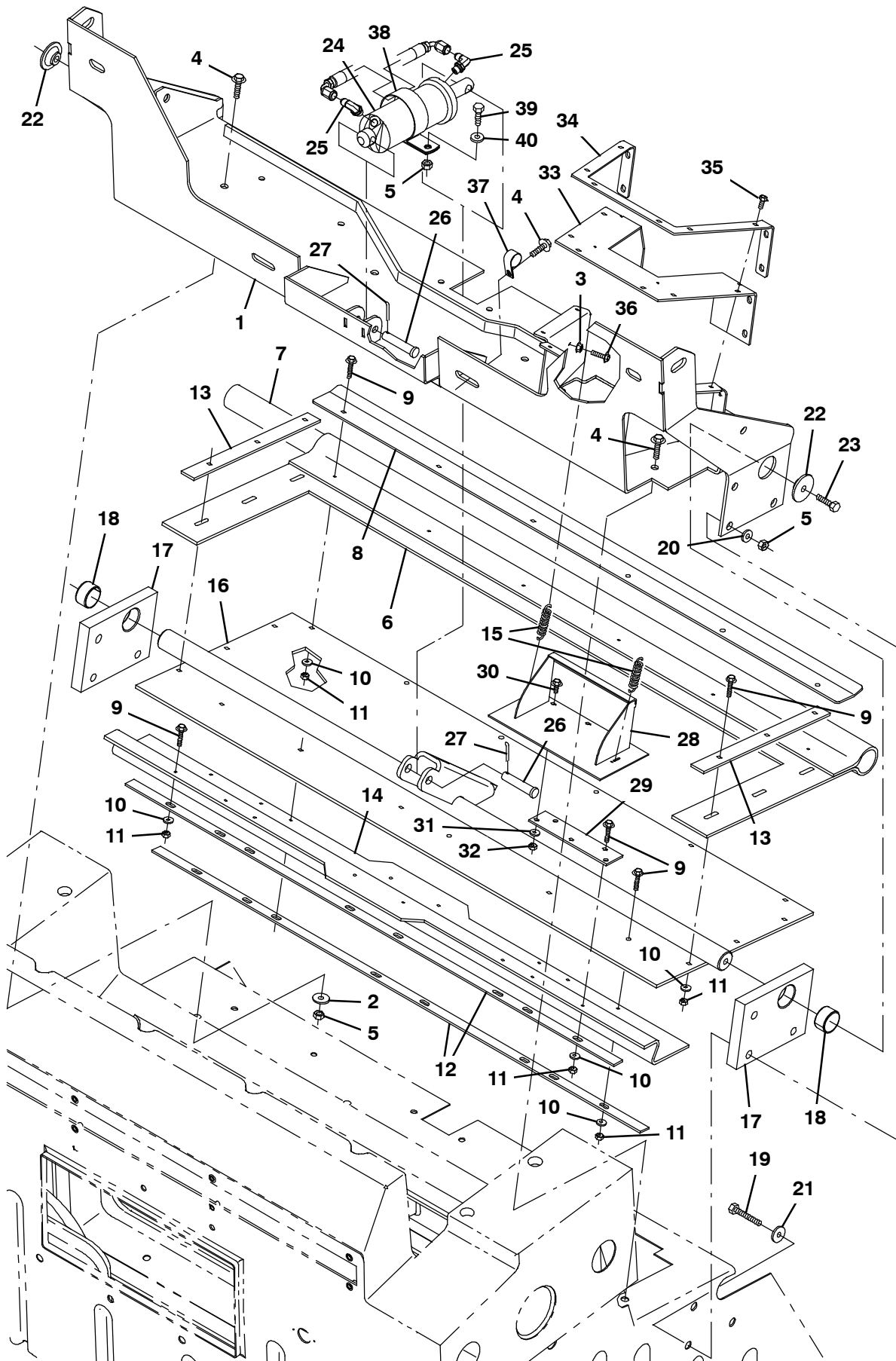
Fig. 52 - Hopper Cylinder and Dump Door Group, Plastic
