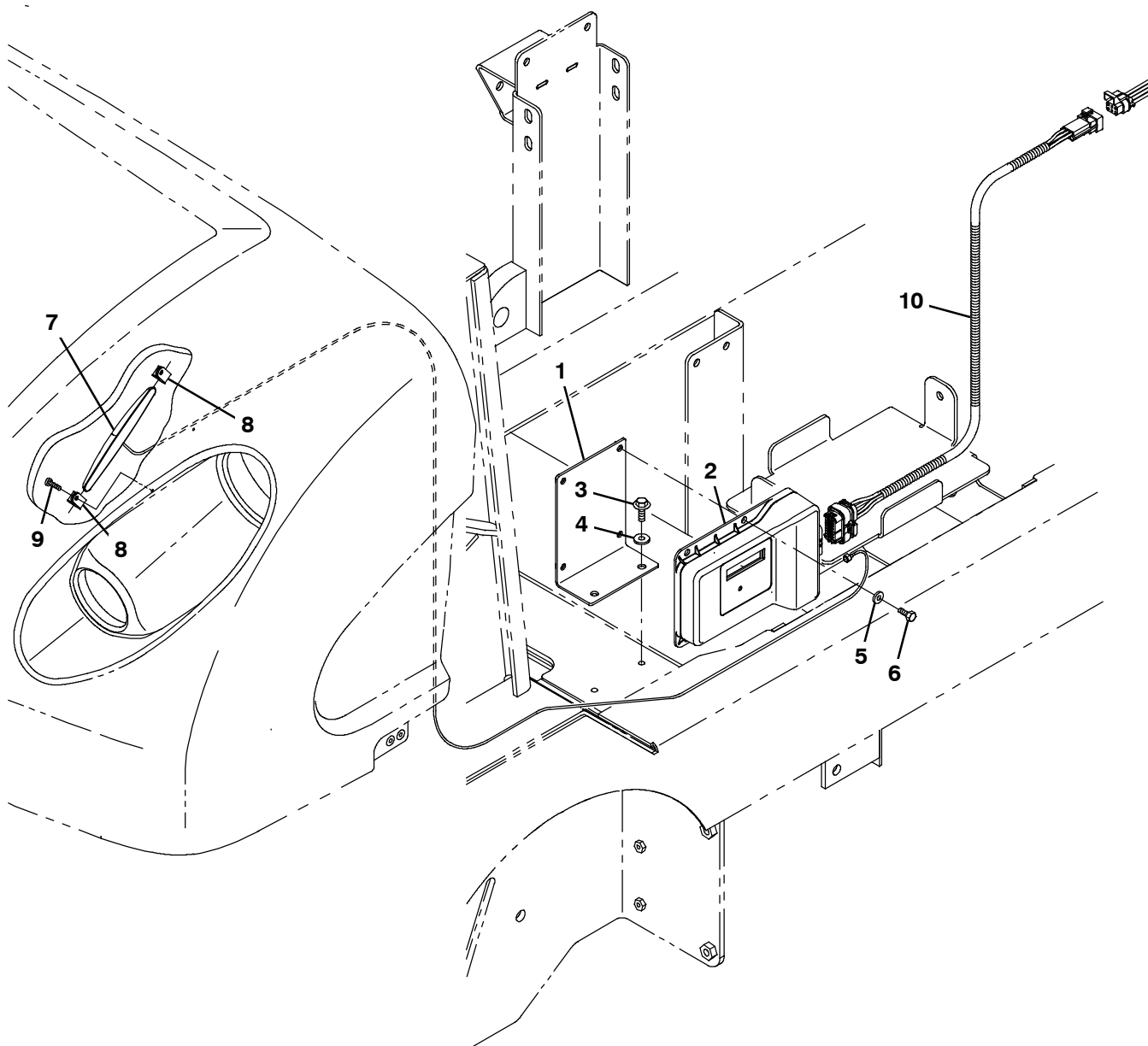
Fig. 22 - Telemetry Group
