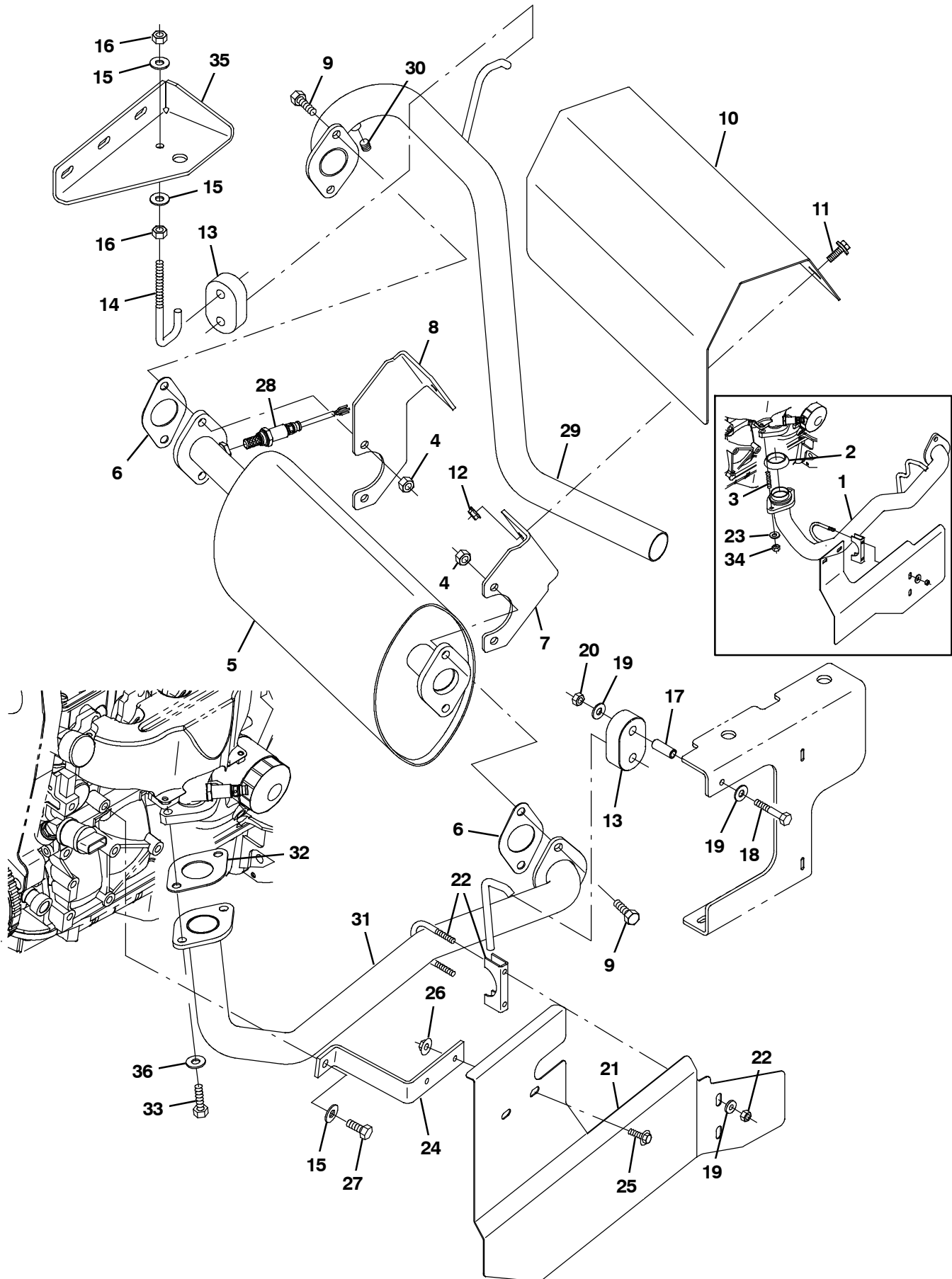
Fig. 35 - Engine Muffler Group (000000-005699)
