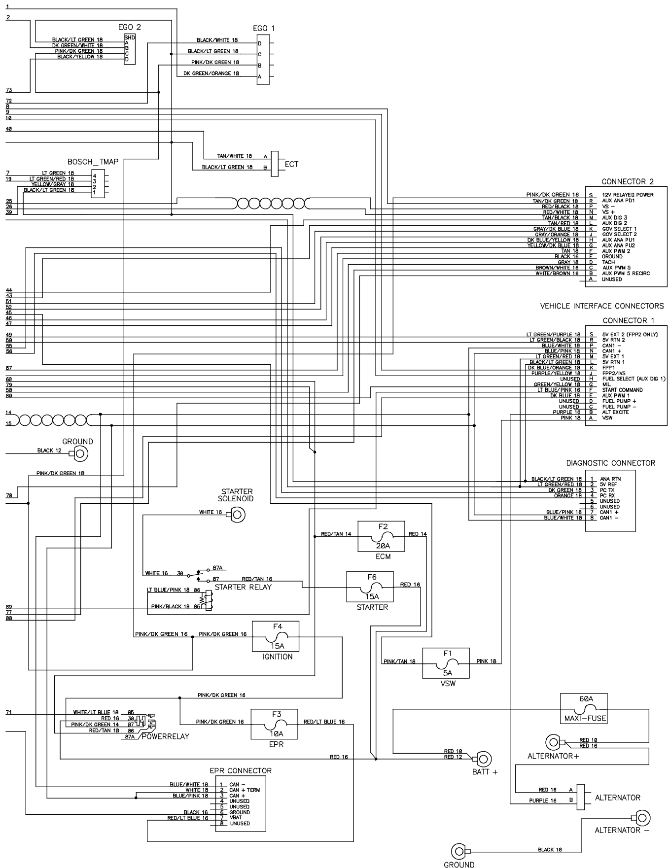
Fig. 86 - Electrical Schematic, LPG Engine Harness, GM (000000-005699) (2 of 2)
