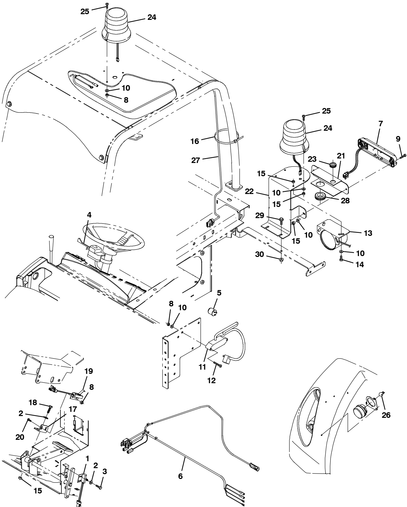
Fig. 4 - Outdoor Light Kit (002100- )
