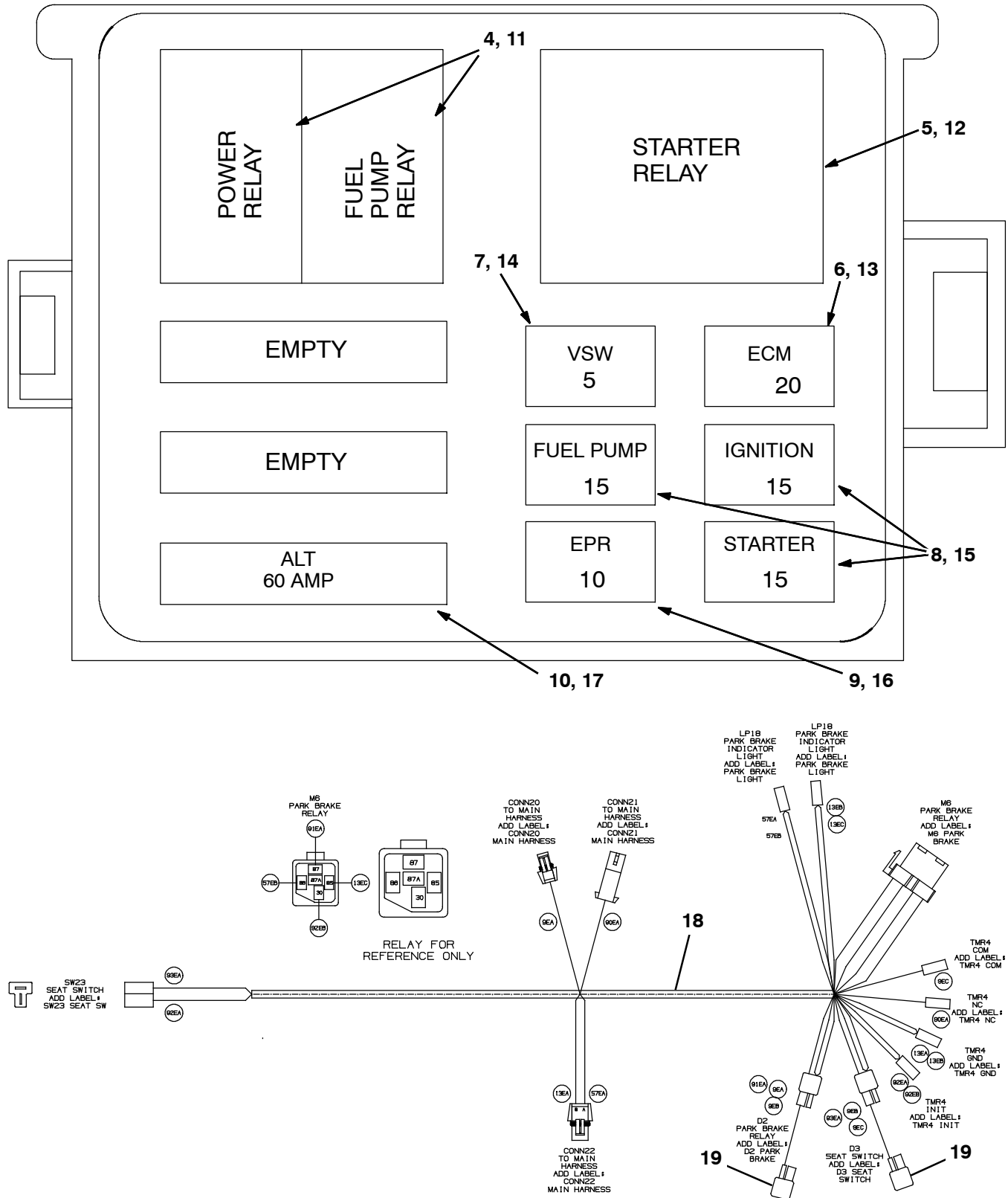
Fig. 88 - Electrical Wire Harnesses Group
