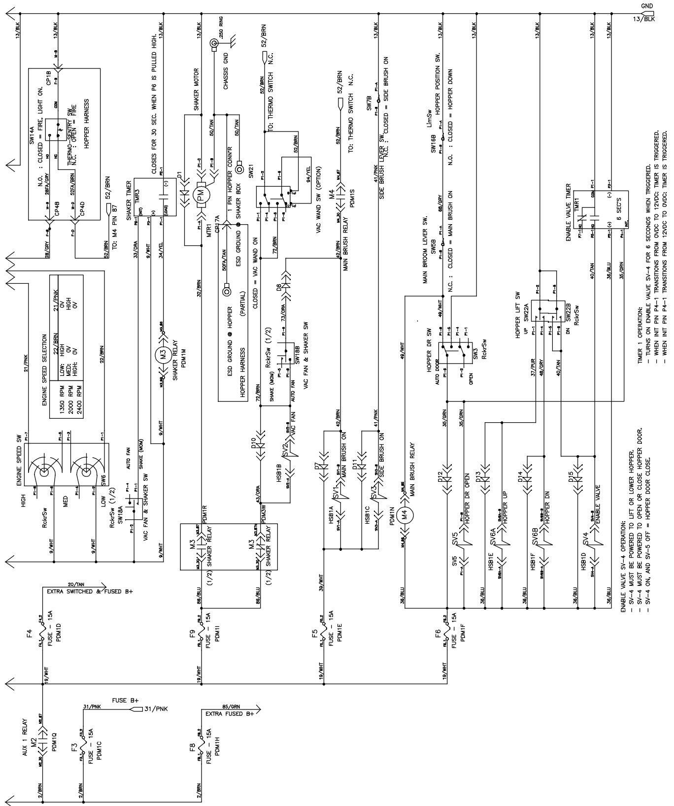
Fig. 80 - Electrical Schematic, GM, S30 (000000-005699) (2 of 4)
