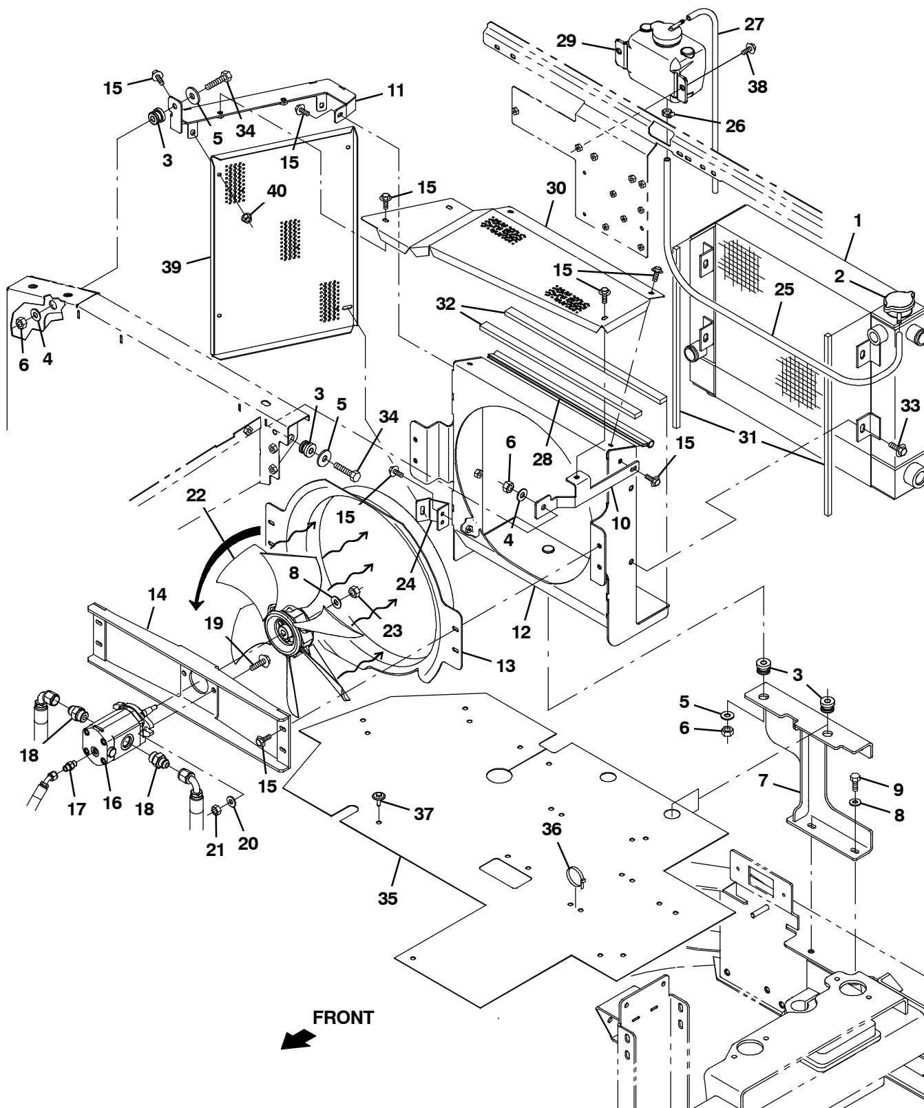
Fig. 40 - Engine Radiator Mount and Fan Group (002100- )
