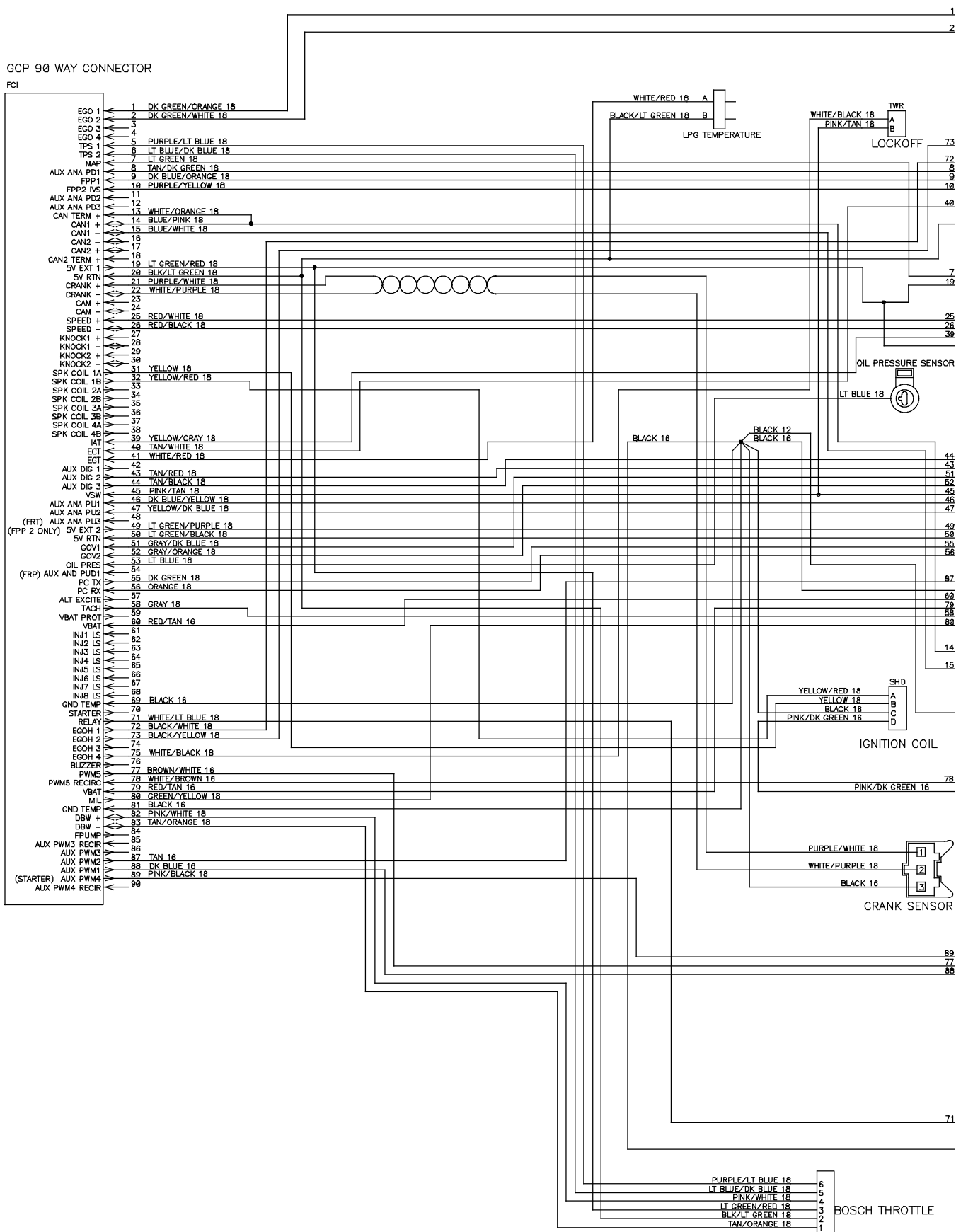
Fig. 86 - Electrical Schematic, LPG Engine Harness GM (000000-005699) (1 of 2)
