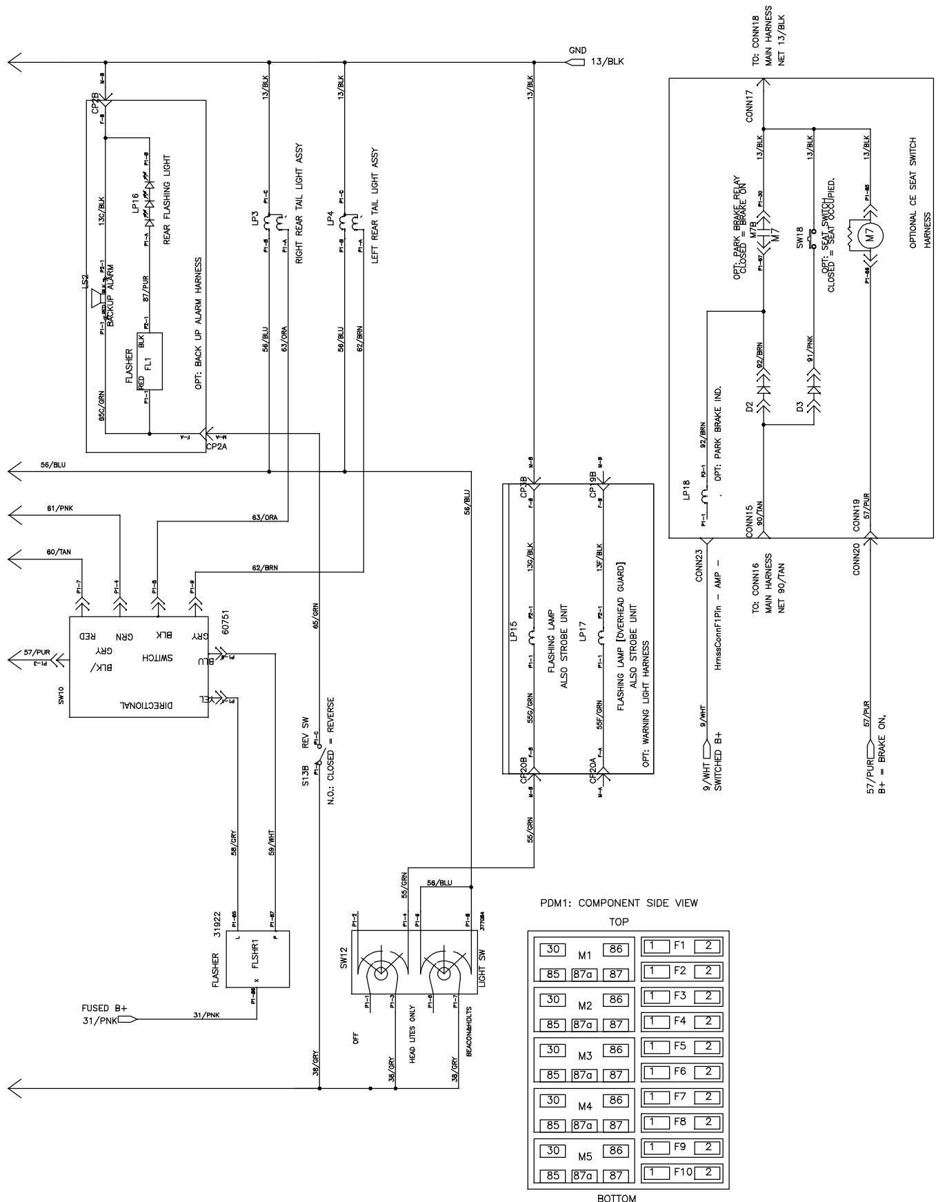
Fig. 82 - Electrical Schematic, GM, S30 XP (000000-005699) (4 of 4)
