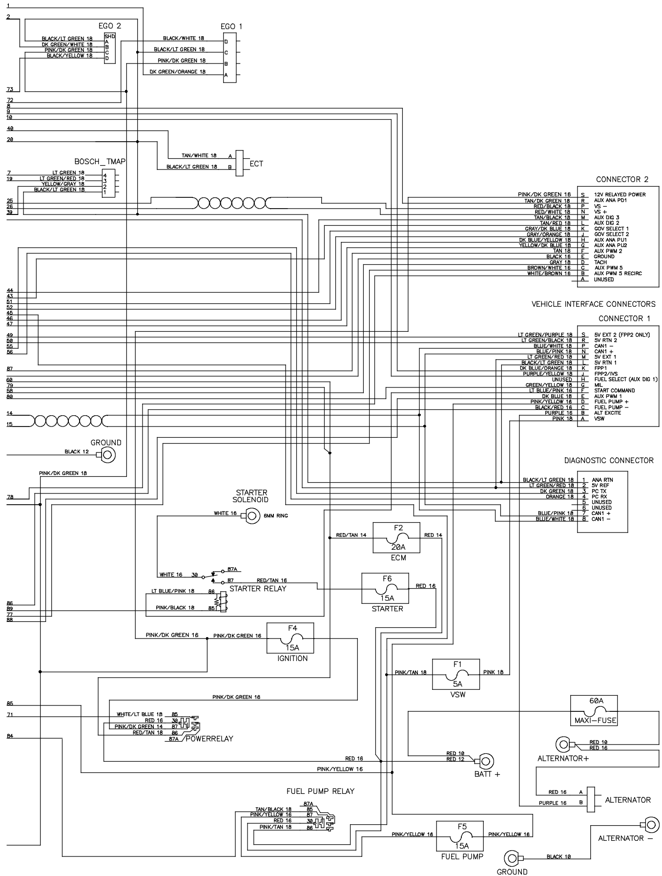
Fig. 84 - Electrical Schematic, Gasoline Engine Harness, GM (000000-005699) (2 of 2)
