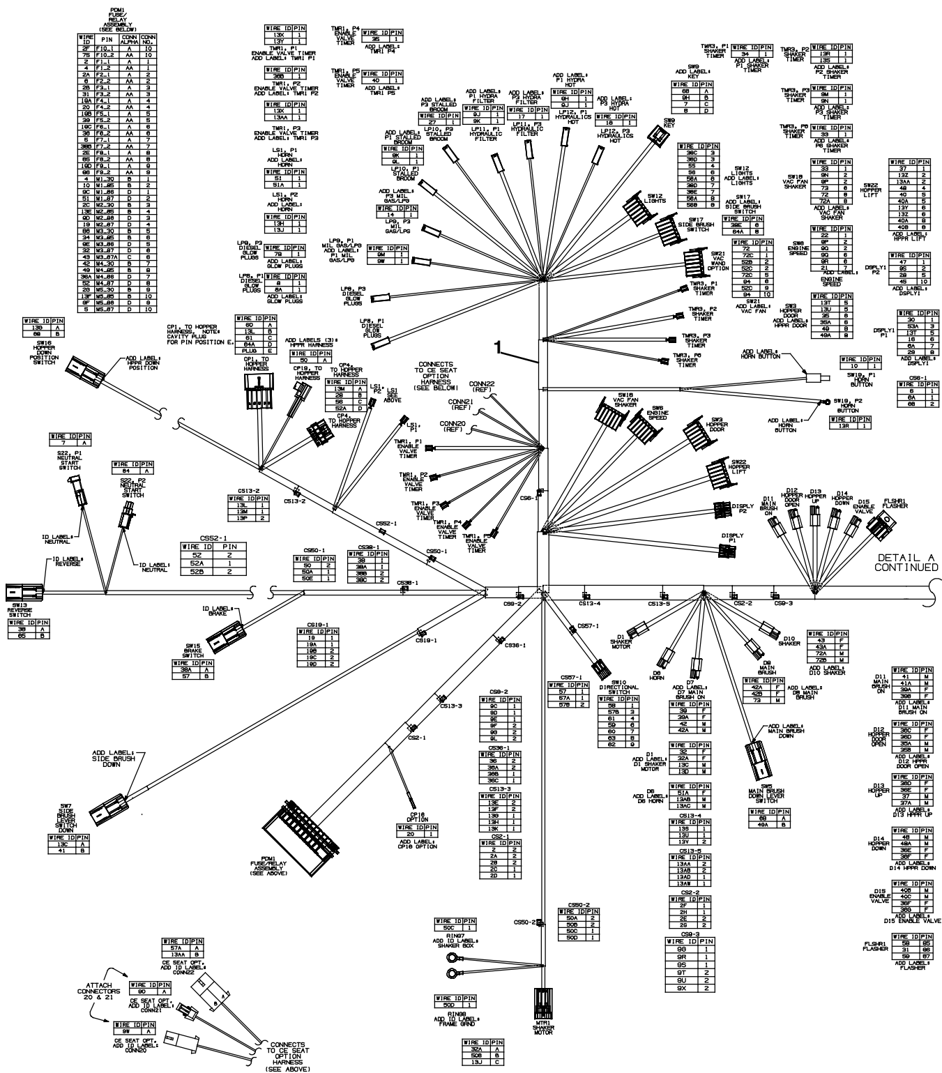
Fig. 88 - Electrical Wire Harnesses Group
