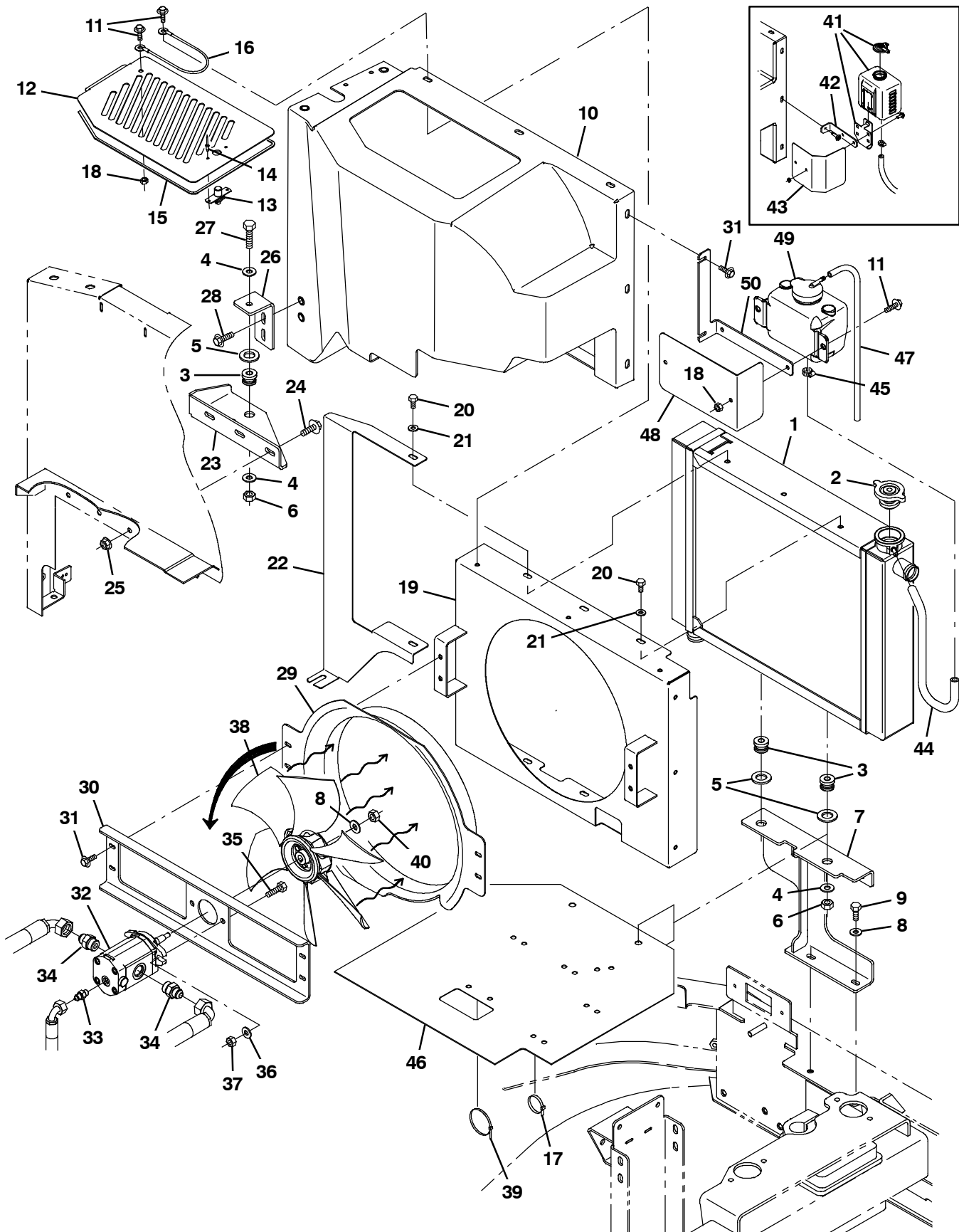
Fig. 39 - Engine Radiator Mount and Fan Group (000000-002099)
