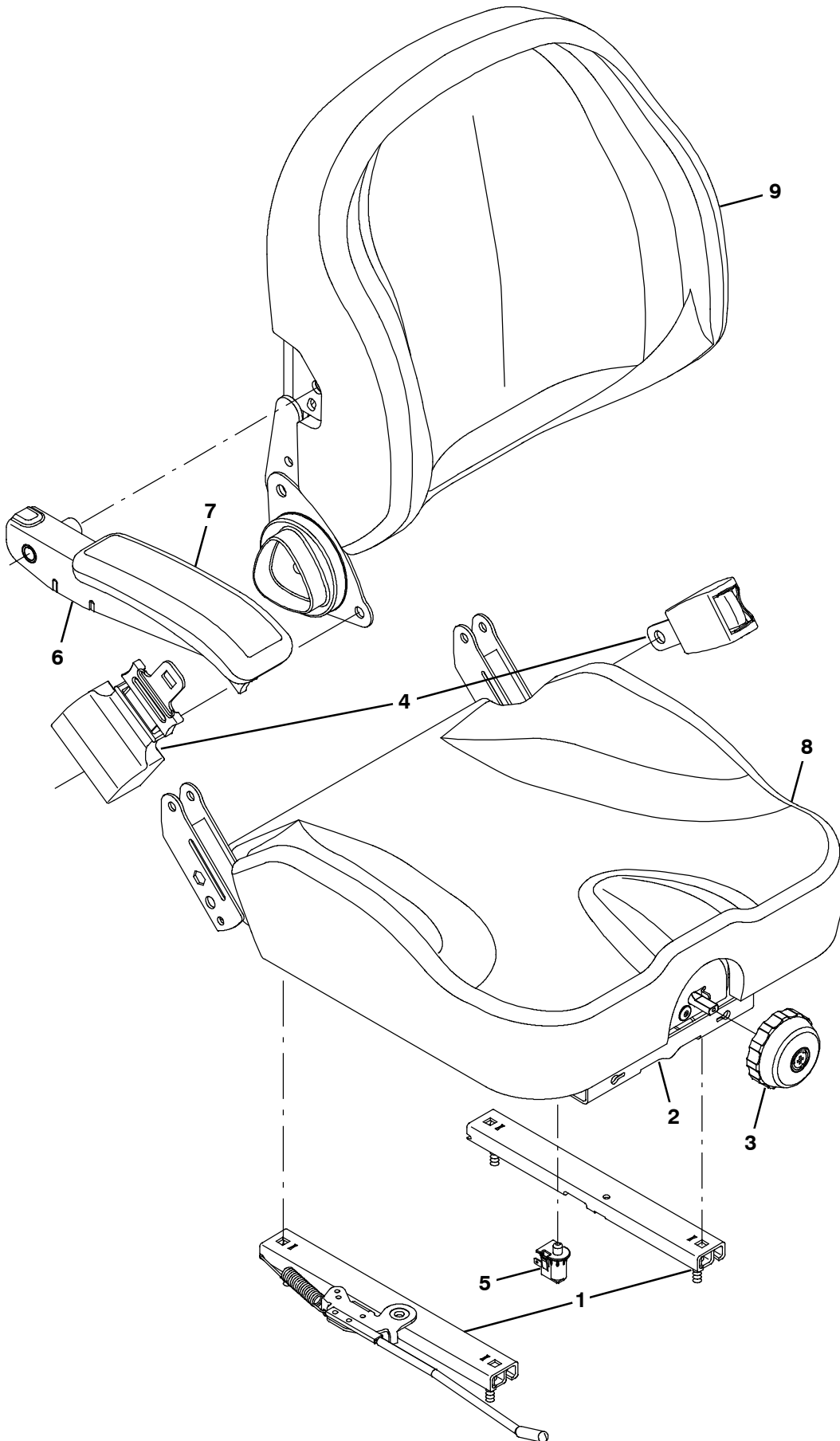
Fig. 7 - Seat Breakdown, 1073641
