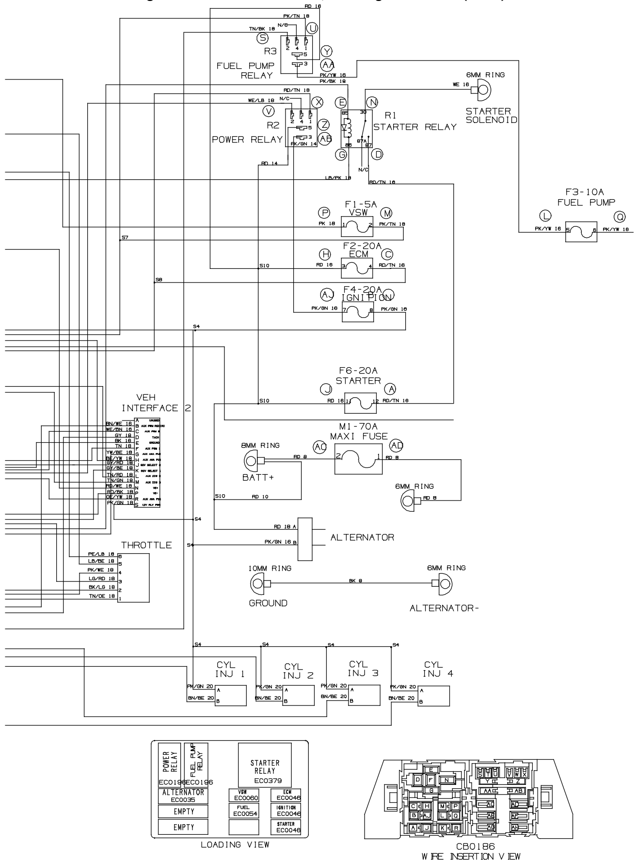
Fig. 60 - Electrical Schematic, Gas Engine Harness (2 of 2)
