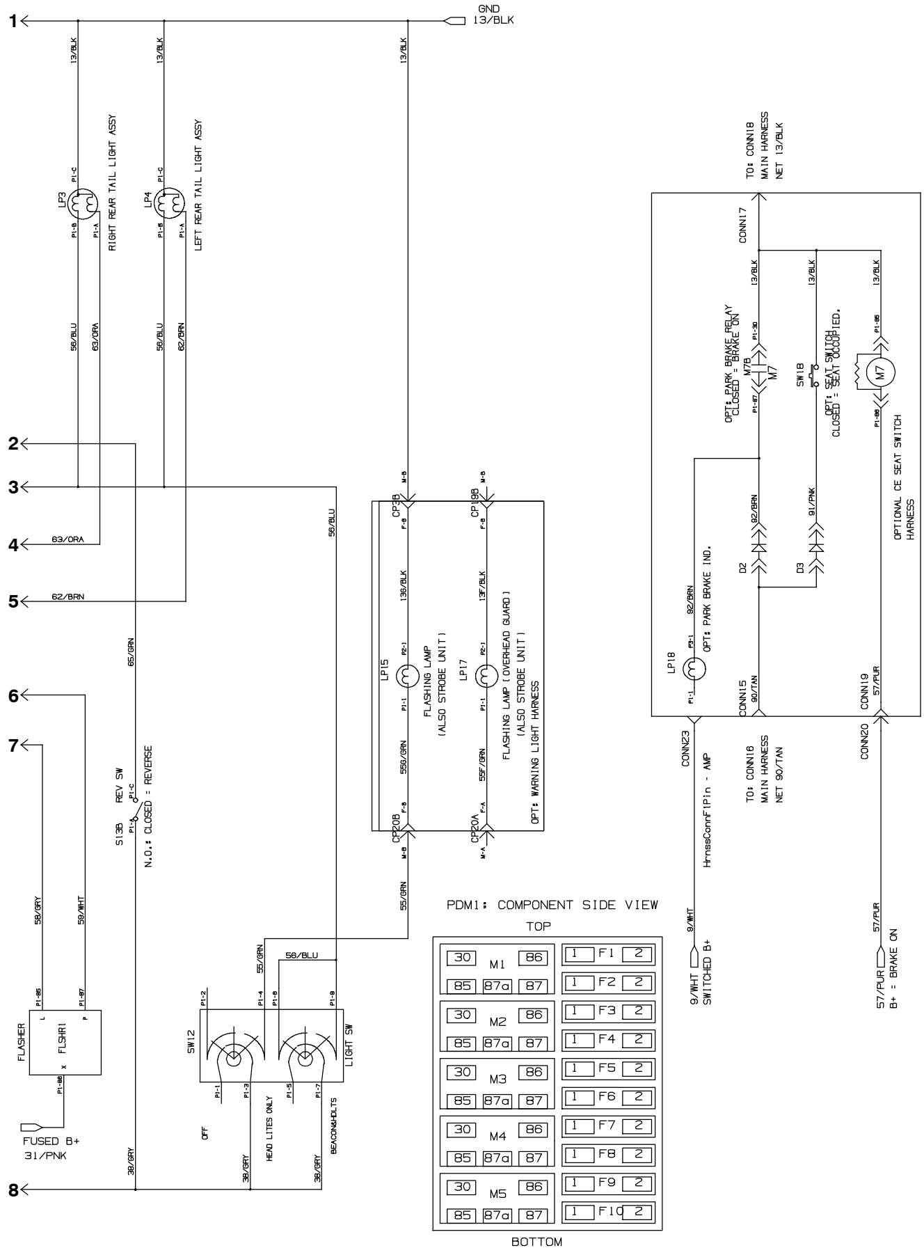
Fig. 59 - Electrical Schematic, S30 XP
