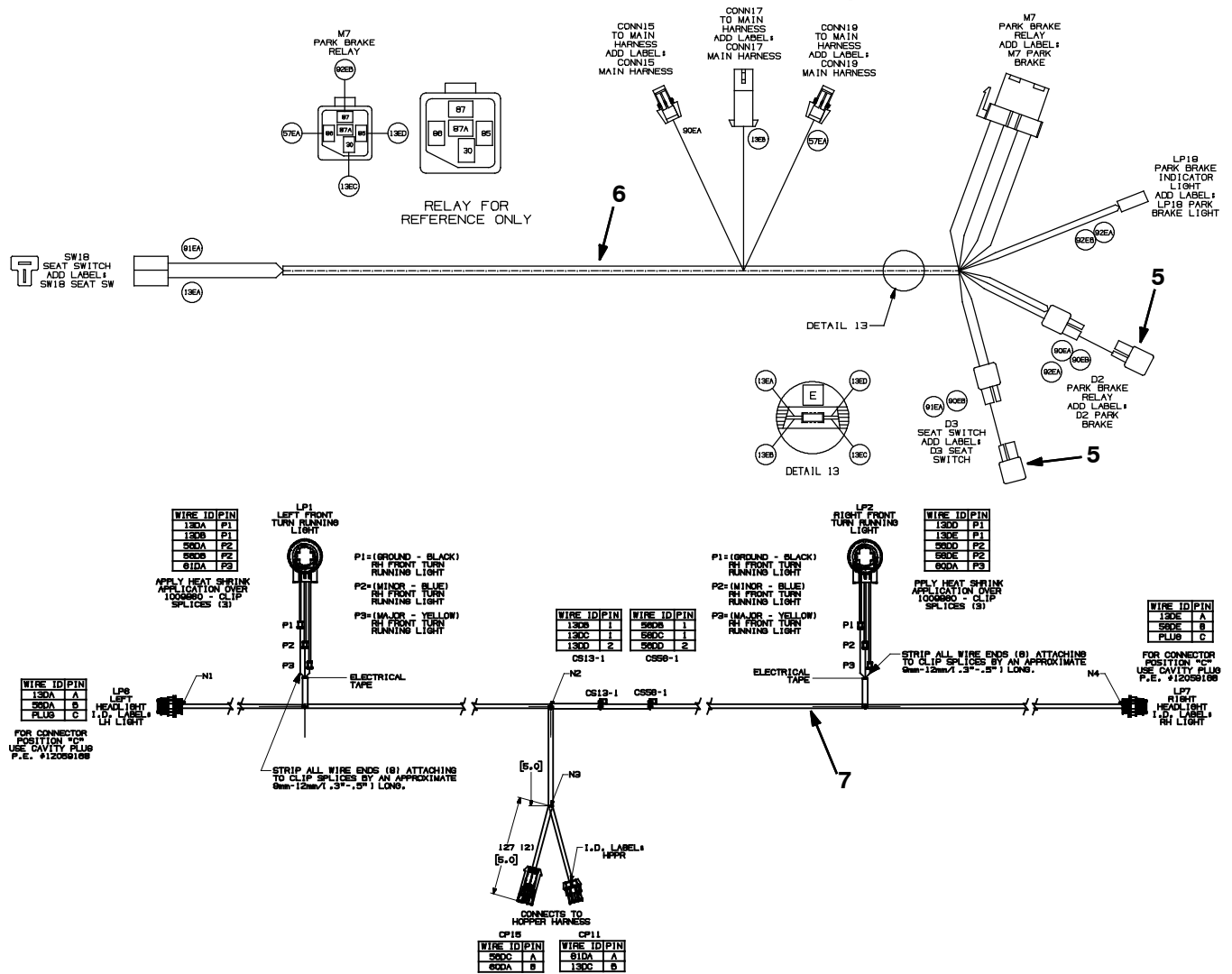
Fig. 62 - Electrical Wire Harnesses Group
