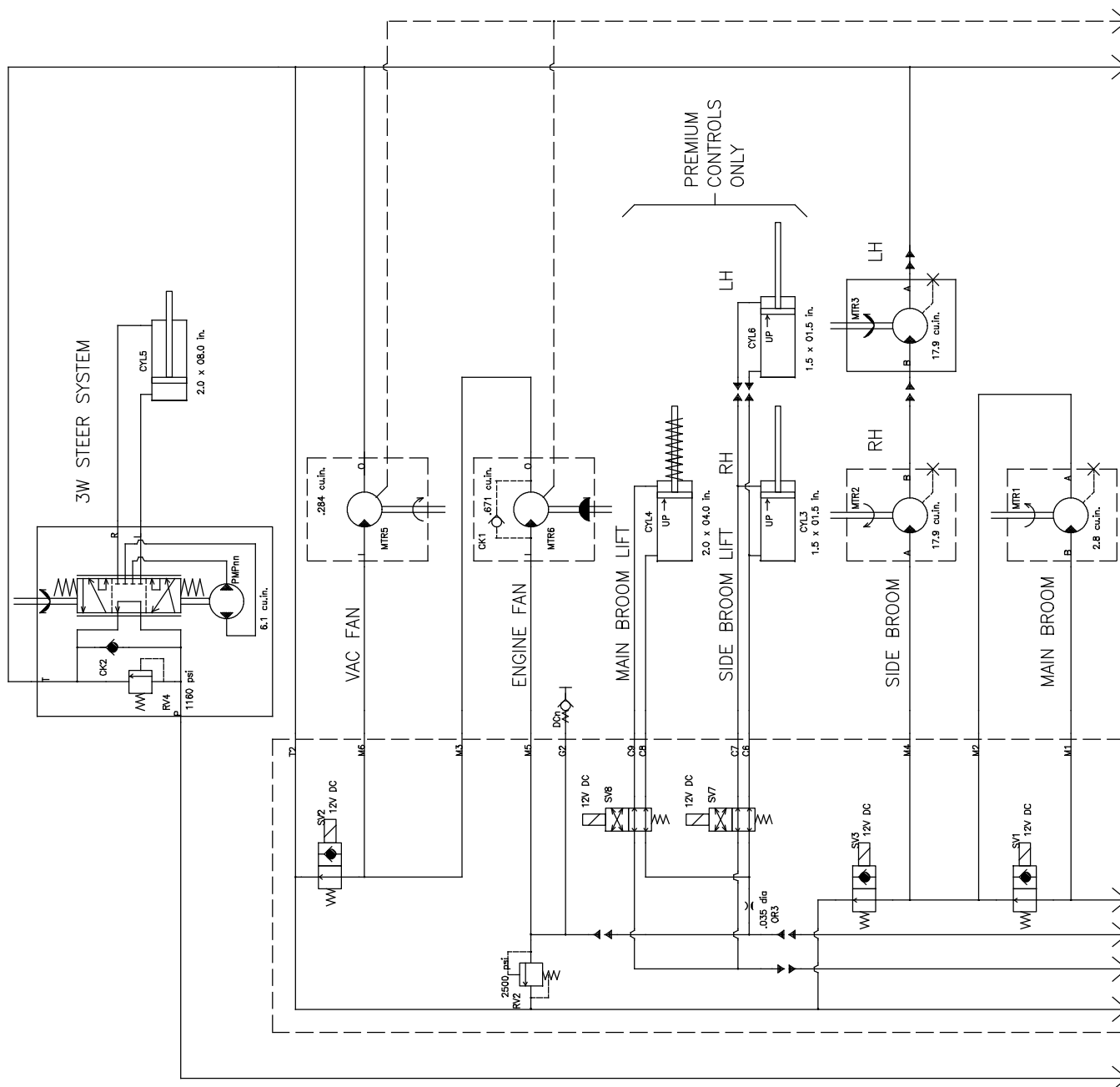
Fig. 50 - Hydraulic Schematic
