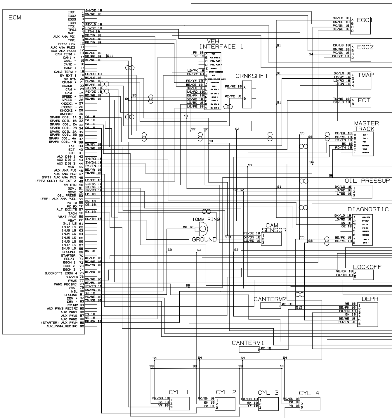
Fig. 61 - Electrical Schematic, LPG Engine Harness (1 of 2)
