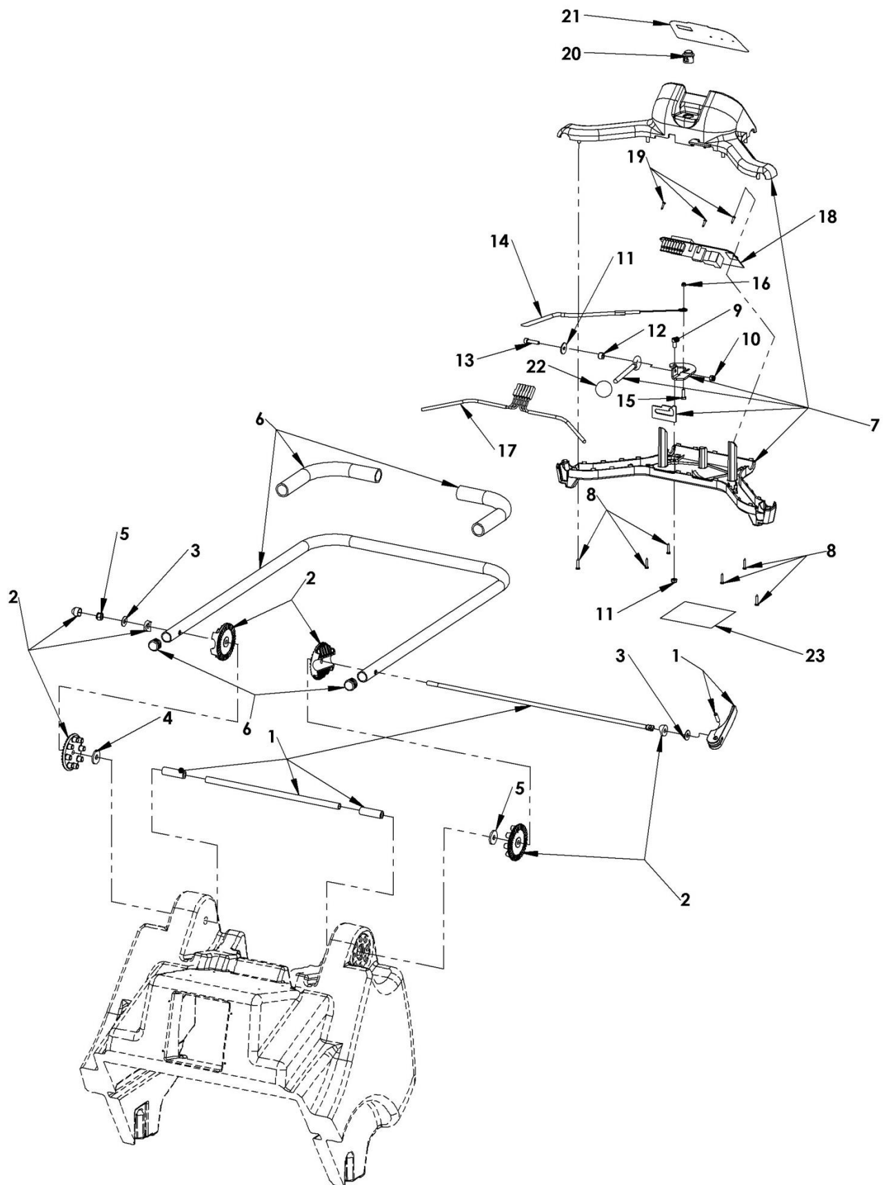
Fig. 4 – Handle Assy
