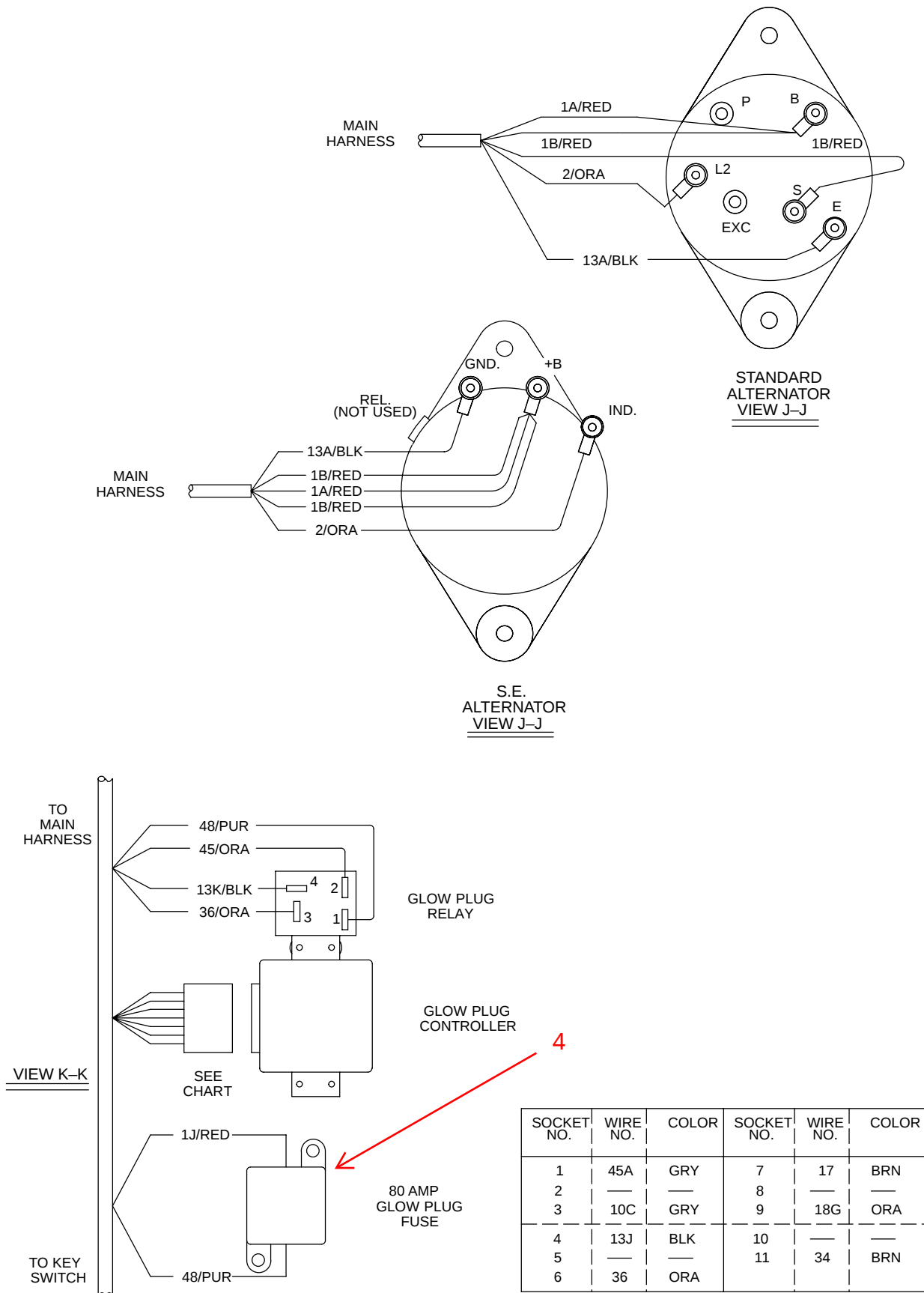
Fig. 71 – Wire Harness Group
