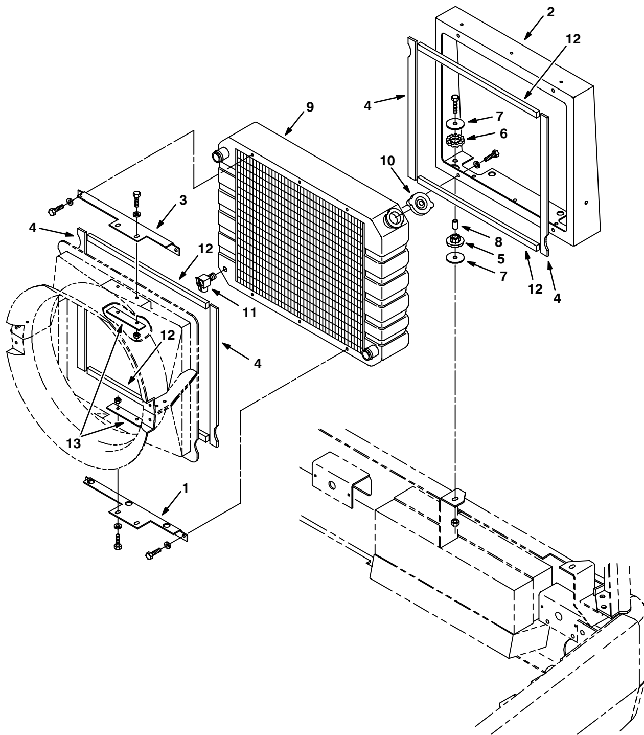
Fig. 38 – Radiator Group
