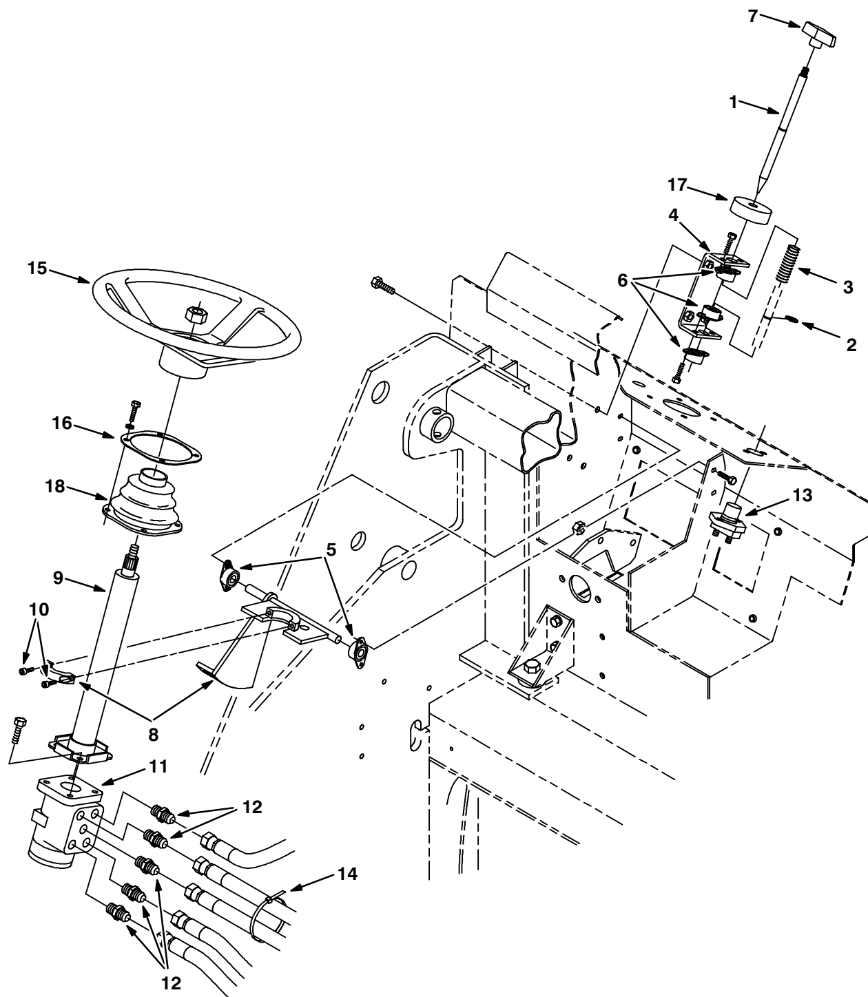
Fig. 67 – Steering Group
