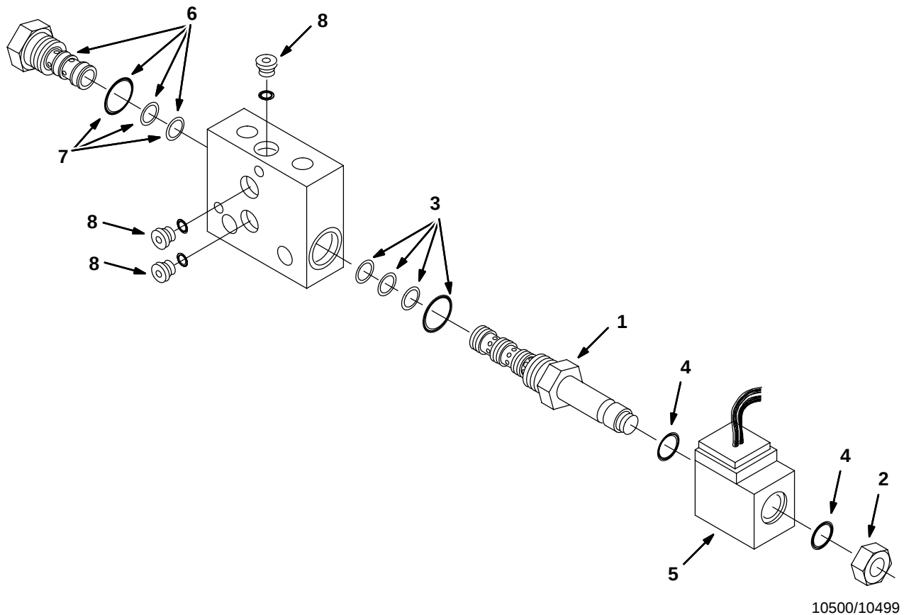
Fig. 20 – Hydraulic Solenoid Valve Breakdown, 84016
