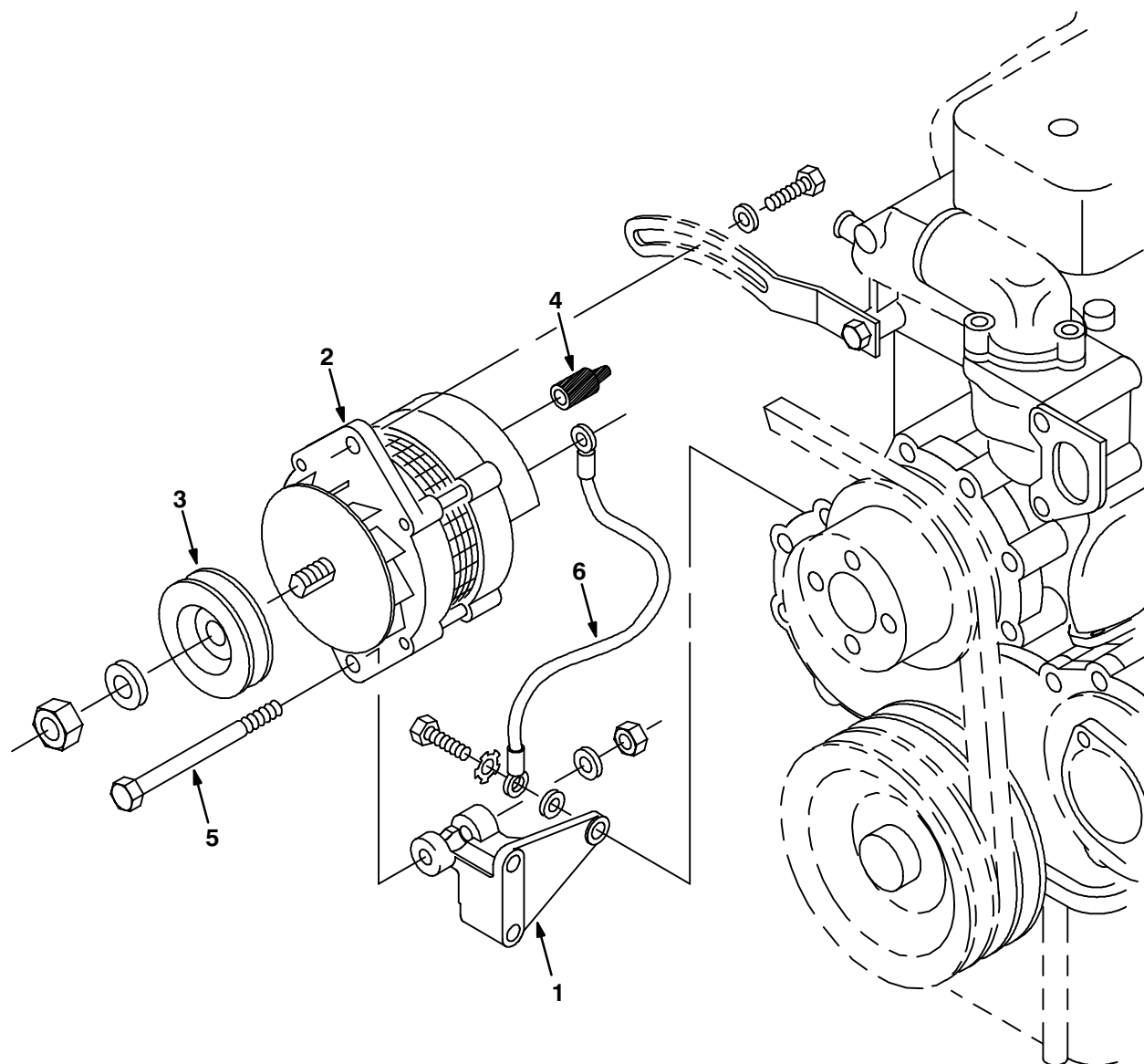
Fig. 30 – Alternator Group
