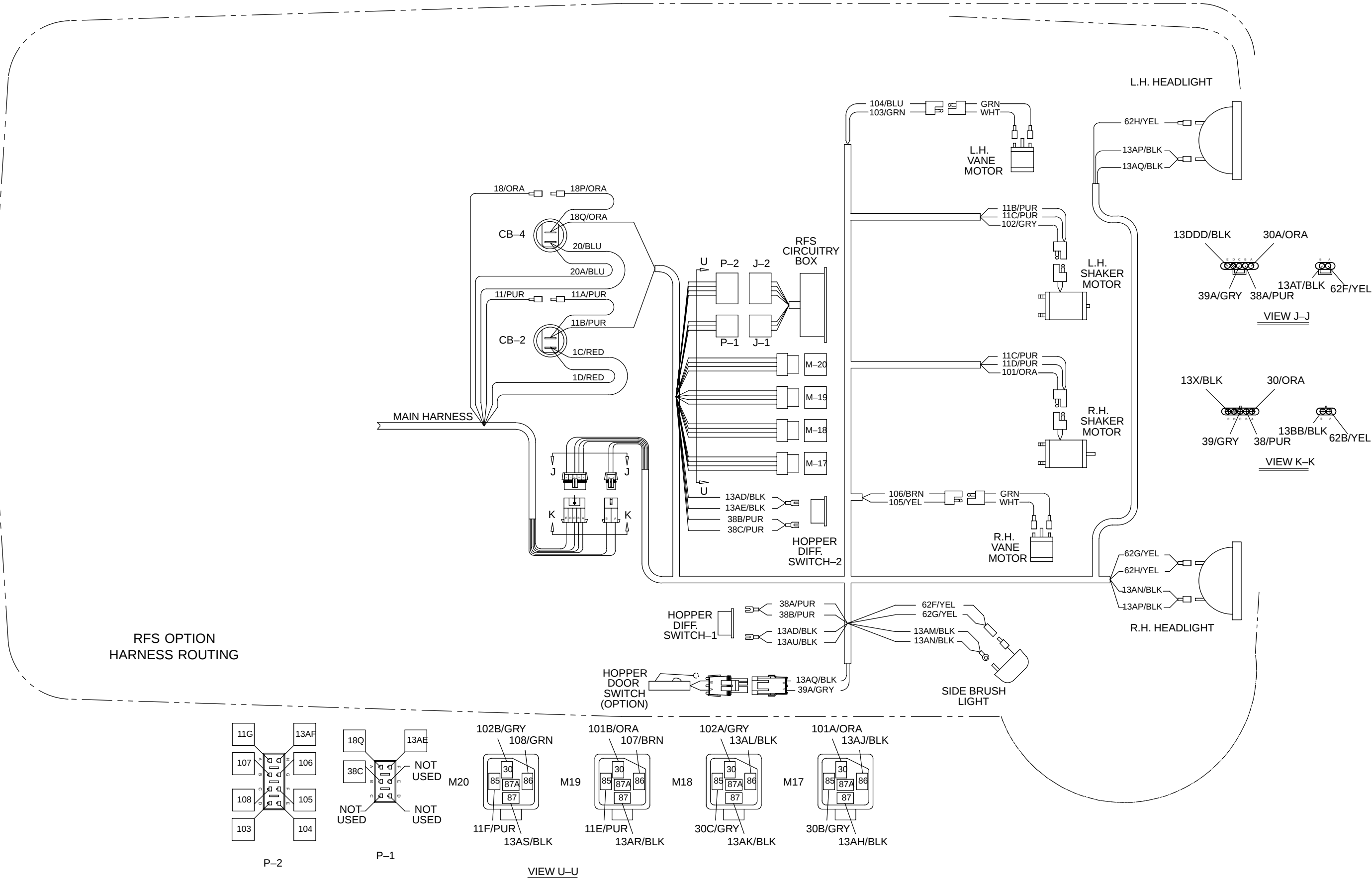
Fig. 71 – Wire Harnesses Group
