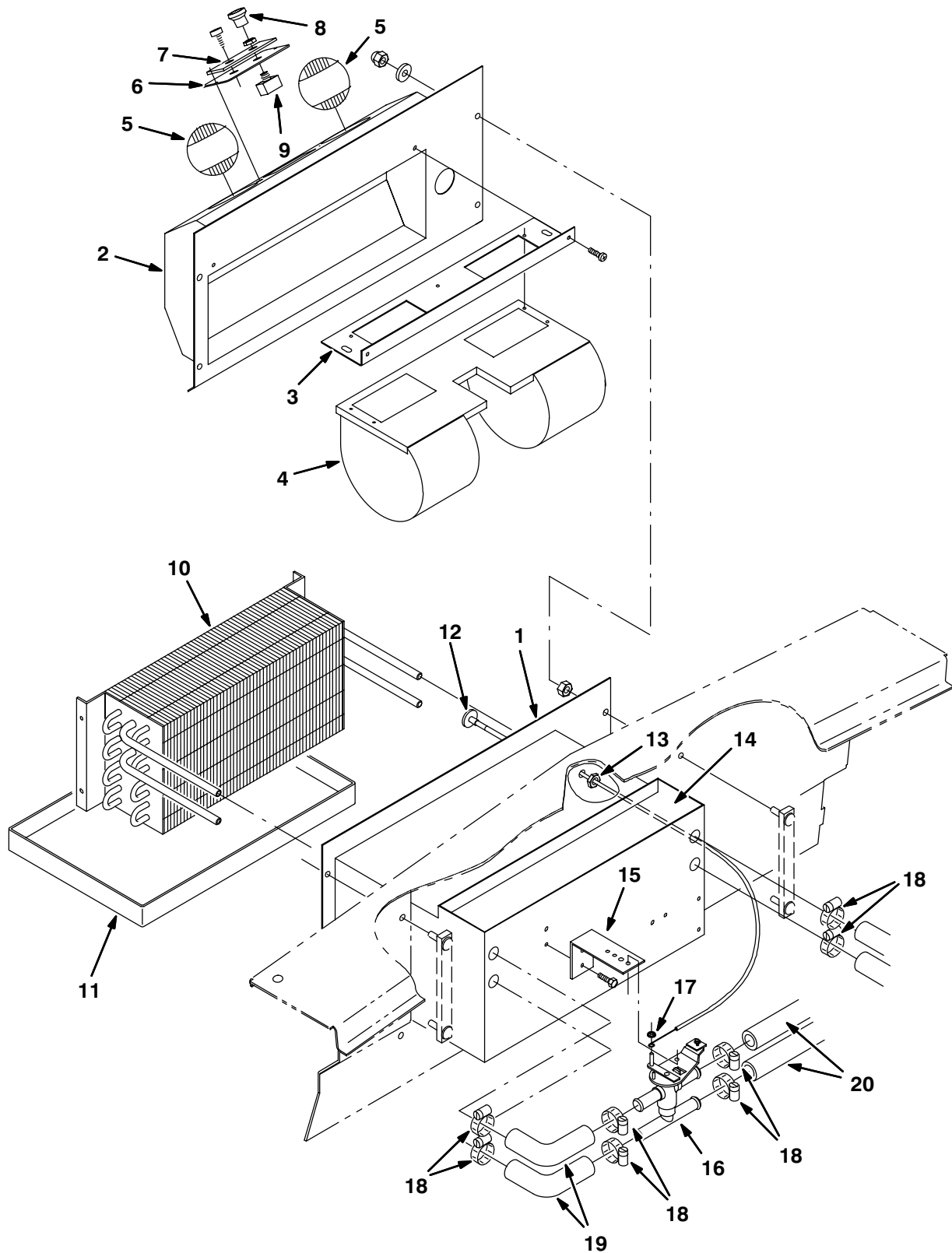
Fig. 32 – Heater/Pressurizer Breakdown, 74091
