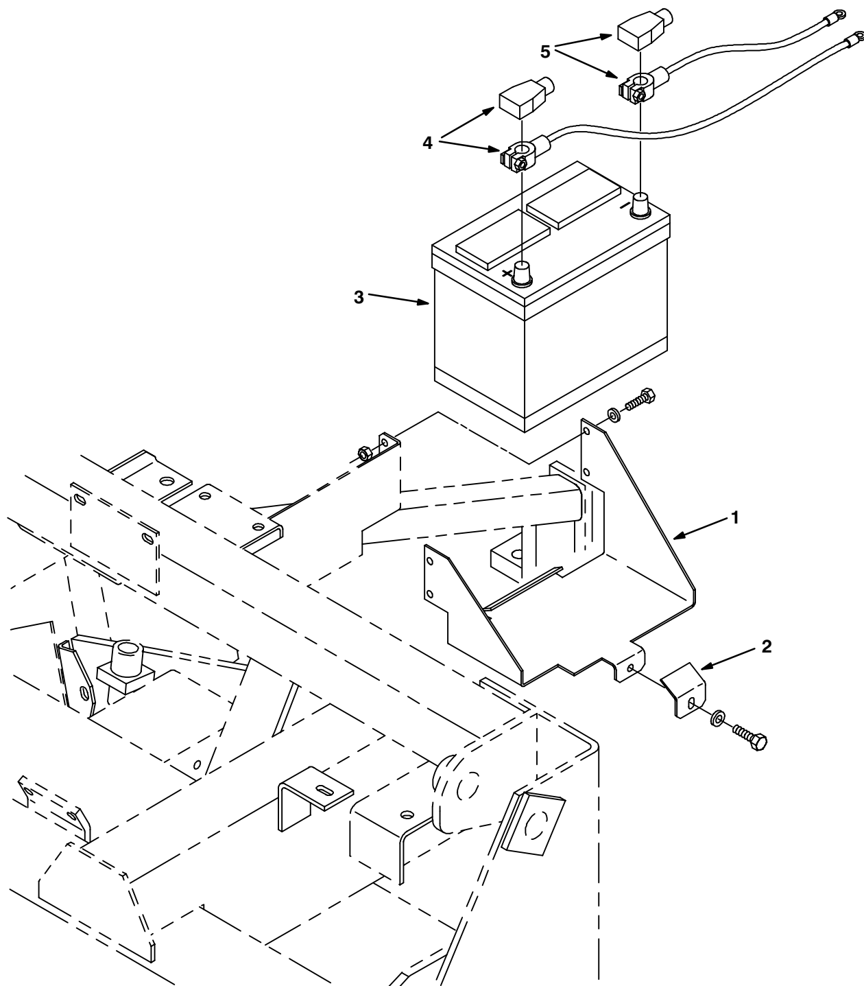
Fig. 42 – Battery Group
