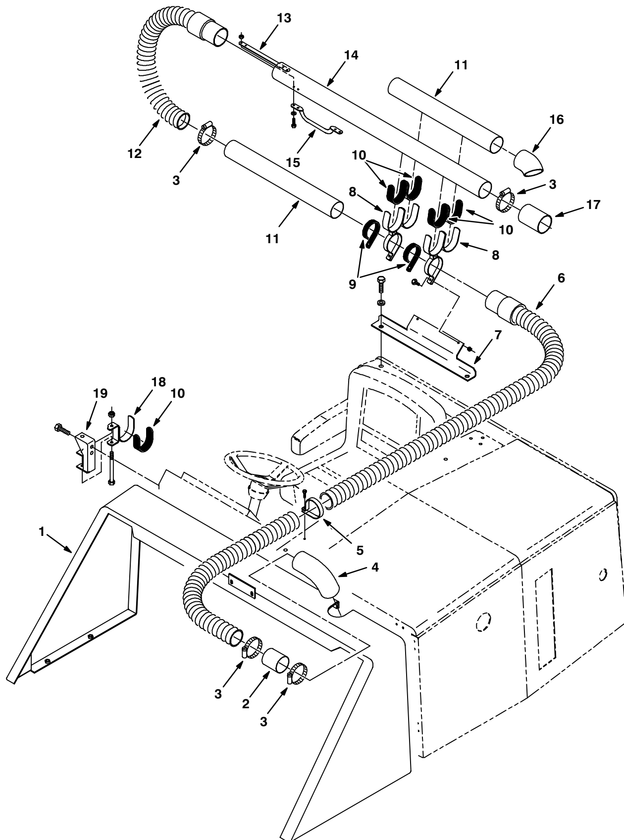
Fig. 12 – Blower Group
