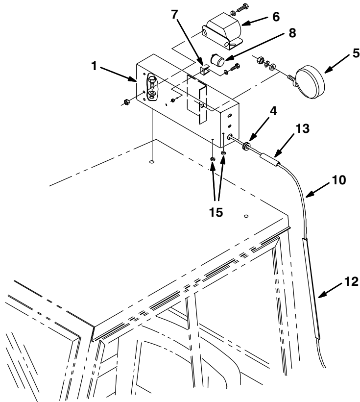
Fig. 7 – Back-Up Alarm Warning Kit
