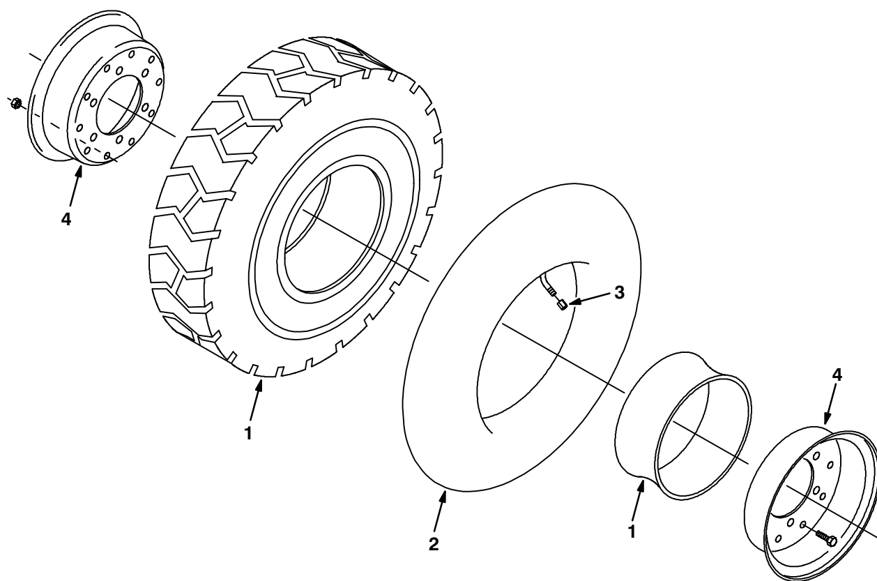
Fig. 45 – Wheel Assembly
