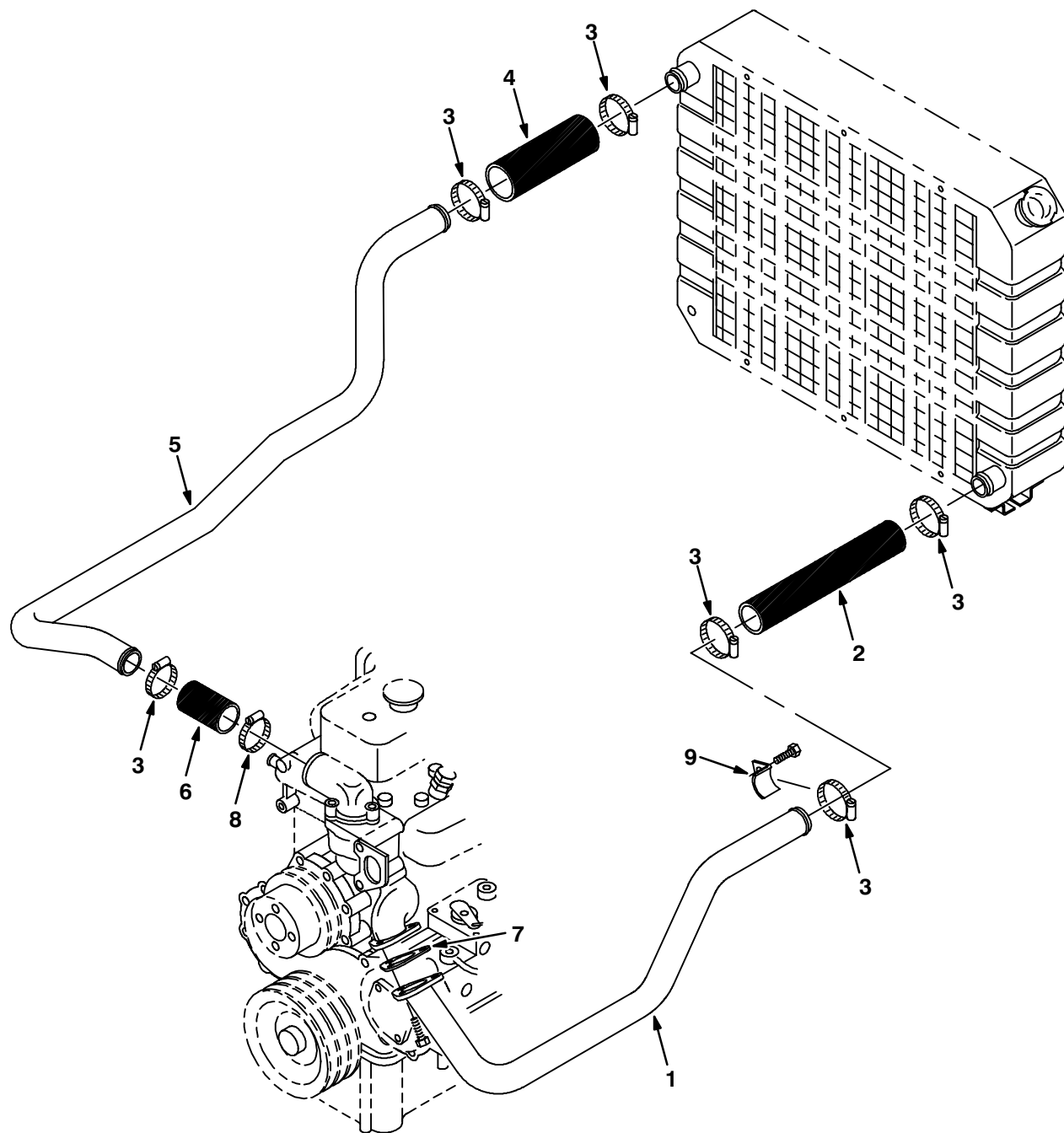
Fig. 36 – Radiator Hose Group
