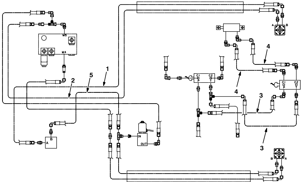
Fig. 24 – Side Brush Hydraulic Hose Group, L.H.
