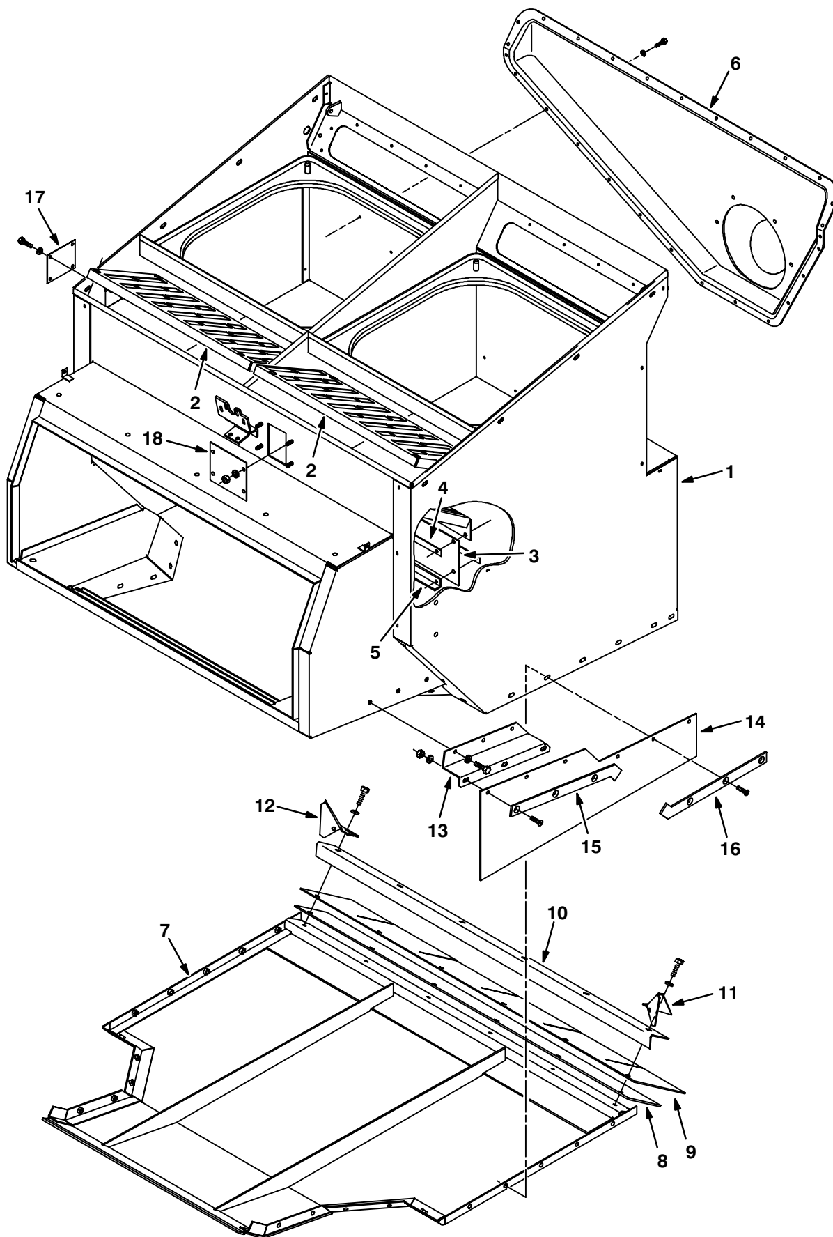
Fig. 18 – Hopper Group
