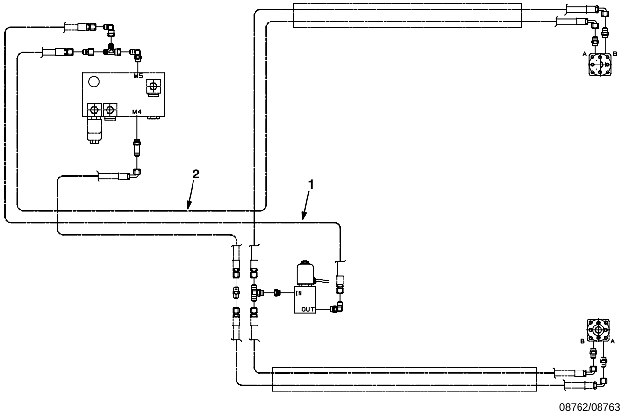
Fig. 23 – Side Brush Hydraulic Hose Group, L.H.
