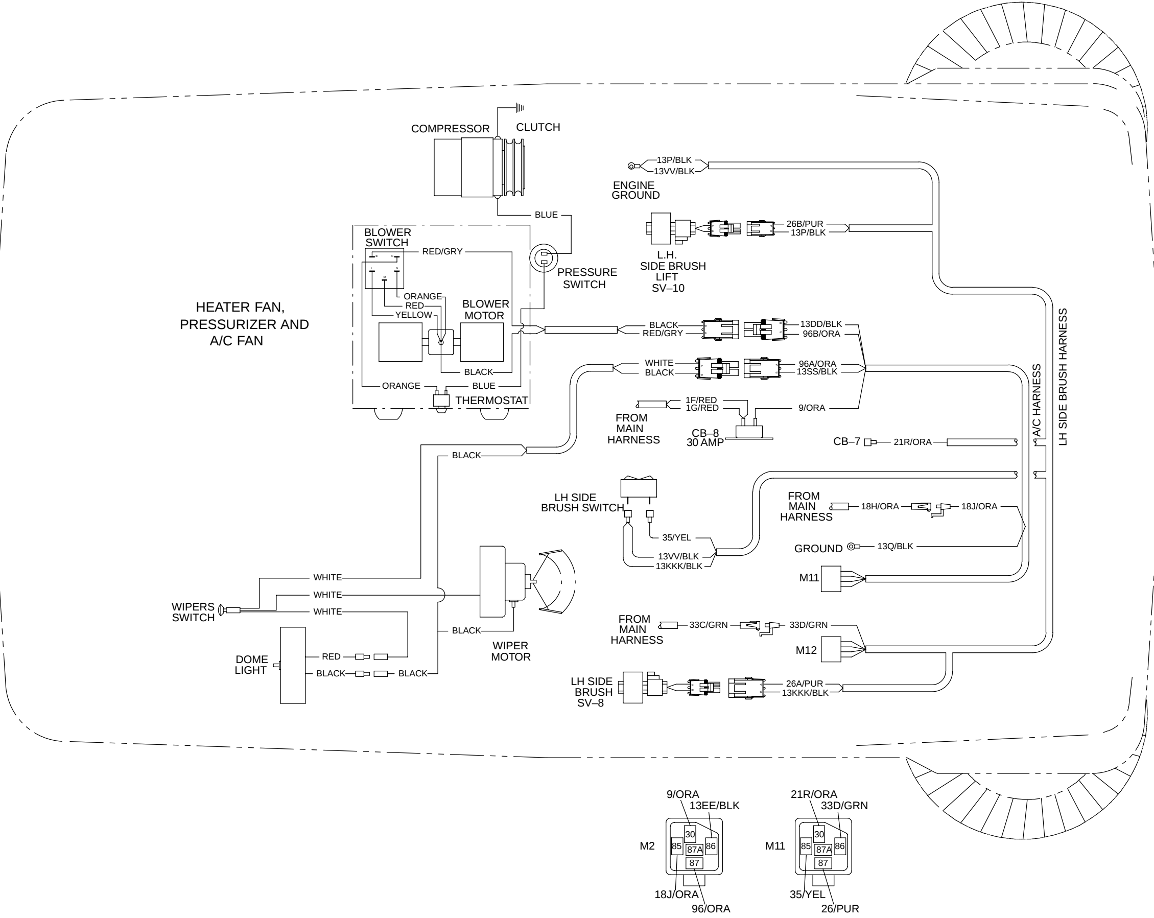
Fig. 71 – Wire Harnesses Group
