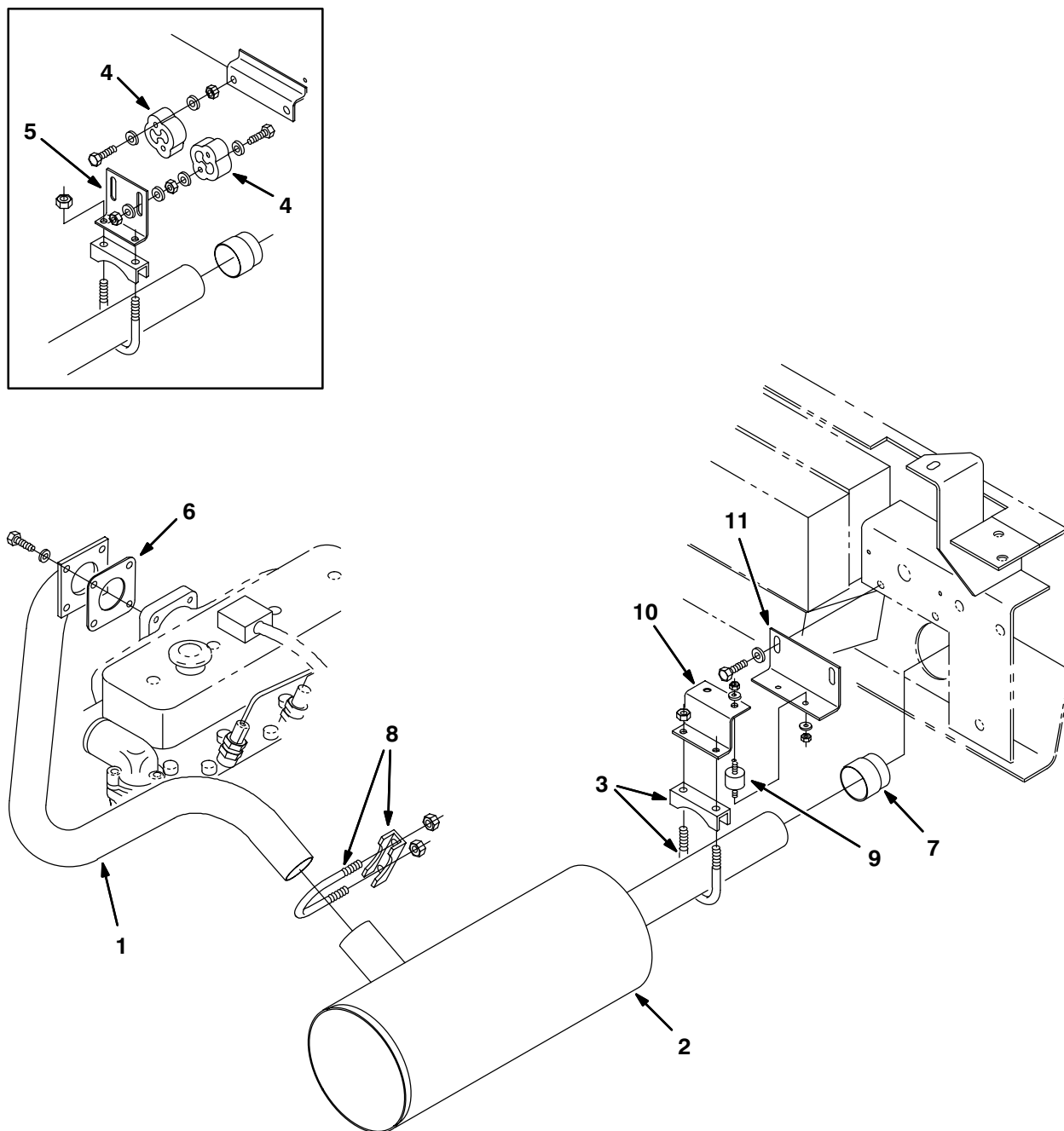
Fig. 33 – Muffler Group
