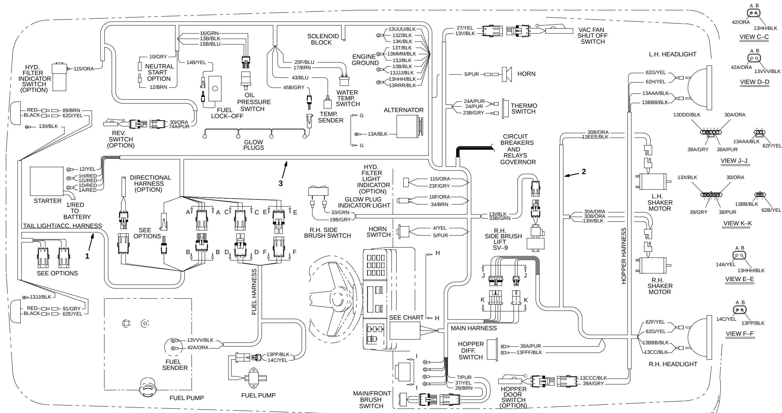
Fig. 71 – Wire Harnesses Group
