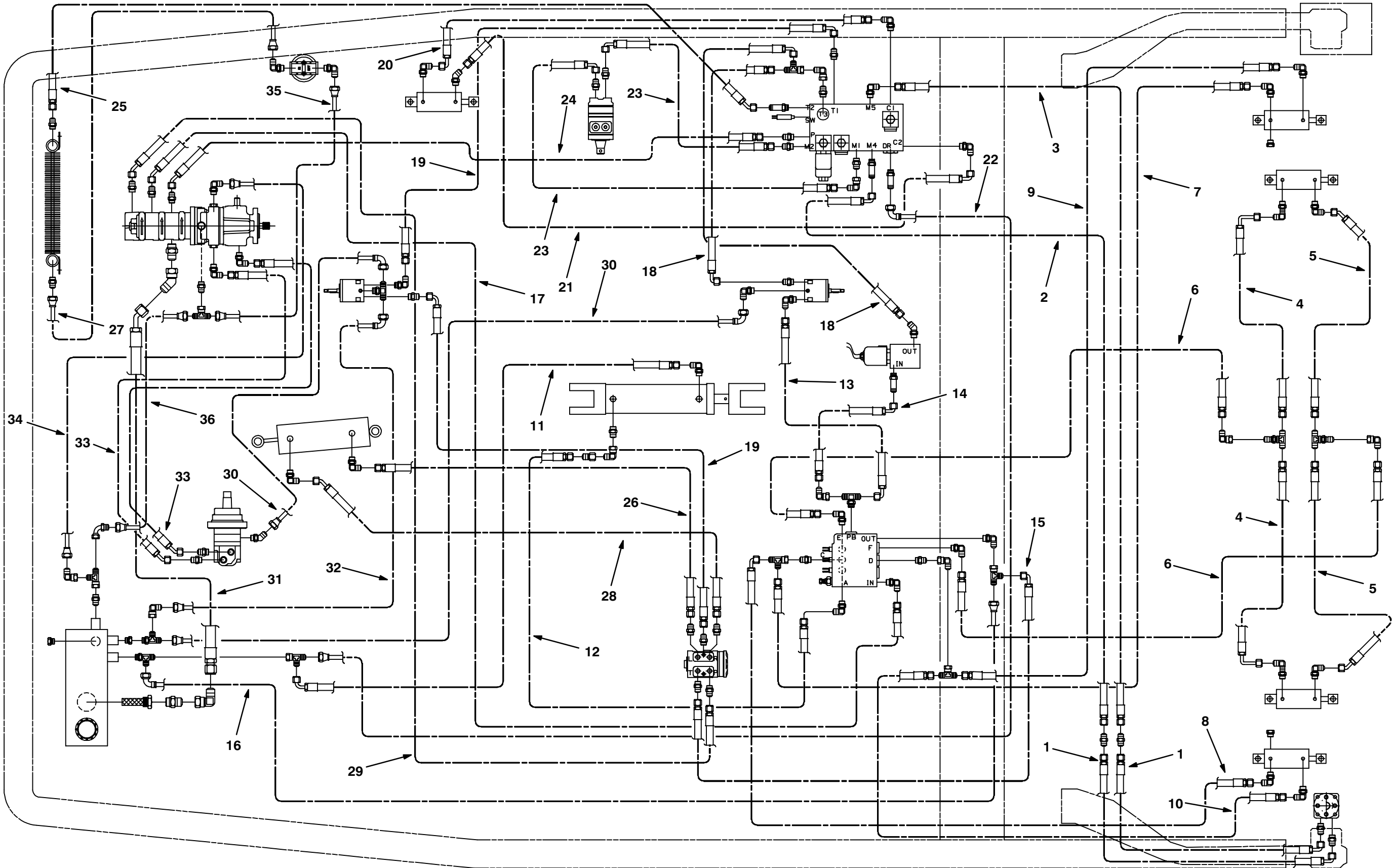
Fig. 51 – Hydraulic Hose Group (for machines below serial number xxxxxx)
