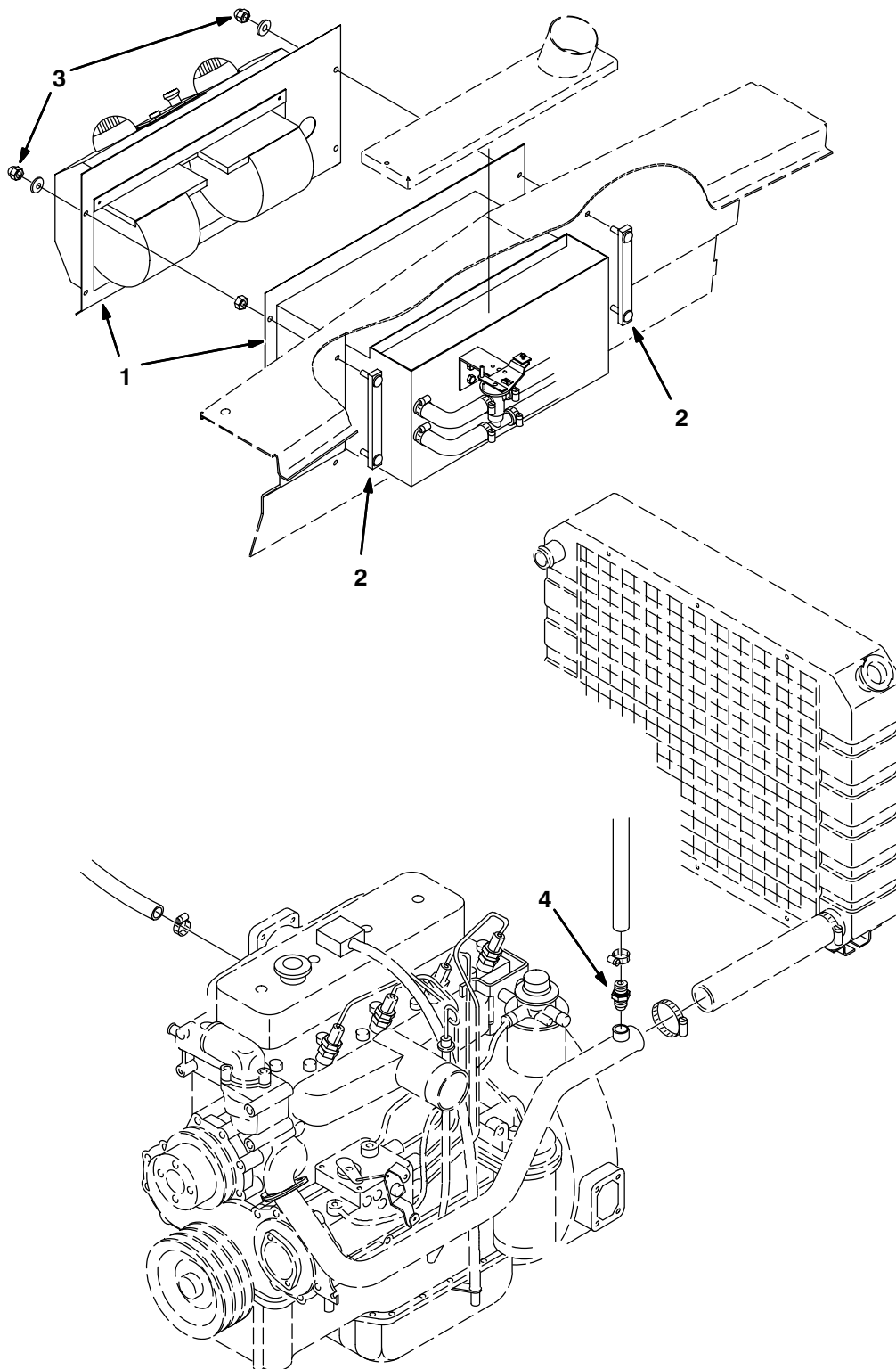
Fig. 32 – Heater/Pressurizer Assembly
