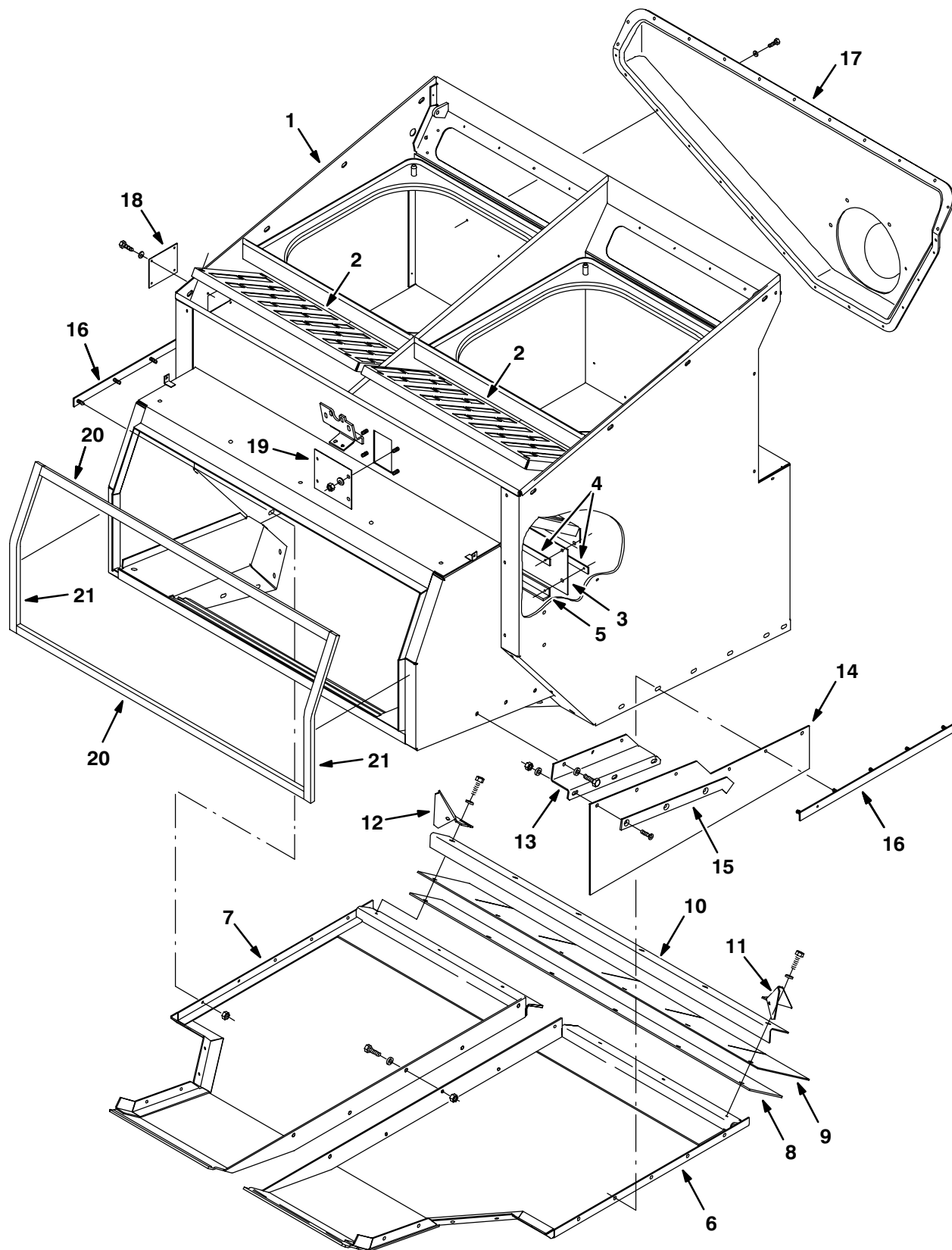
Fig. 19 – Hopper Group
