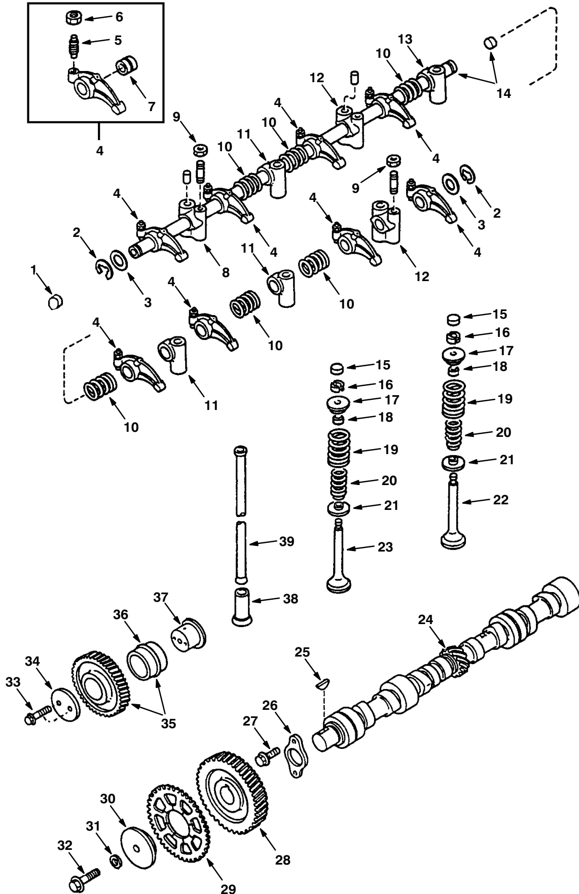
Fig. 5 – Valve Group
