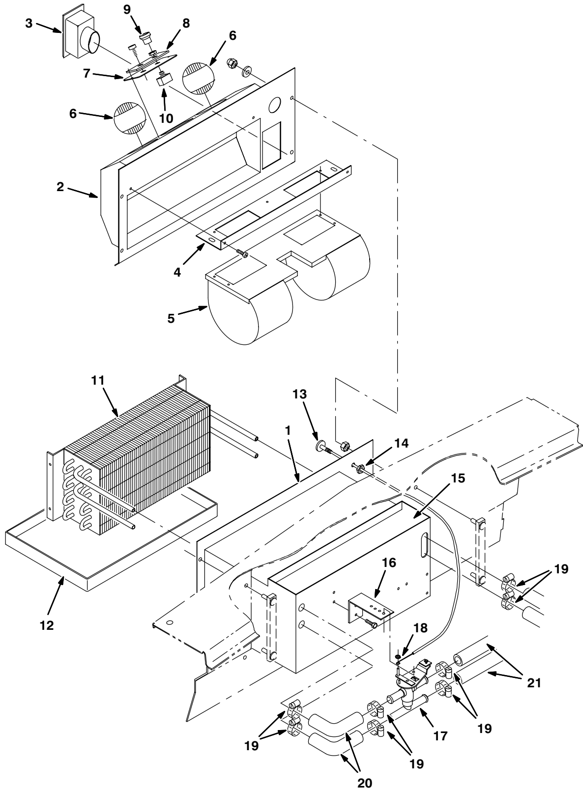
Fig. 33 – Heater/Pressurizer Breakdown, 21271
