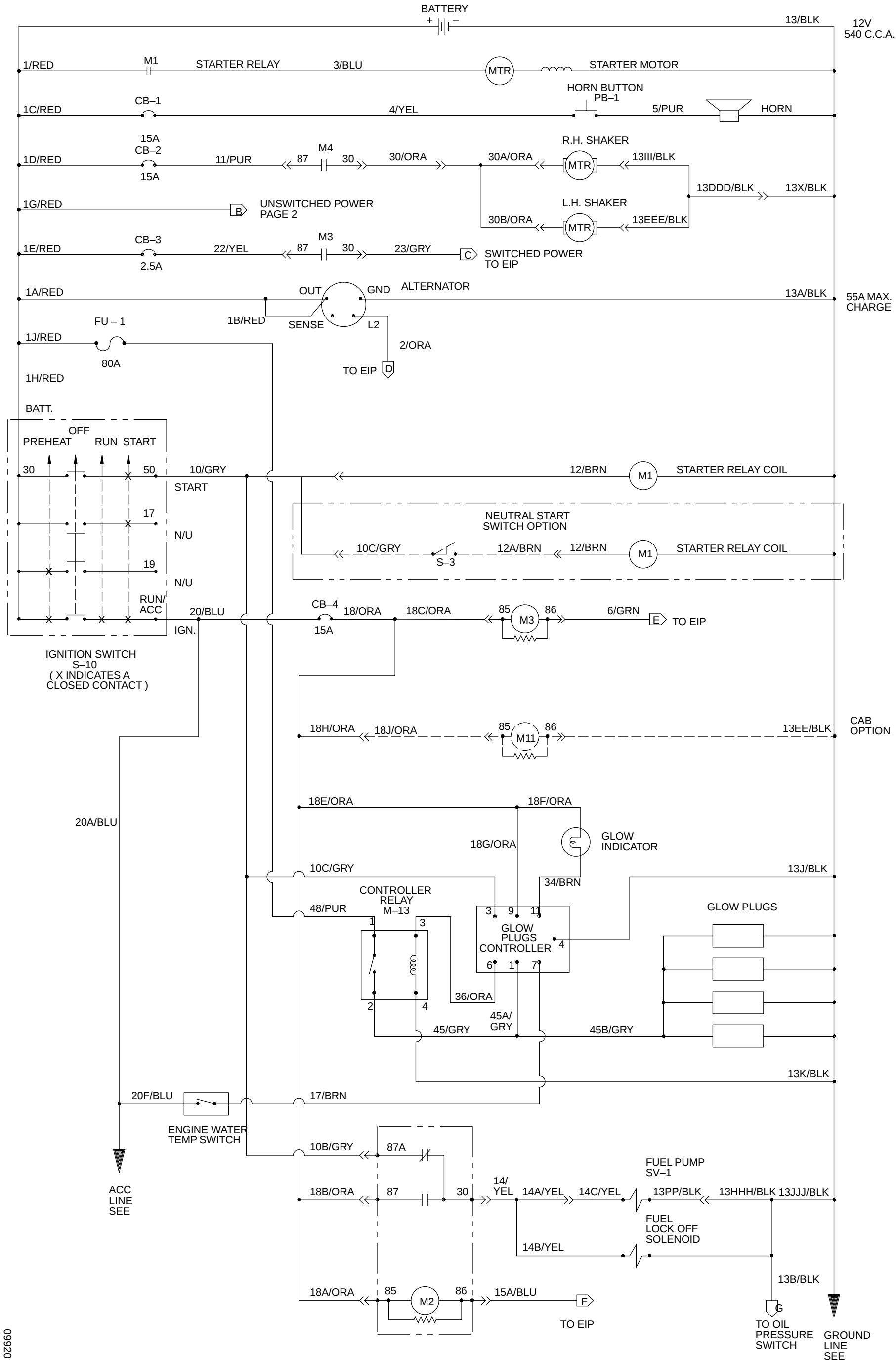
Fig. 70 - Electrical Schematic
