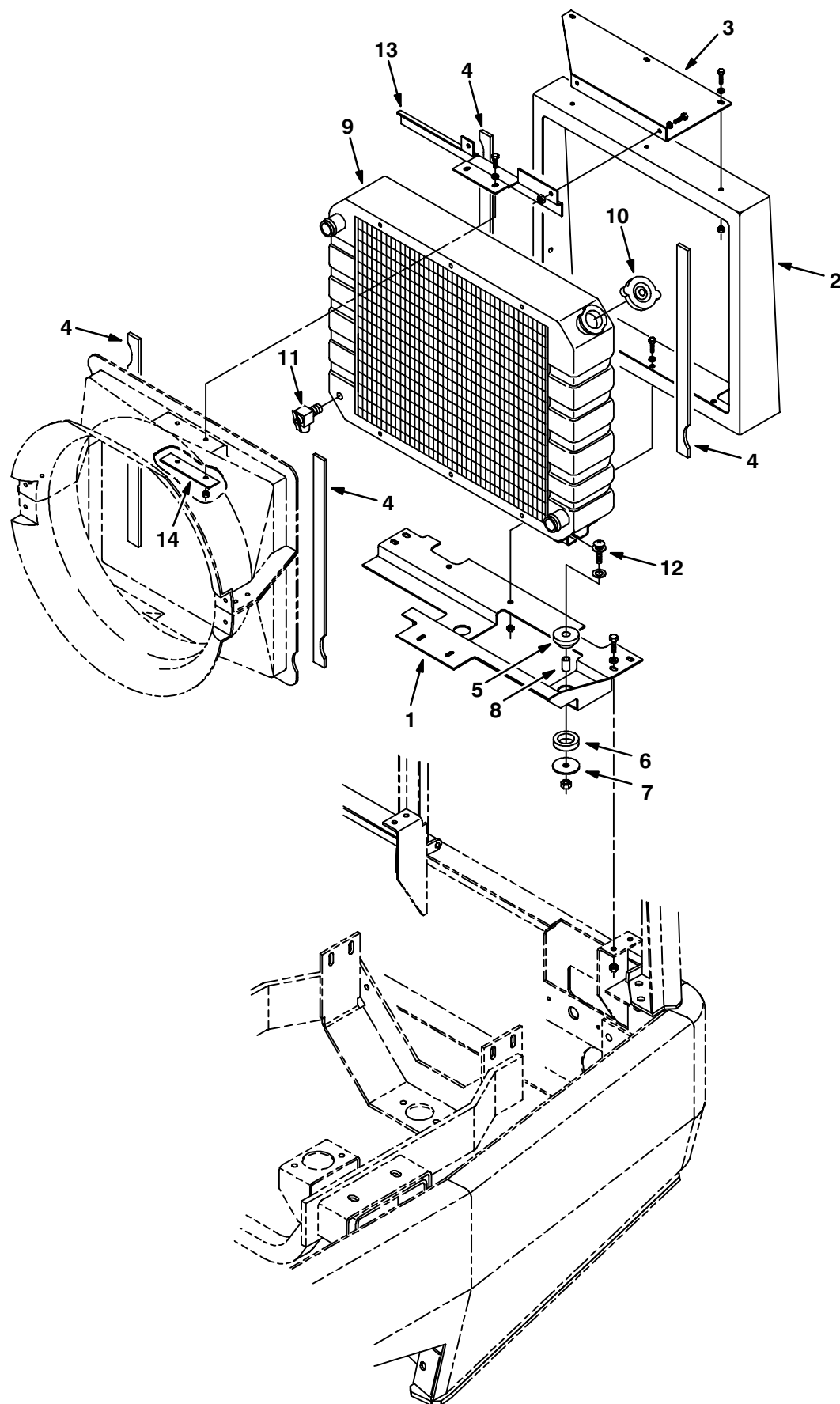
Fig. 37 – Radiator Group
