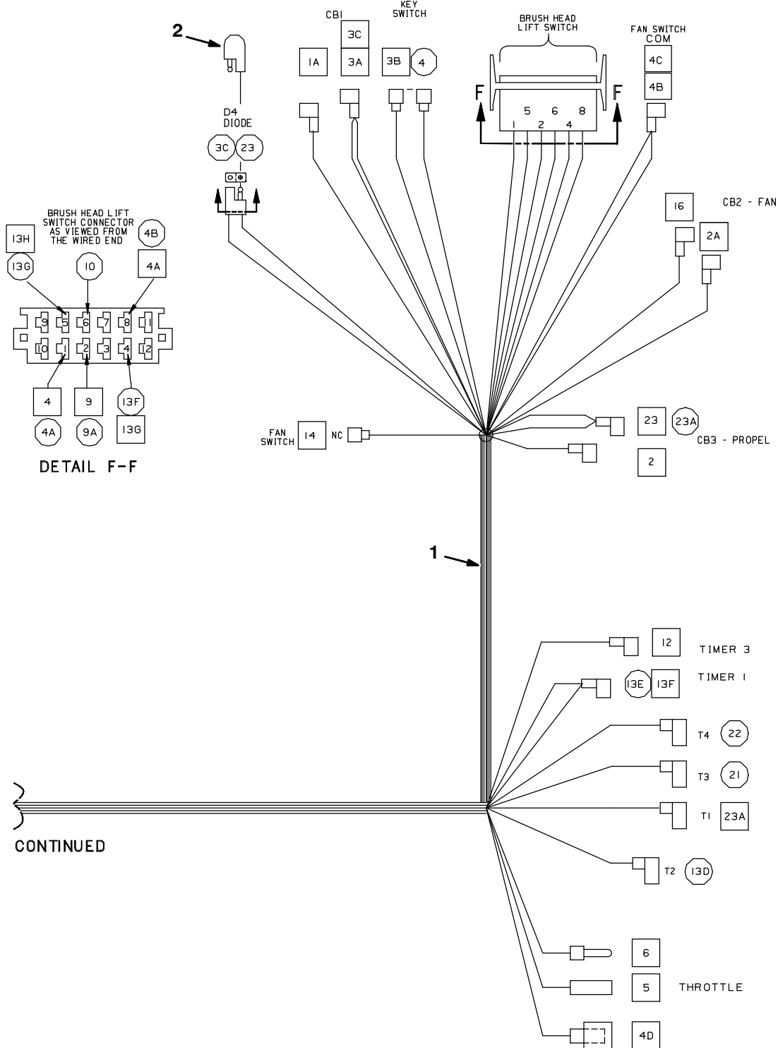
Fig. 34 – Main Wire Harness Group – Cont'd (S/N 10000000–10551745)
