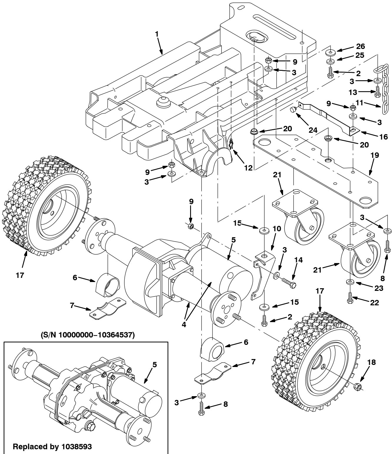
Fig. 5 – Main Frame and Drive Group (S/N 10000000–10705714)
