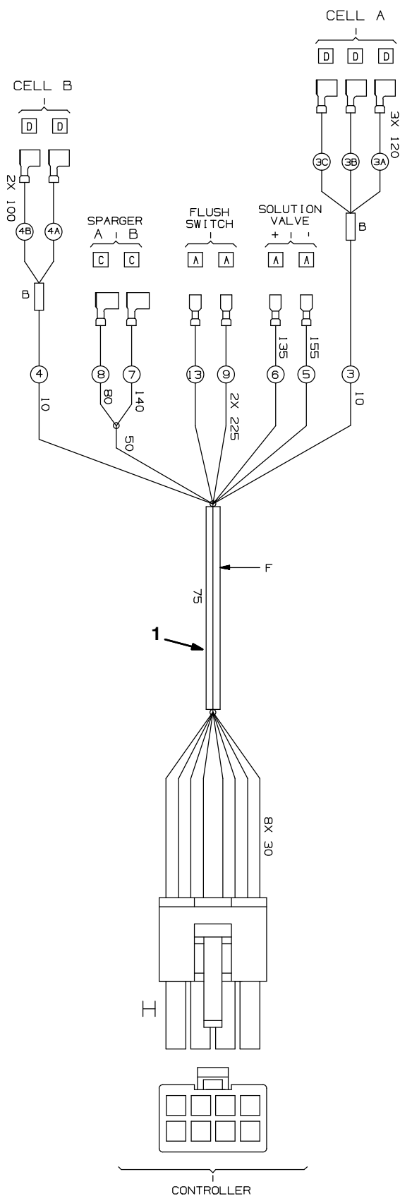
Fig. 40 – ec-H2O Main Control Board Harness Group (S/N 10489542–10740686)
