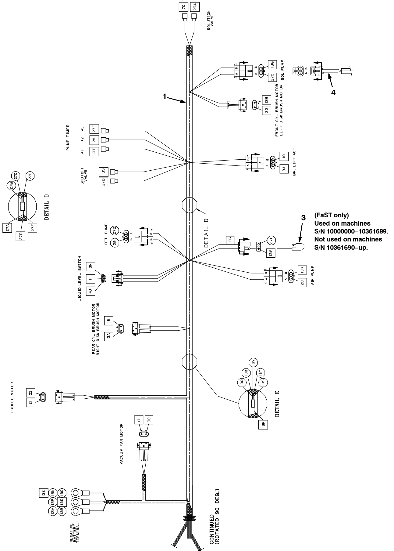
Fig. 34 – Main Wire Harness Group – Cont'd (S/N 10000000–10551745)
