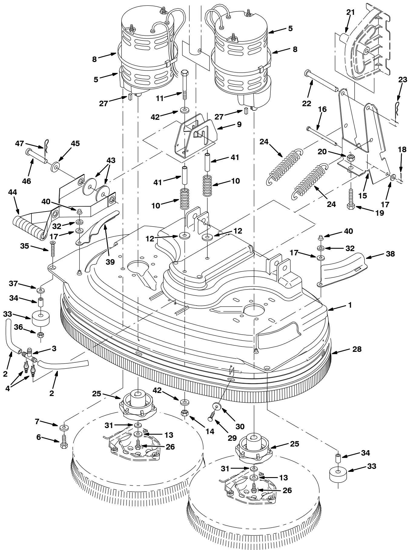
Fig. 12 – Scrub Head Kit, Model 900D, 900 mm (36 in) (S/N 10000000–10548157)
