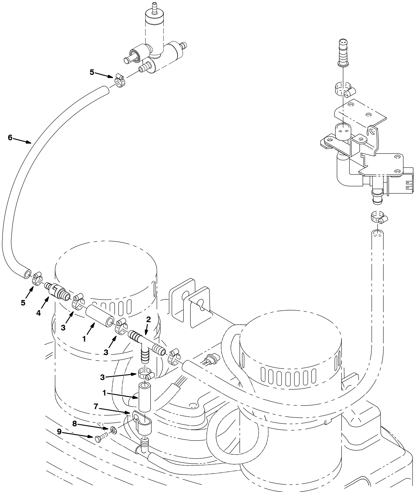
Fig. 4 – FaST Solution Supply Group, Disk Scrub Head (S/N 10361690– )
