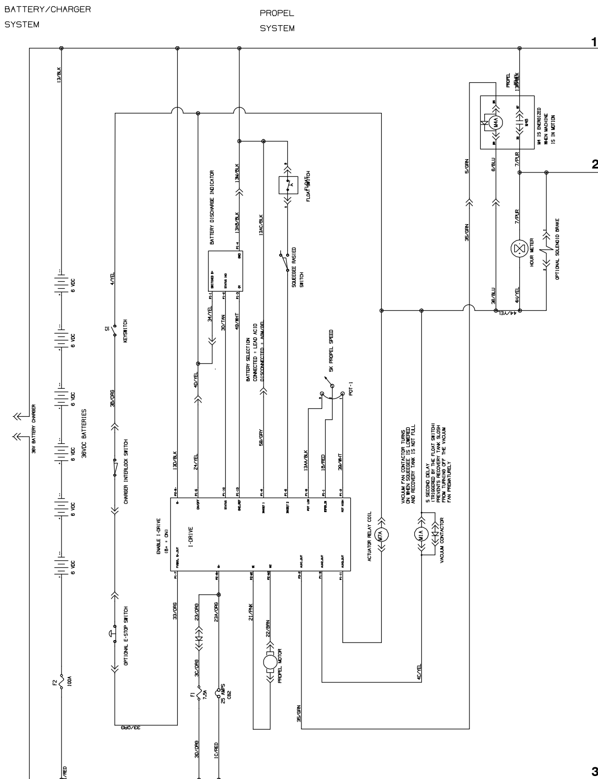
Fig. 32 – Electrical Schematic, Standard, Fast, & ec-H 2 O Models (S/N 10714325–10740686)
