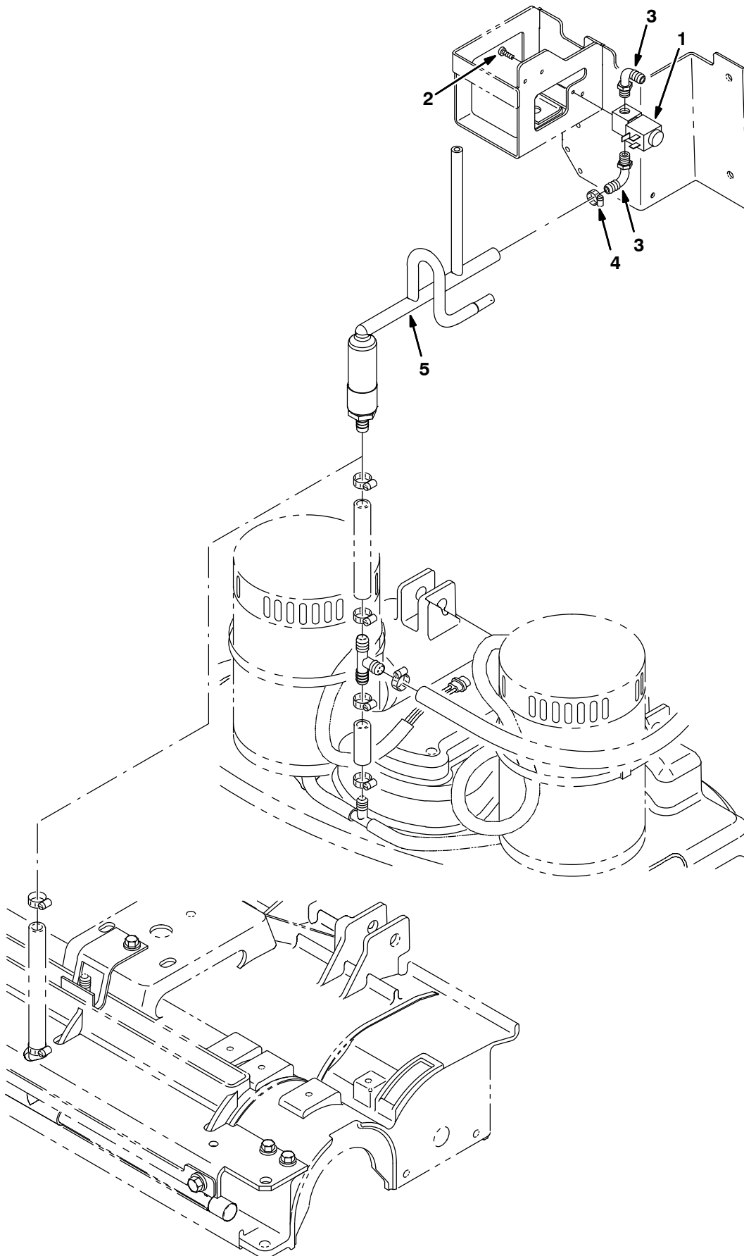
Fig. 7 – FaST Foam Filter Group (S/N 10000000–10361689)
