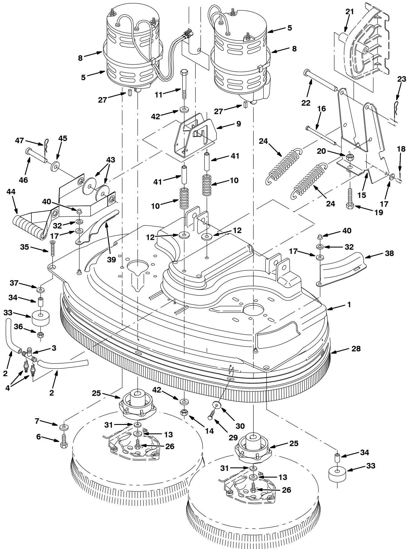
Fig. 10 – Scrub Head Kit, Model 800D, 800 mm (32 in) (S/N 10000000–10548157)
