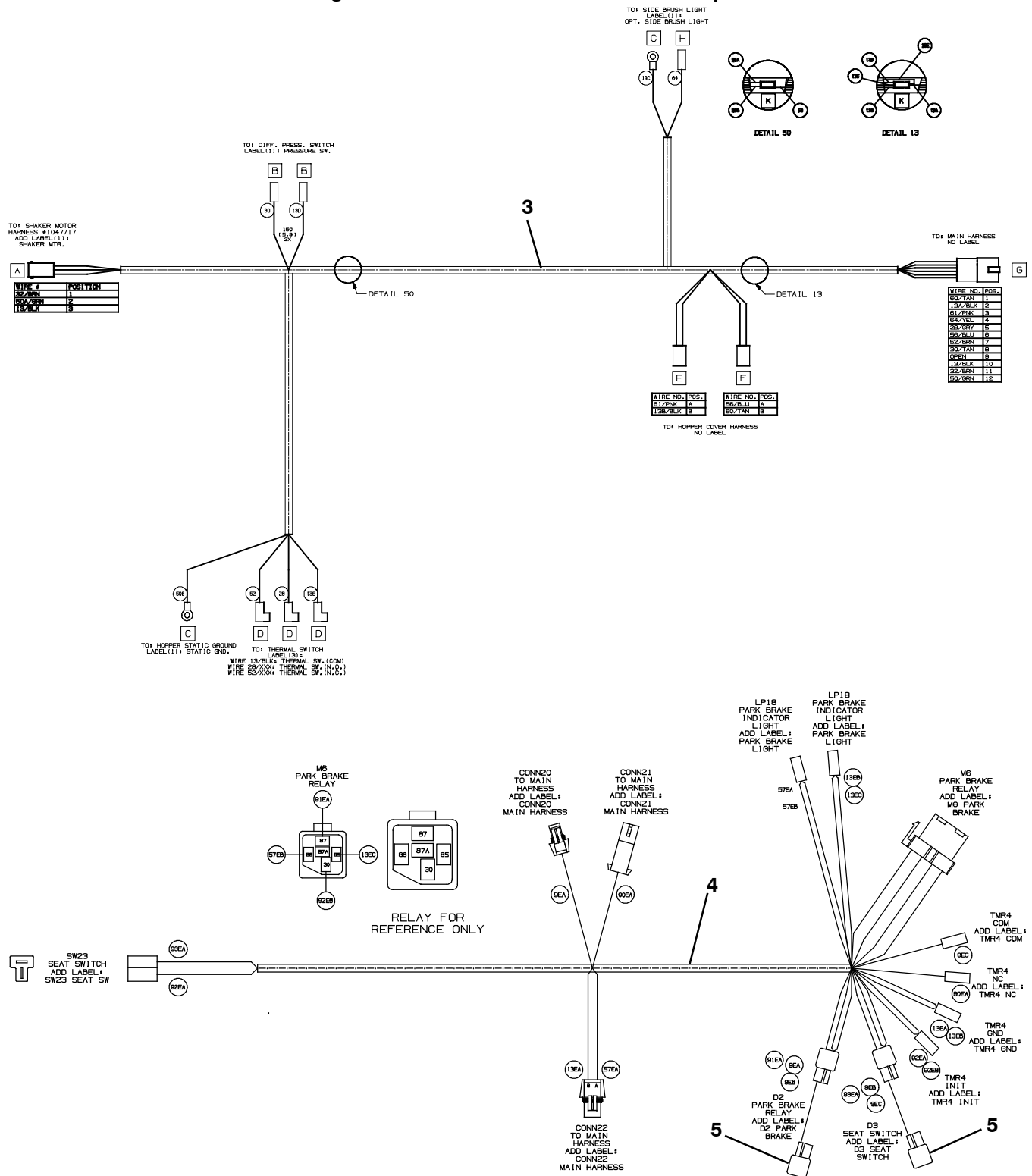
Fig. 64 - Electrical Wire Harness Group
