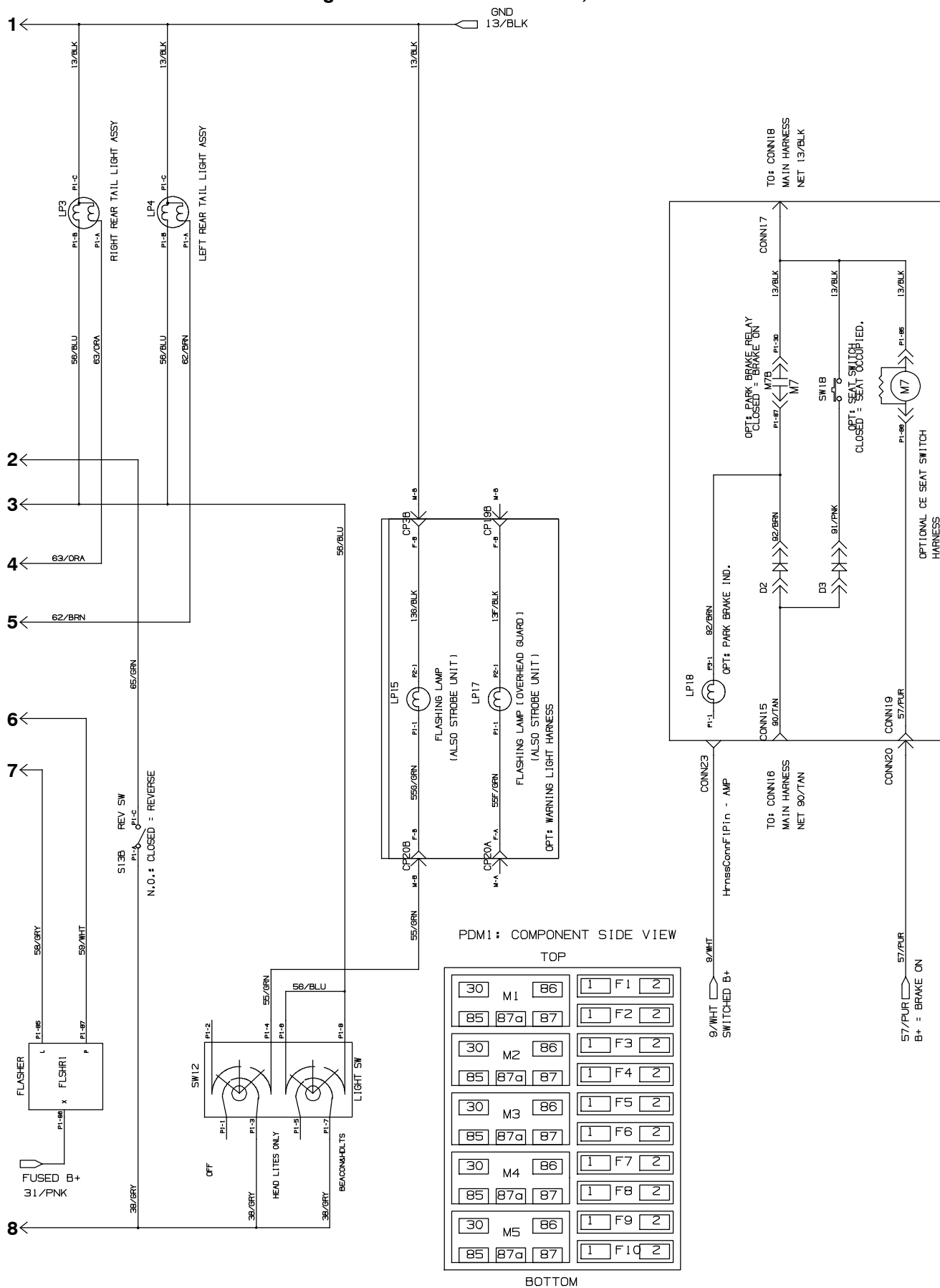
Fig. 63 - Electrical Schematic, S30 XP
