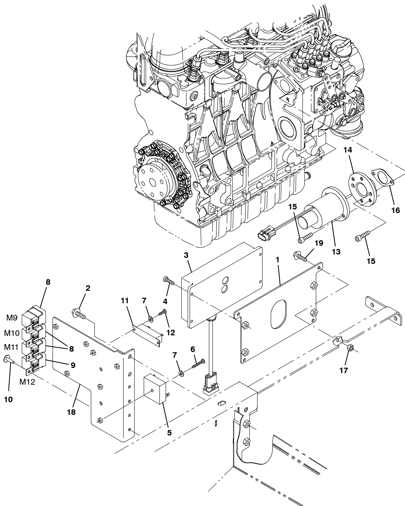
Fig. 14 - Engine Governor and Electrical Group, Diesel
