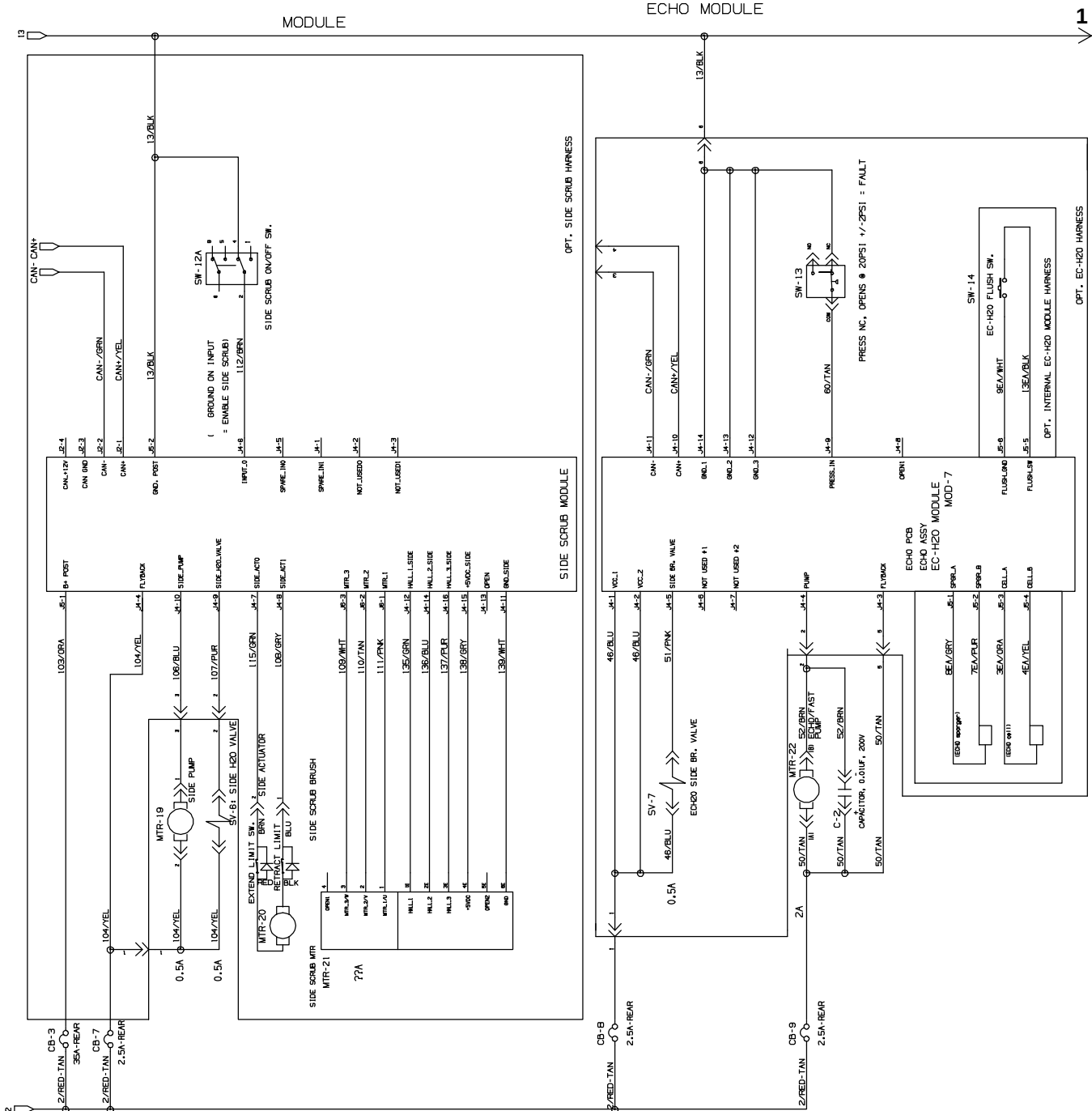
Fig. 51 – Electrical Schematic (000000–010999)
