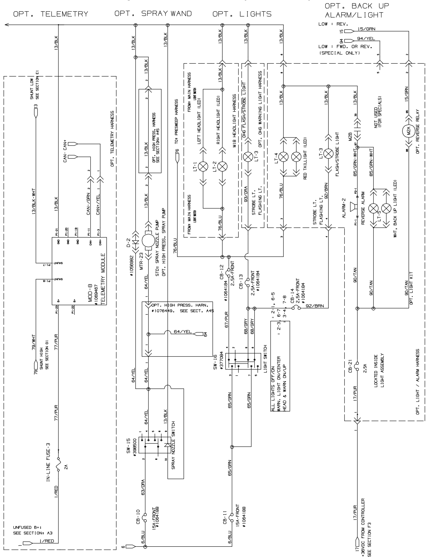
Fig. 52 – Electrical Schematic (011000–011999)
