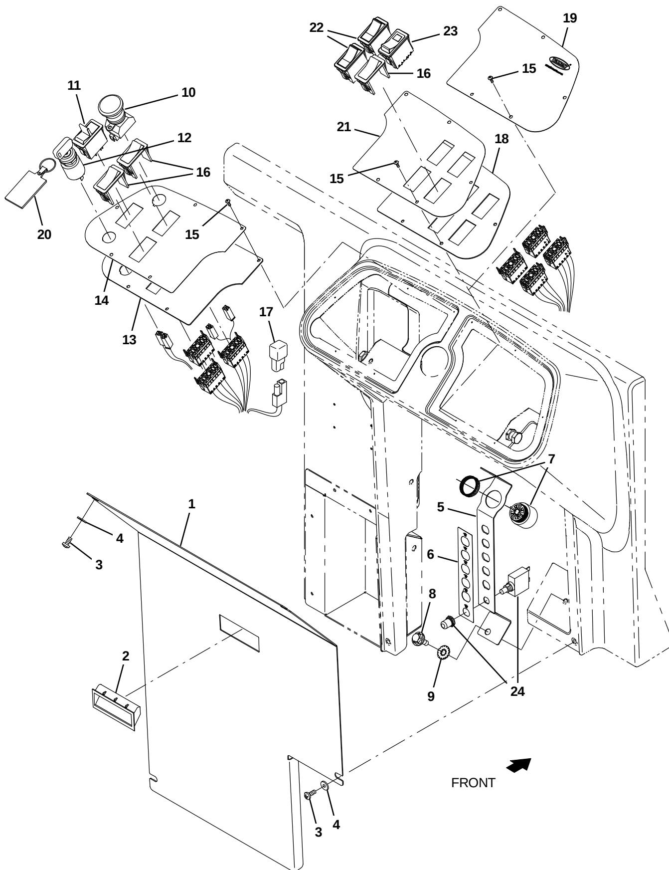
Fig. 8 – Instrument Panel Group
