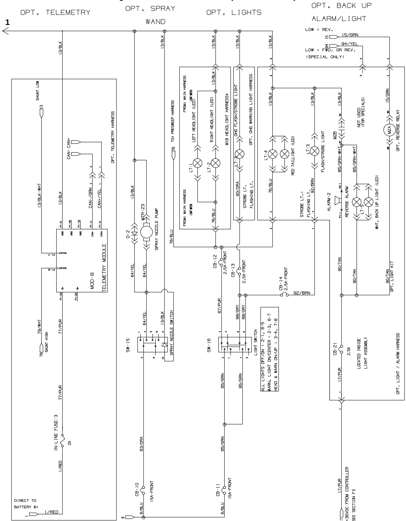
Fig. 51 – Electrical Schematic (000000–010999)
