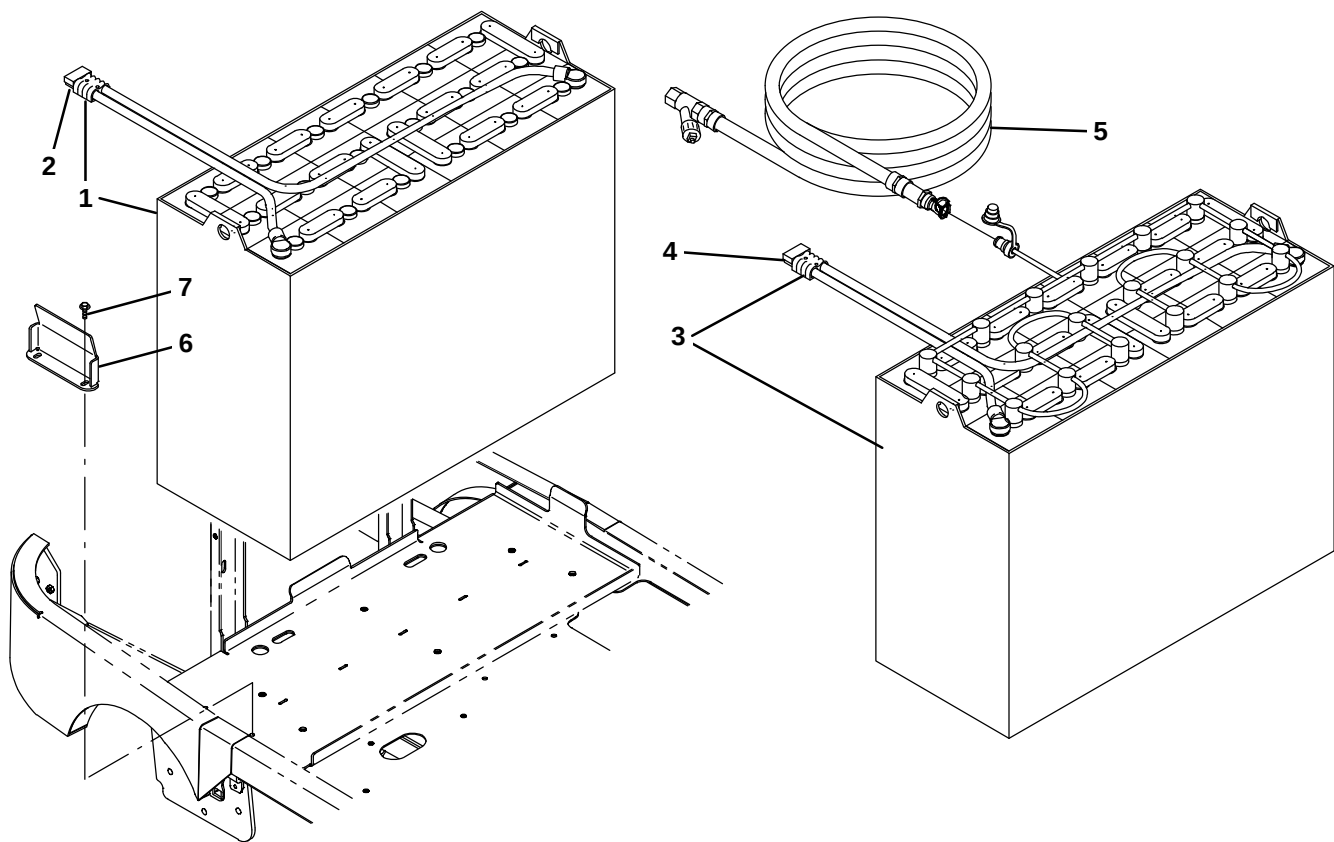
Fig. 27 – Battery and Charger Group, 930AH
