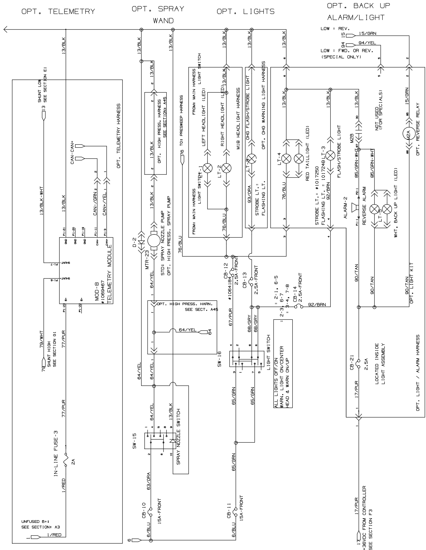
Fig. 53 – Electrical Schematic (012000- )
