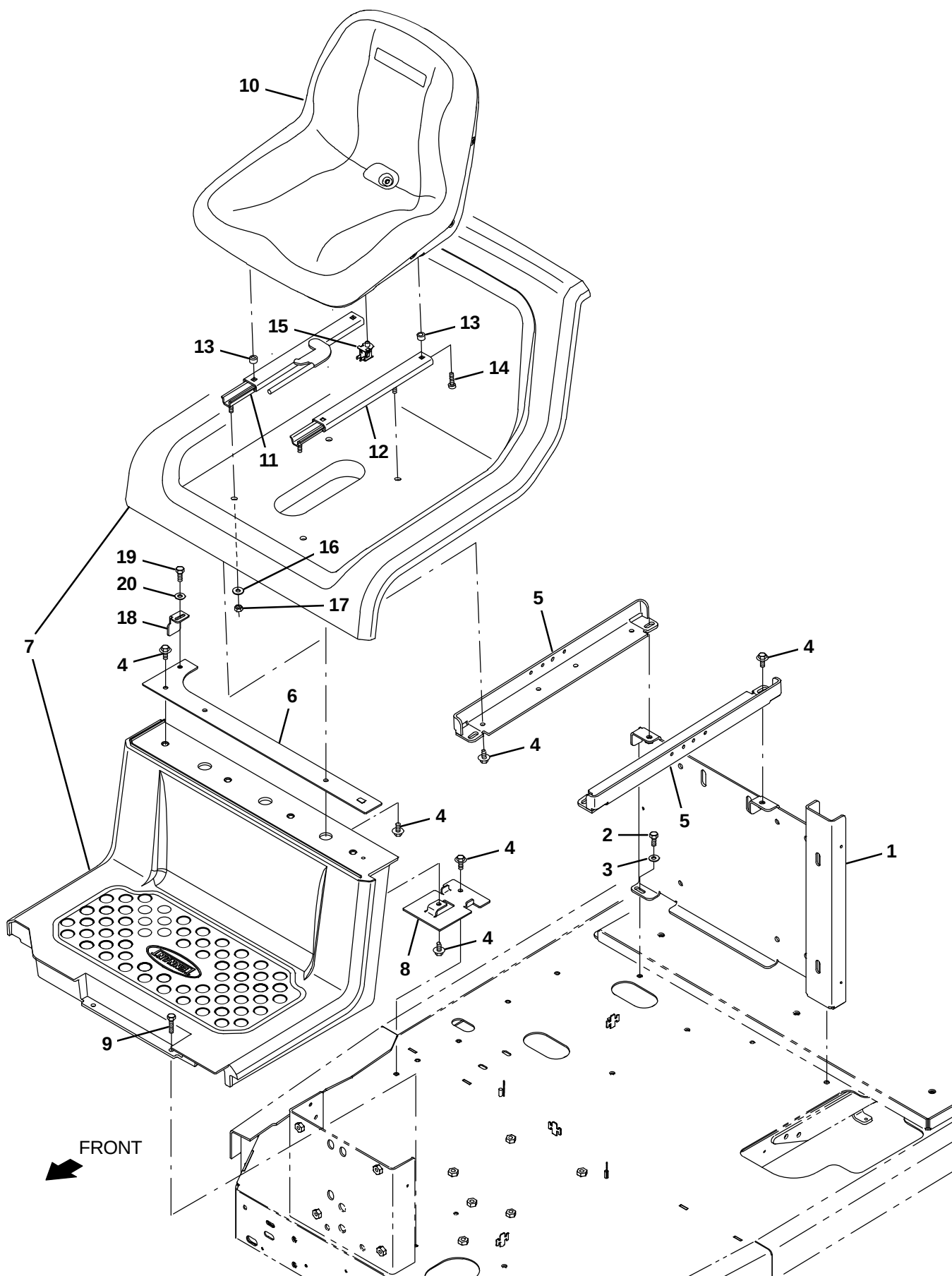
Fig. 9 – Seat Group
