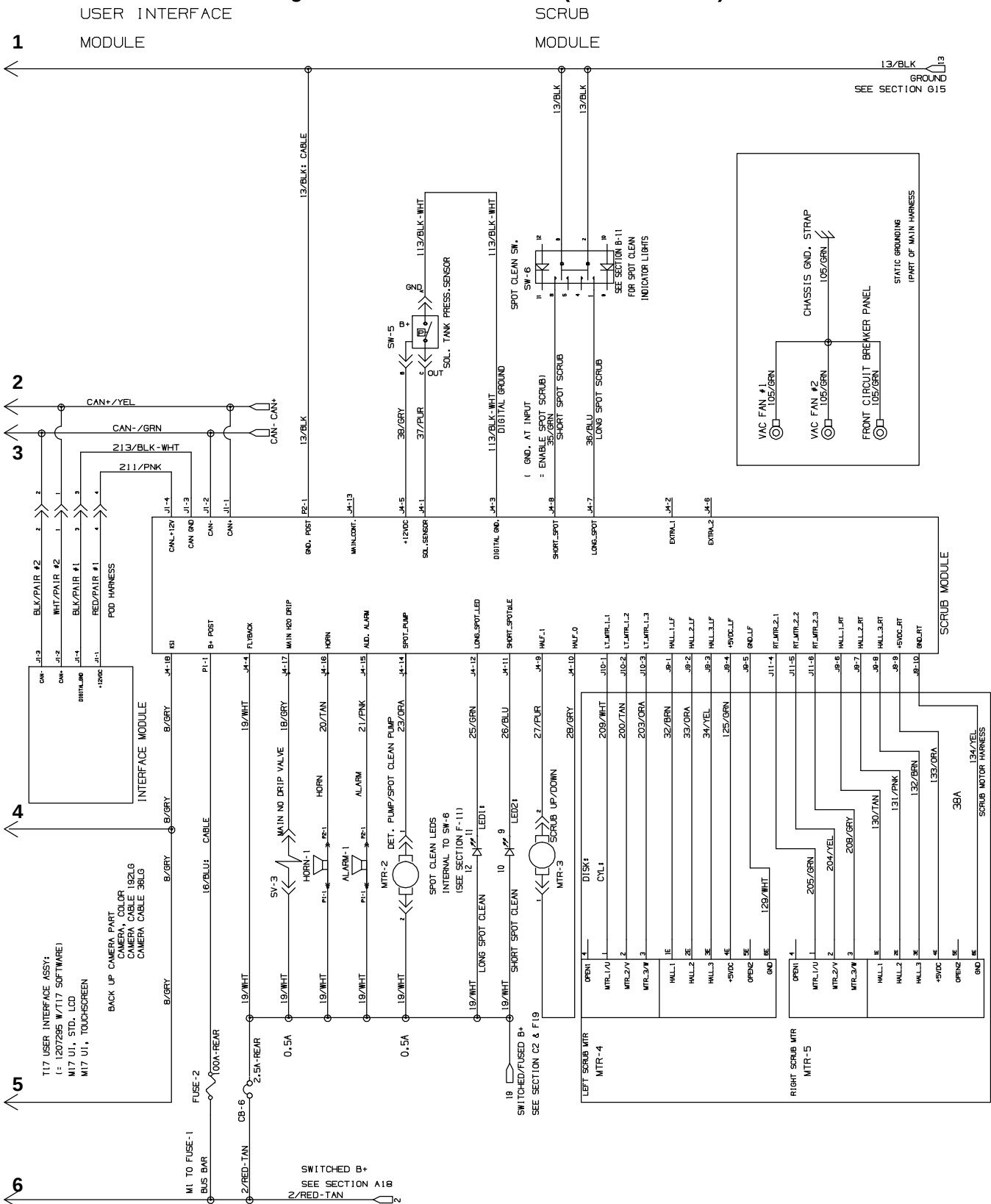
Fig. 51 – Electrical Schematic (000000–010999)
