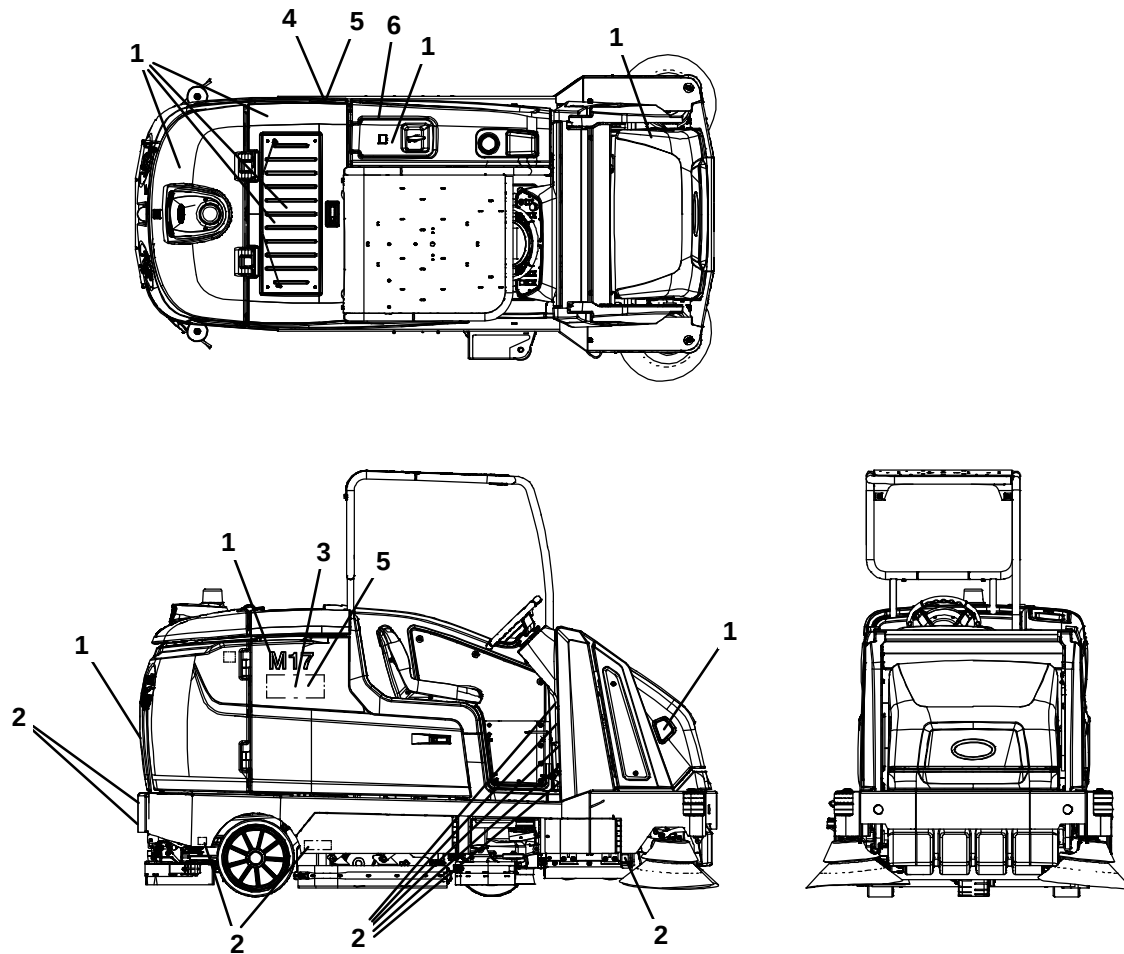
Fig. 55 – Label Group
