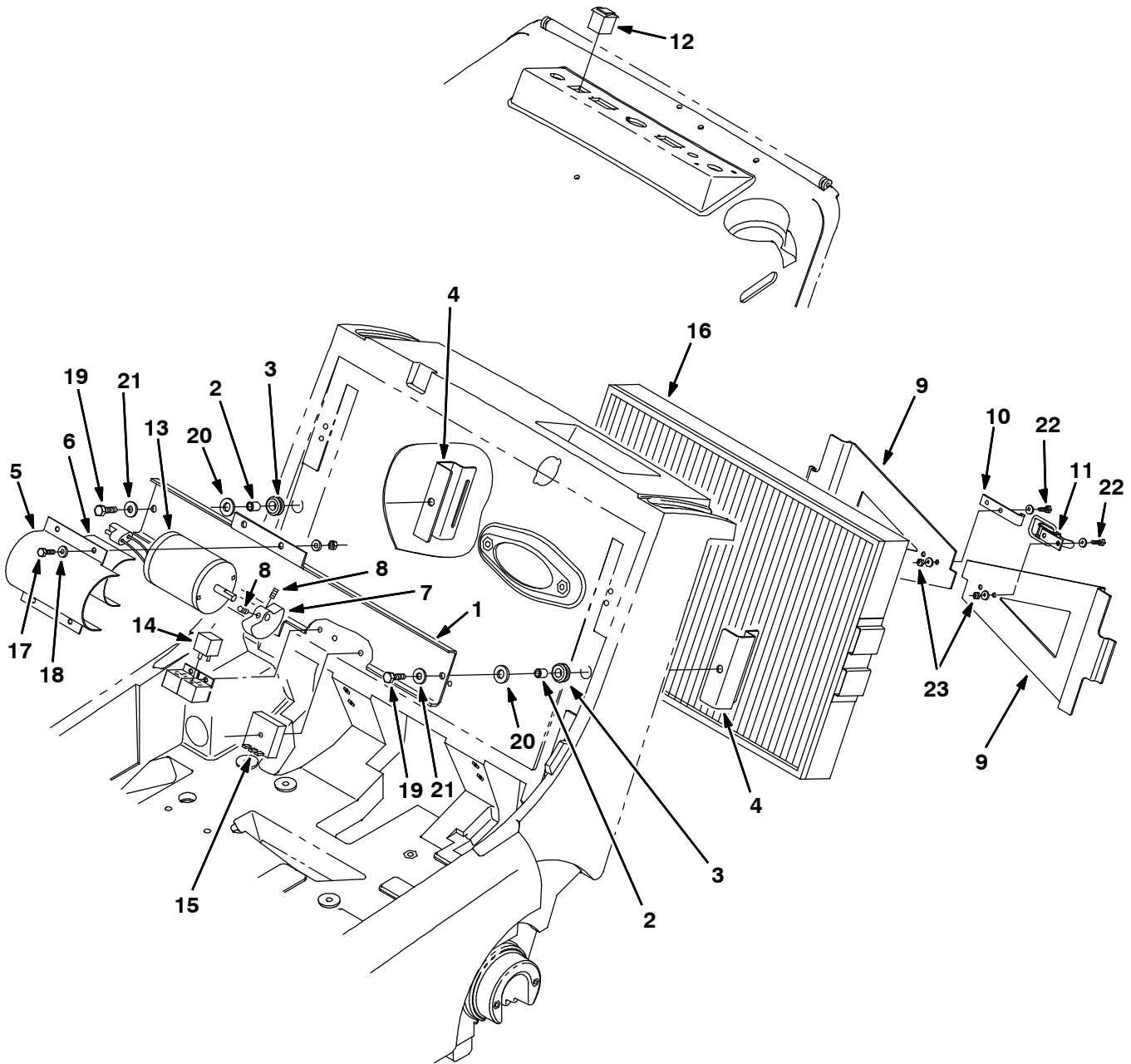
Fig. 10 - Panel Filter Group
