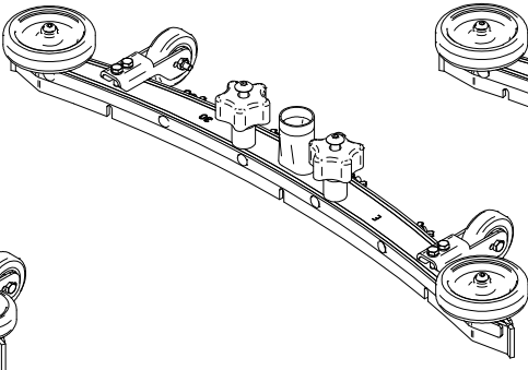
30 INCH SQUEEGEE ASSEMBLY 150-7180
