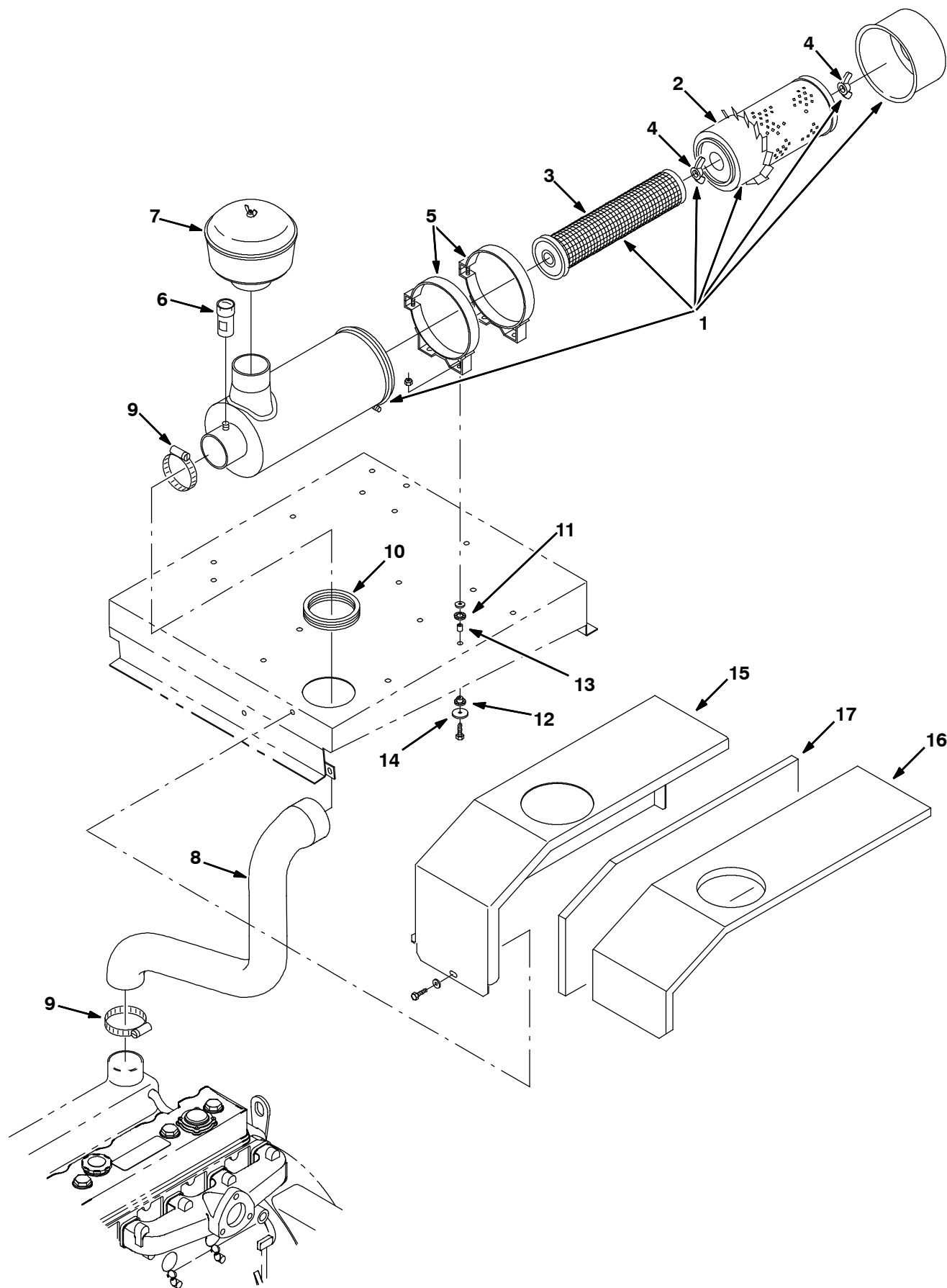
Fig. 24 - Engine Air Cleaner Group (004000-006008)
