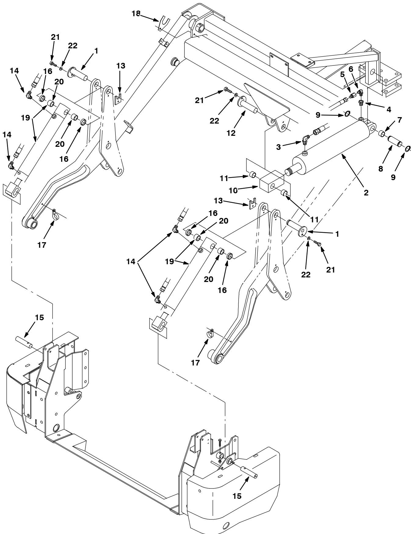
Fig. 12 - Hopper Lift Cylinders Group
