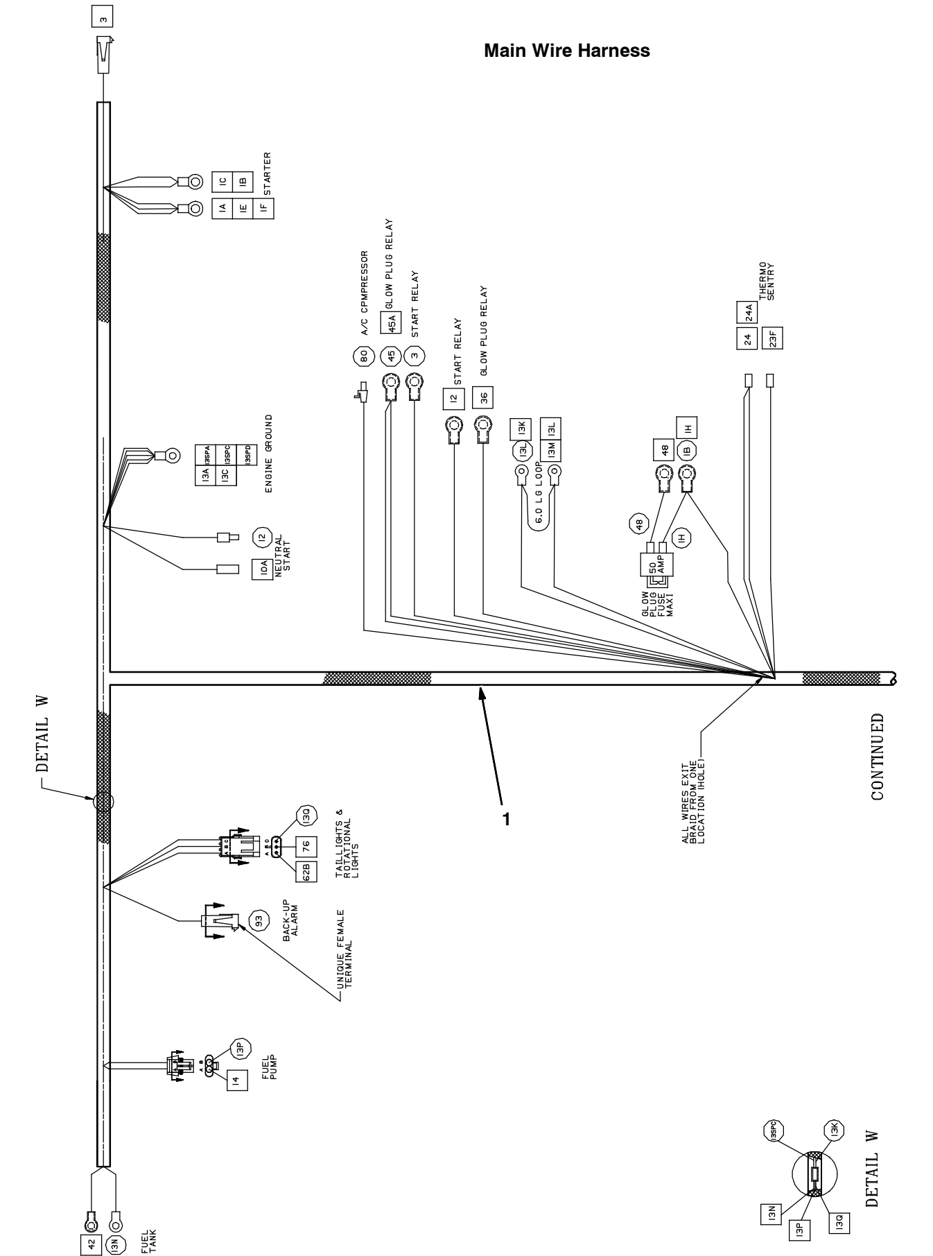
Fig. 67 - Wire Harnesses Group, Diesel, Main (006009- )
