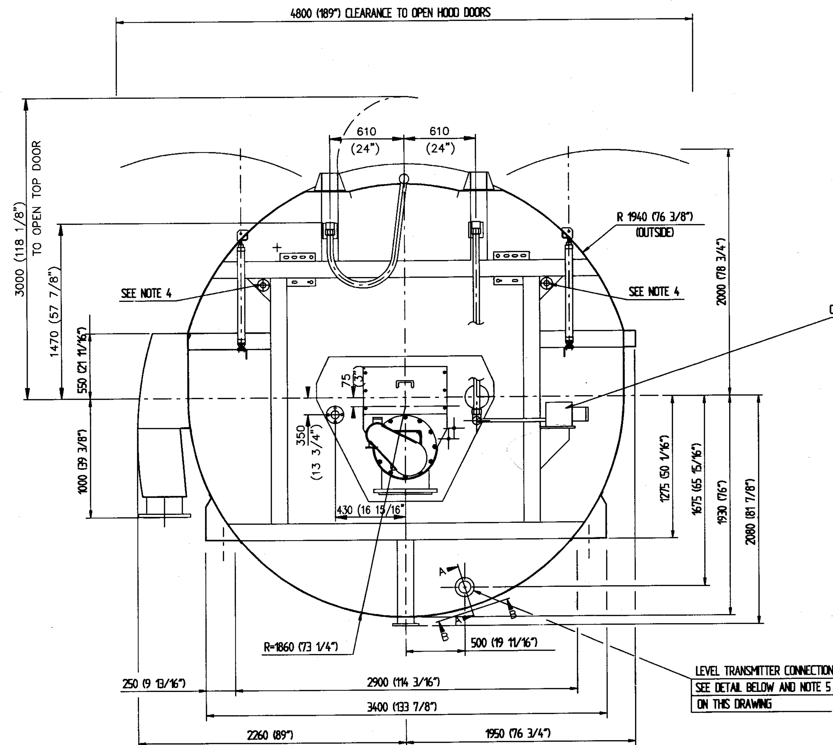
DISCHARGE END VIEW
