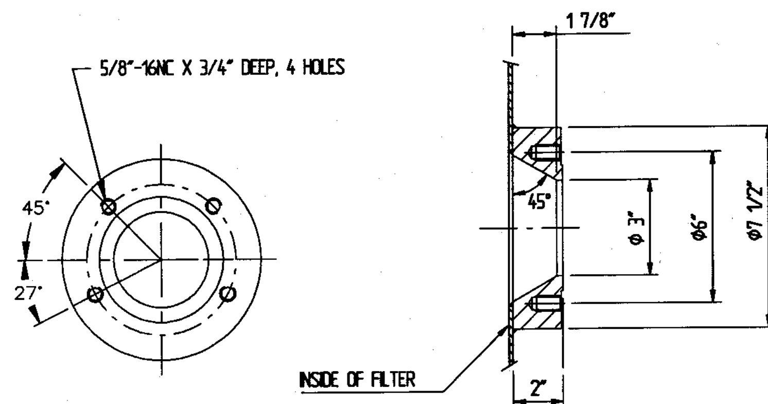
LEVEL TRANSMITTER CONNECTION DETAIL
