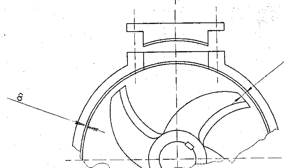
mm 15 Nominal gap
