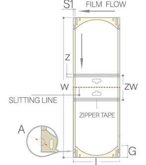
单 / 双线站立拉链三边封 2 Lane Stand Pouch With Zipper
