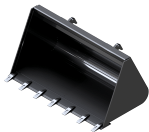
Standard Digging Bucket with Teeth (Compact machines) - BS 1850 / 740 T
