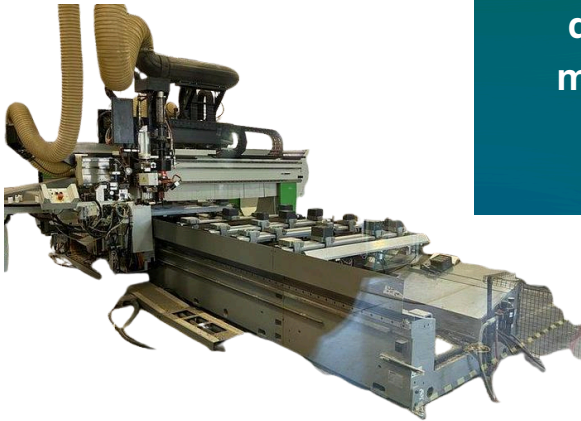
Biesse Rover B 1650 G Edge, Pod & Rail CNC with 4 Coil Edgebanding, Bsolid Software $222,000 (USD)
