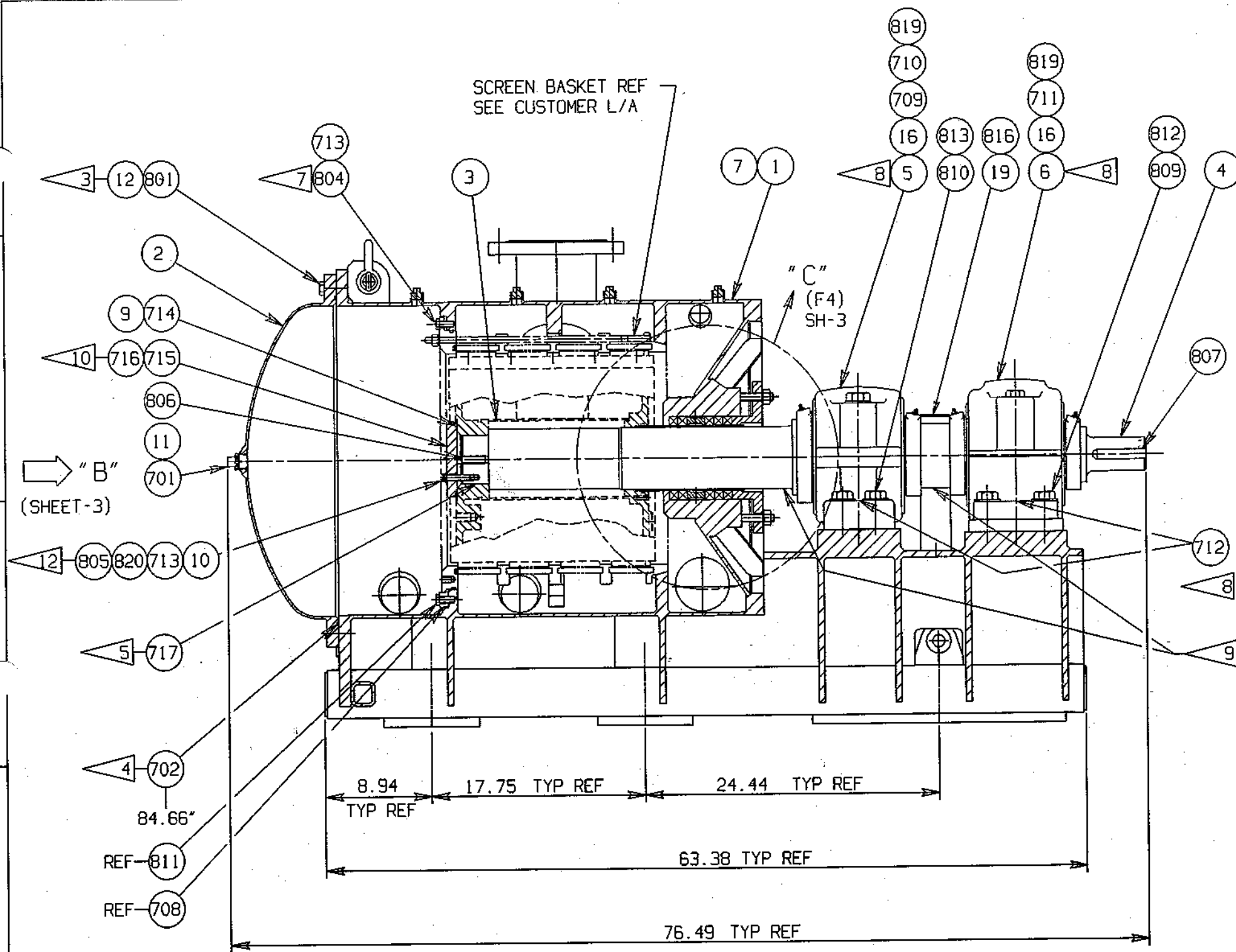
SECTION "A" - "A" (G1)
