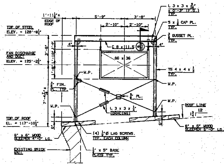
SECTION 3/8" = 1'-0"
