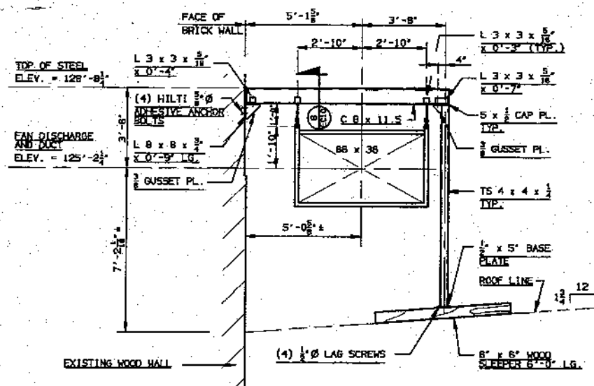
SECTION 3/8" = 1'-0"
