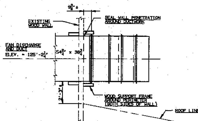
SECTION 3/8" = 1'-0"
