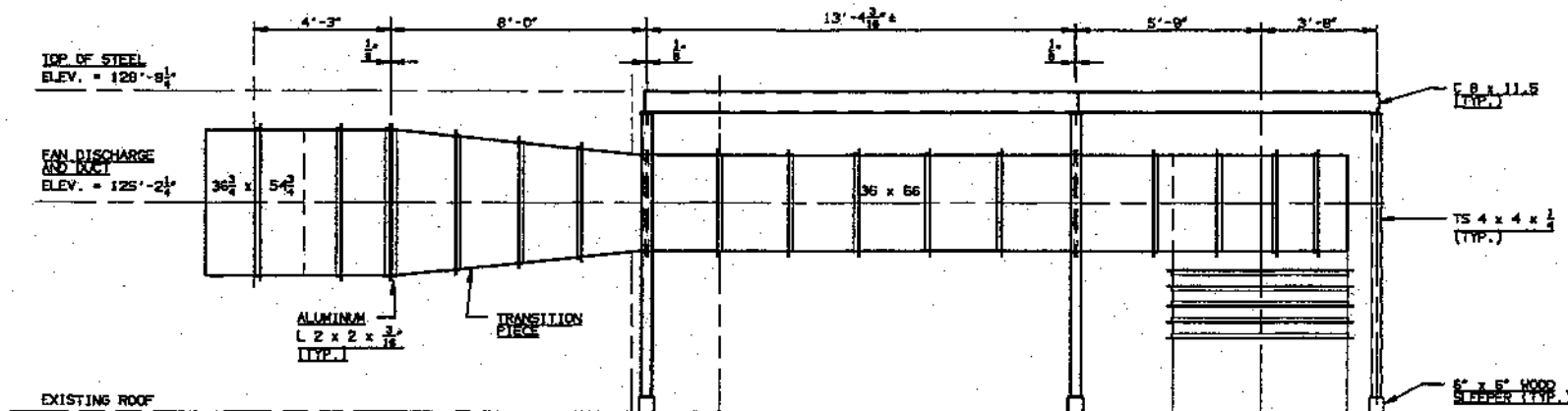
ELEVATION 3/8" = 1'-0"
