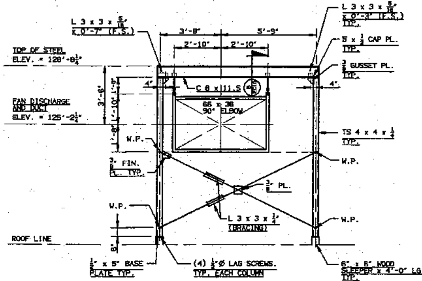
SECTION 3/8" = 1'-0"
