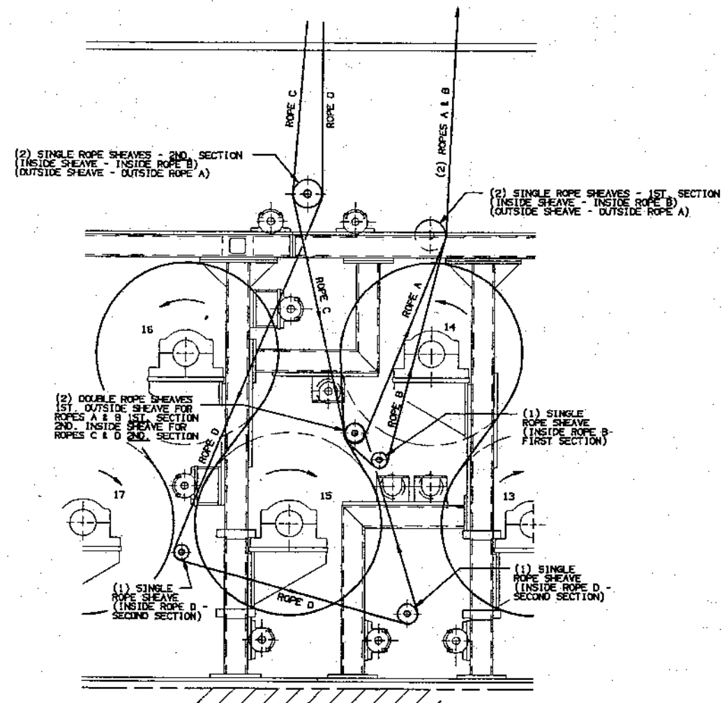
FIRST AND SECOND SECTION ROPE SYSTEM TRANSFER DETAIL
