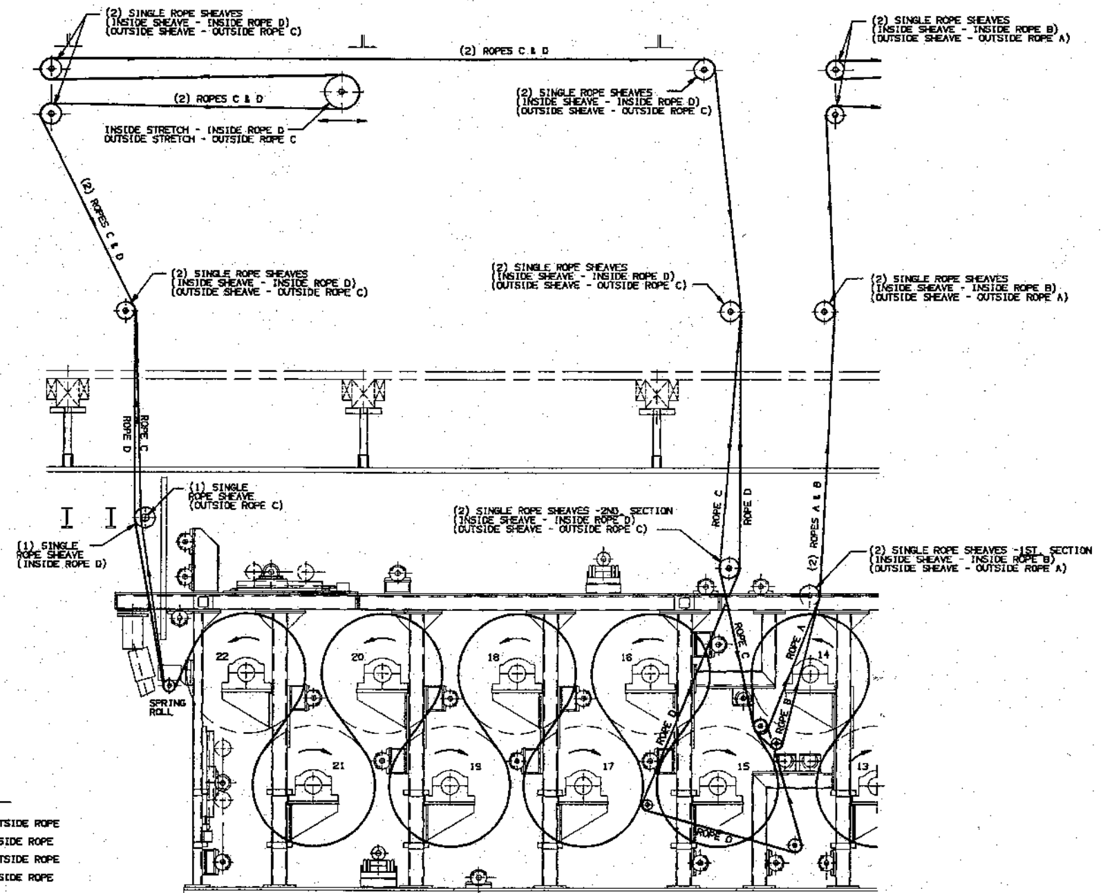
ROPE SYSTEM - SECOND DRYER SECTION TENDING SIDE ELEVATION
