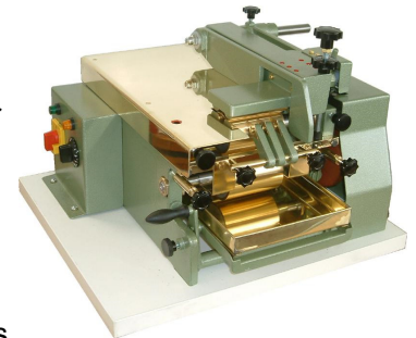
Two roller edge gluer Mod. CORONEL 90 mm
