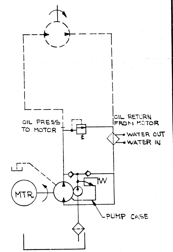
SCHEMATIC OF HYDRAULIC CIRCUIT
