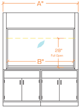
elevation view – bench top fume hood
