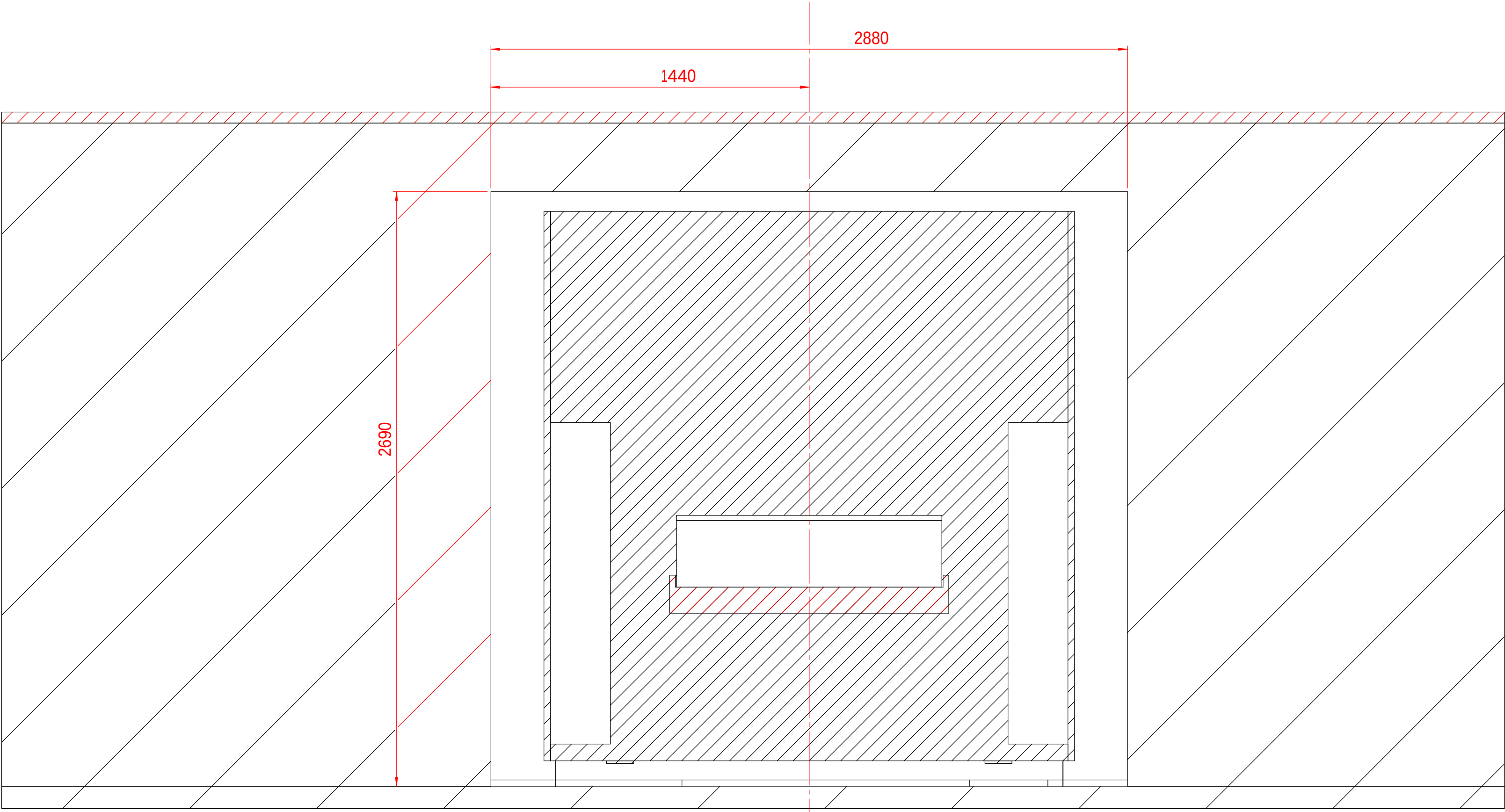
View A-A wall opening HQL 1 : 16
