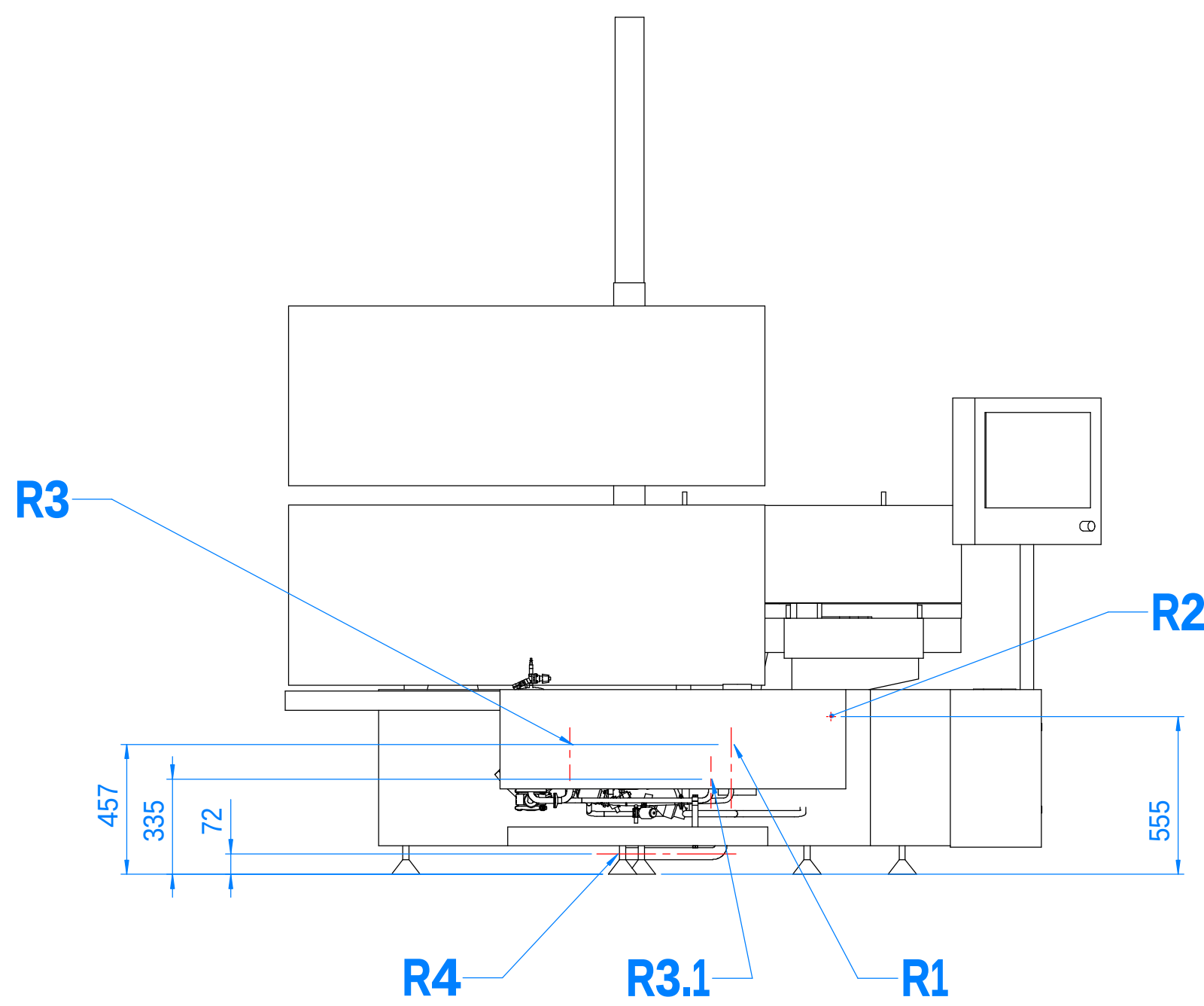
Side view RRN 1:20
