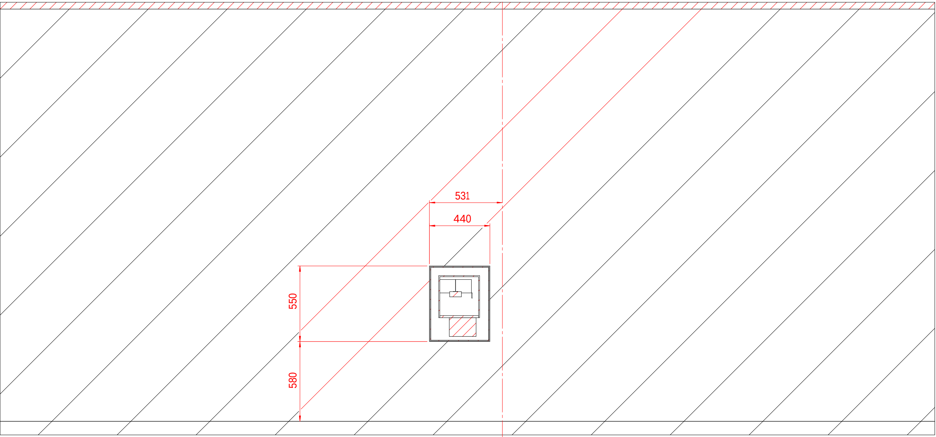
View C-C wall opening VRK outfeed 1 : 16
