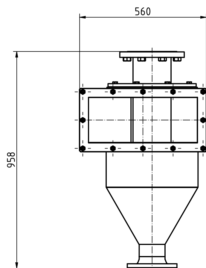
Cyclone ( 1 : 10 ) approx. 70 kg
