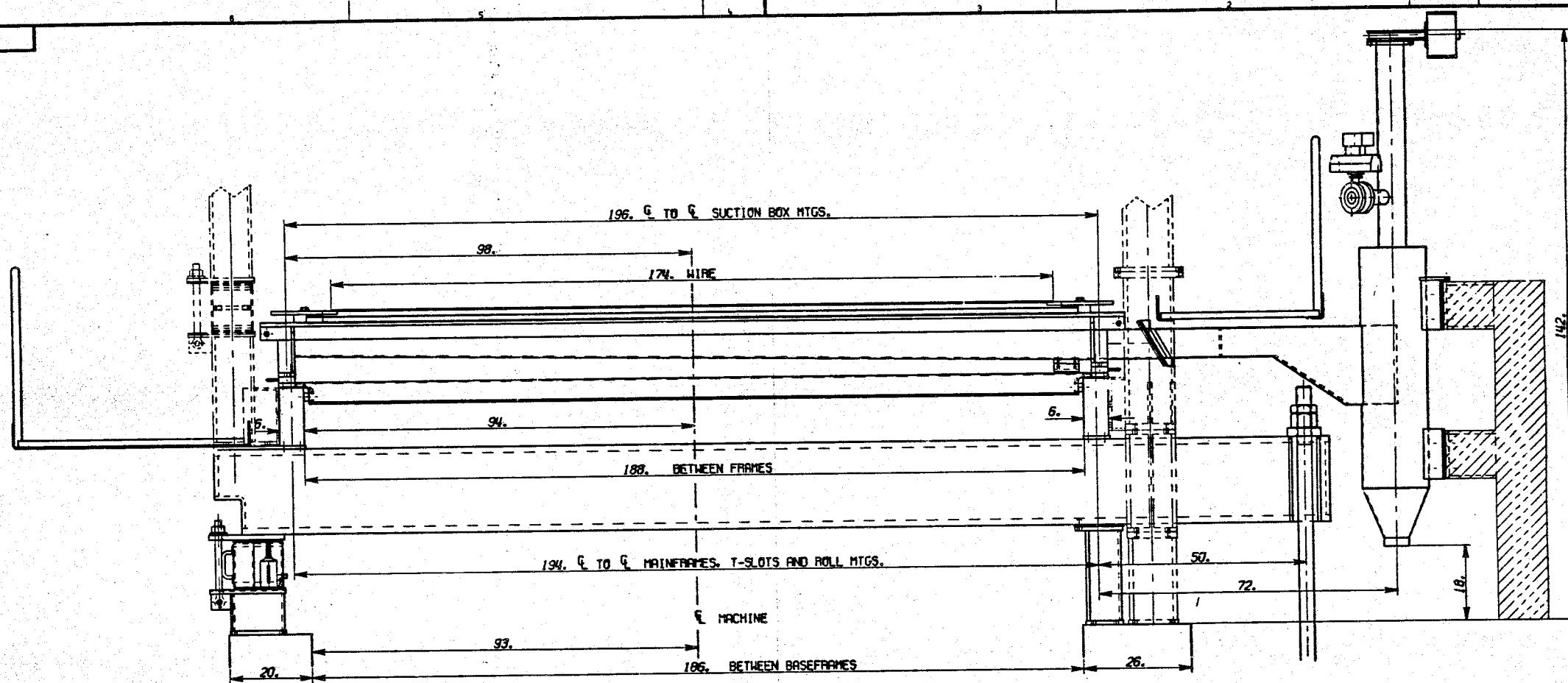
VIEW AT CANTILEVER BEAM #2
