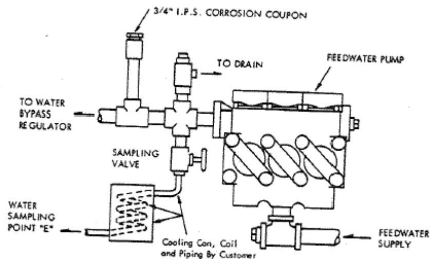
Figure 8, Typical Pump Piping
