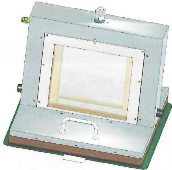
Thermal Fixture with Probe-Through Windows
