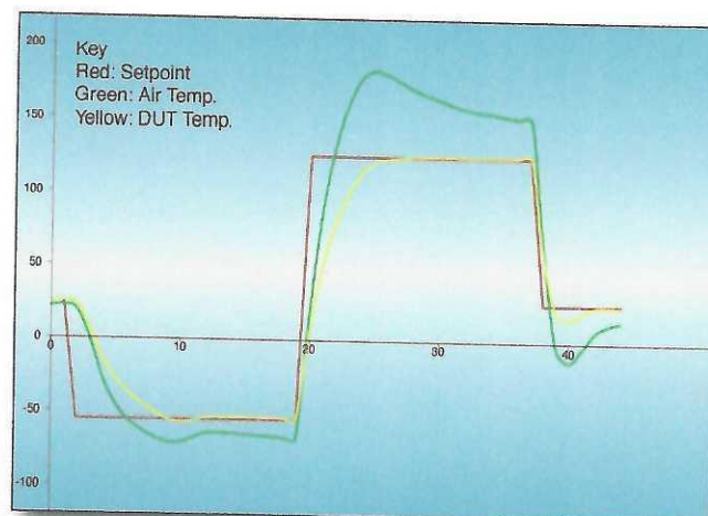
Typical Device Temperature Response
