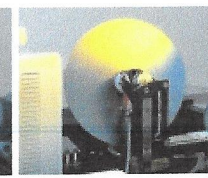
Back side periphery macro inspection (using a fiber optic illuminator)
