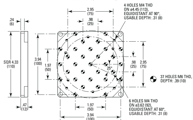
MODEL SHOWN: M-ILS & M-ILS-LM INTERFACE DIMENSIONS IN INCHES (AND MILLIMETERS)
