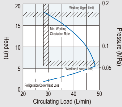
Pump w/Copper-Less Spec. Wetted Parts For RKS40□/75□J-MV
