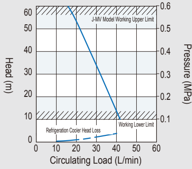
High Head / High Flow-Rate Pump For RKS402/75□J-MV
