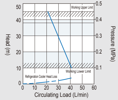
Pump w/Copper-Less Spec. Wetted Parts For RKS150□J-MV
