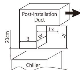
Fig. 2 Installation method when Lx and Ly are longer than 2 m.
