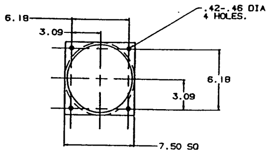
VIEW Z-Z
