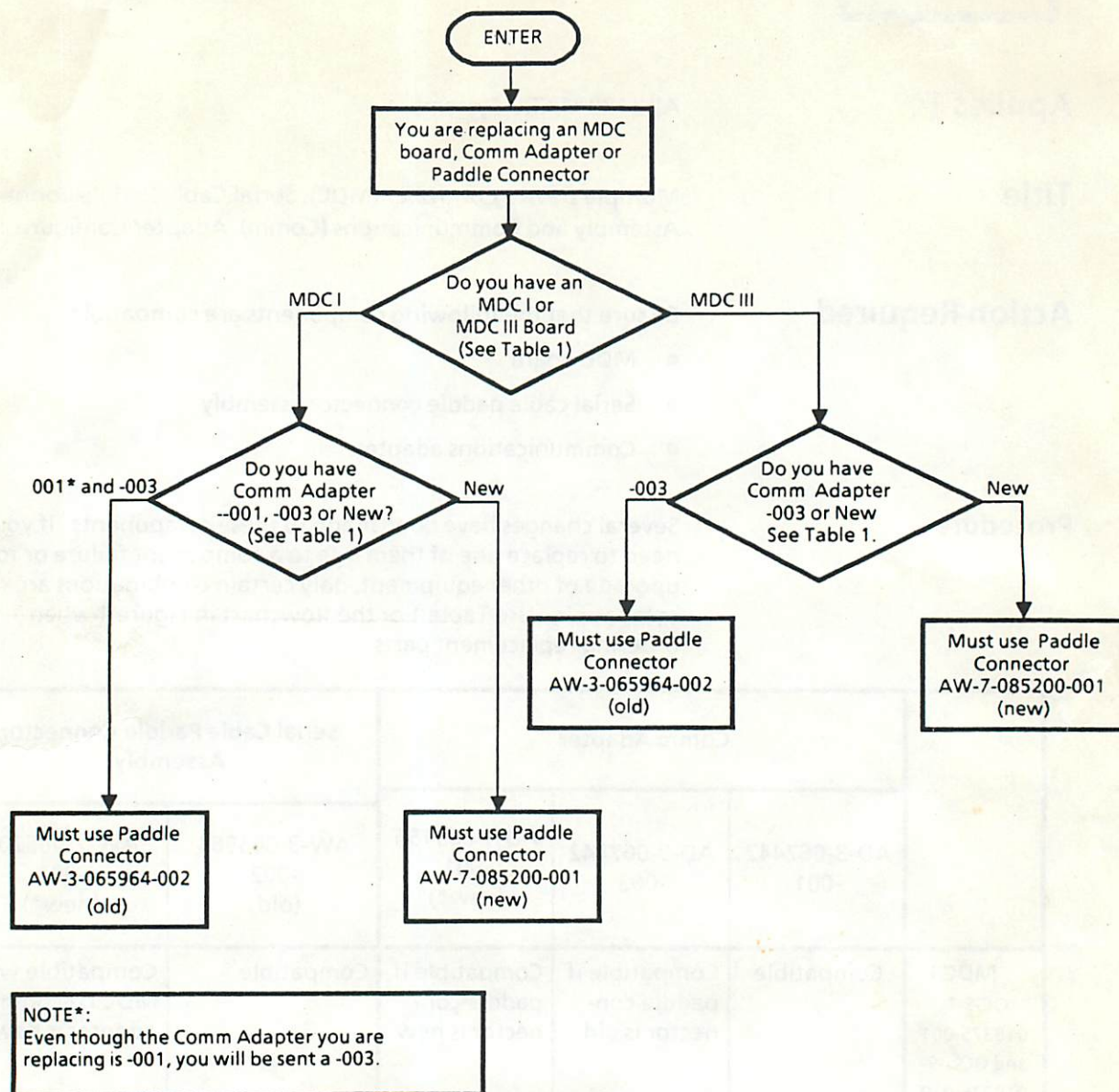
Figure 1 MDC, Paddle Connector and Communications Adapter Compatible Configurations
