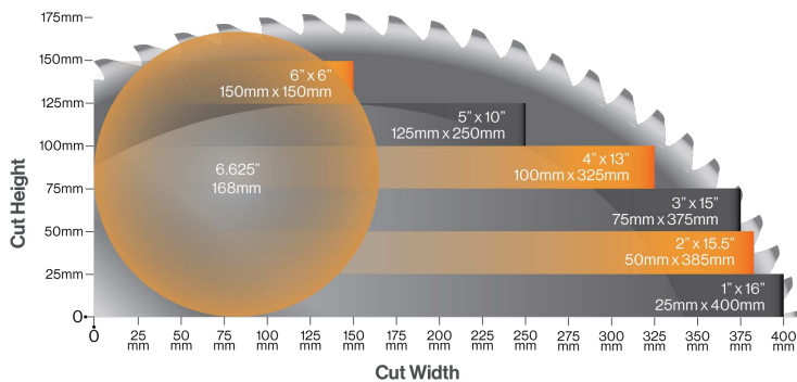
TigerSaw 1000 - Cutting Envelope 500mm Saw Blade
