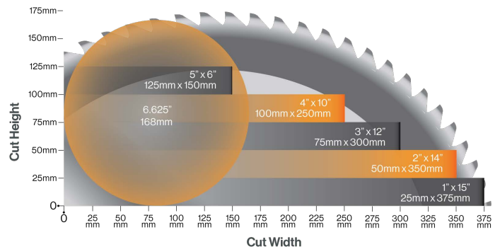
TigerSaw 1000 - Cutting Envelope 450mm Saw Blade
