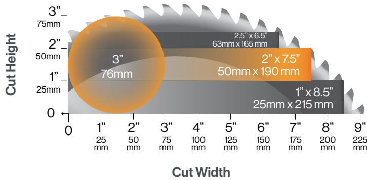
TigerSaw 1000 Compact - Cutting Envelope 14" (355mm) Saw Blade
