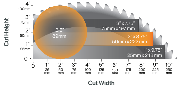
TigerSaw 1000 Compact - Cutting Envelope 16" (406mm) Saw Blade
