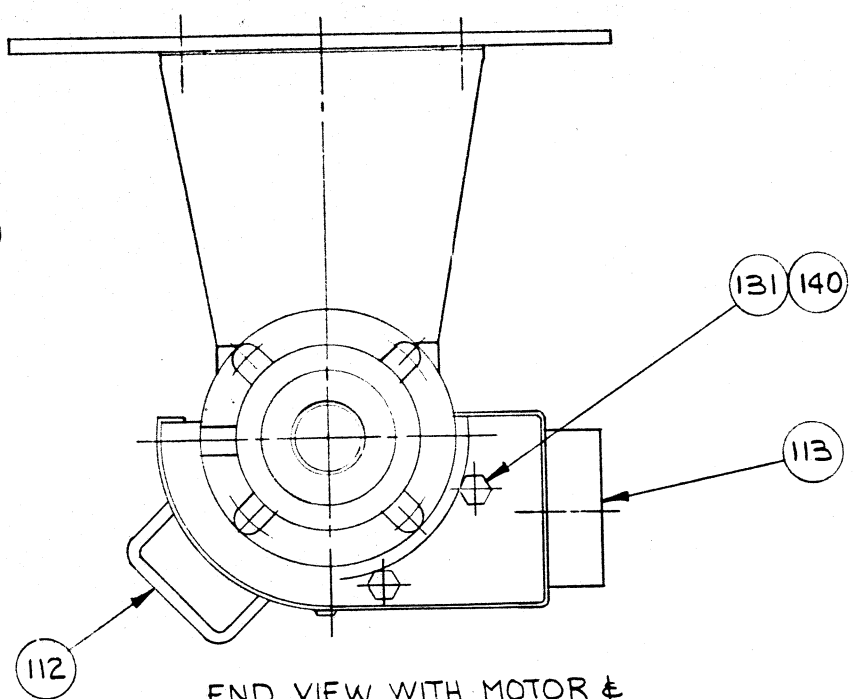
END VIEW WITH MOTOR & BRACKET REMOVED
