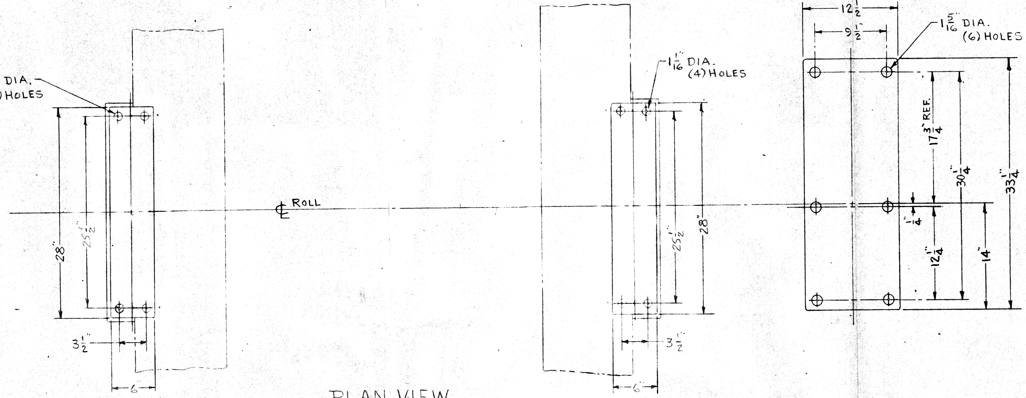
PLAN VIEW
