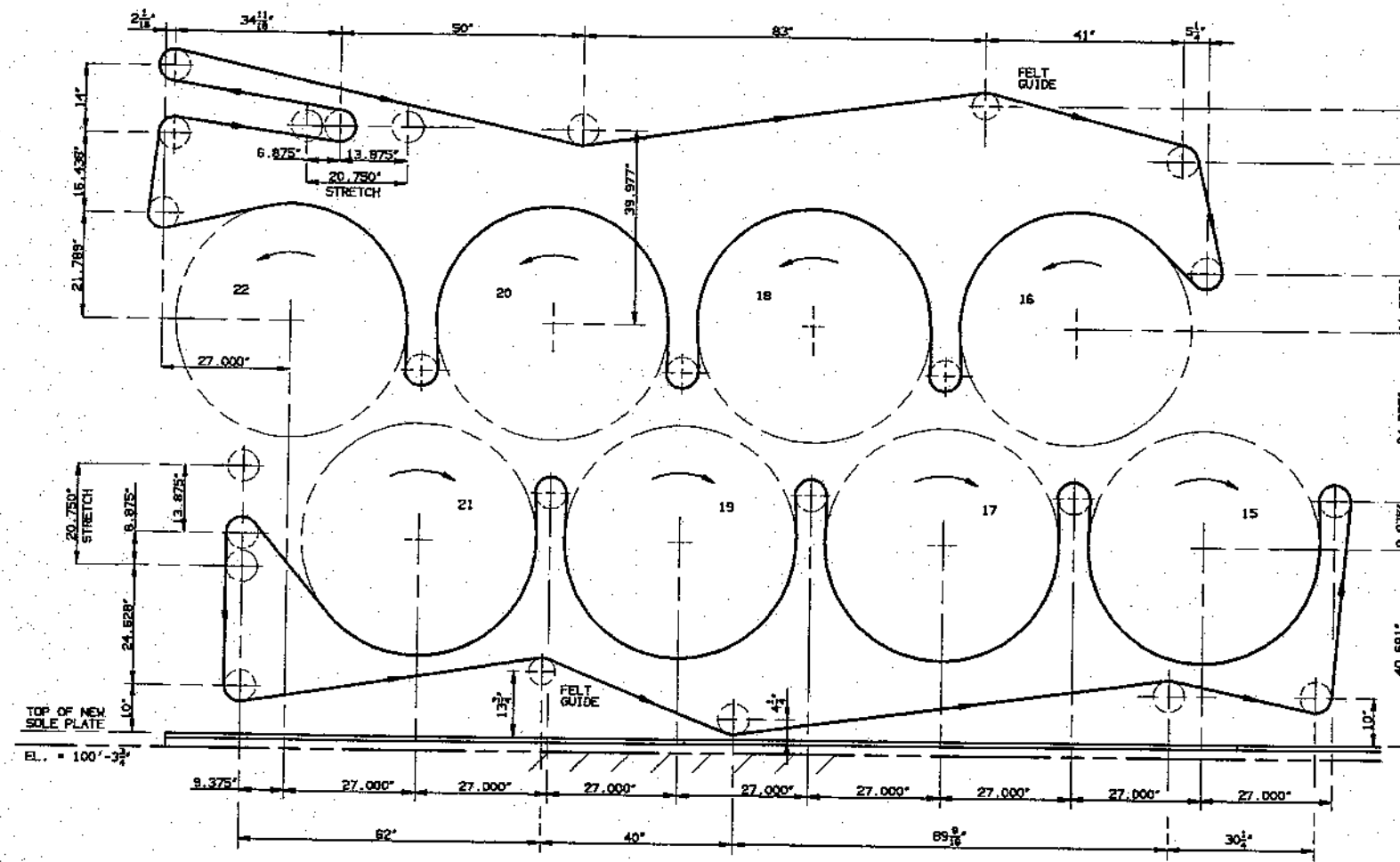
SECOND DRYER SECTION - PROPOSED FELT RUNS
