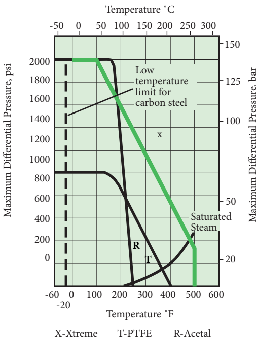
1/4" – 2" (DN 8 – 50) Standard Port
