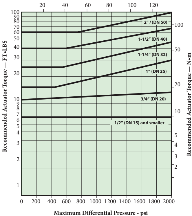
Acetal Seated Valves
