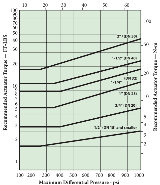
PTFE (T) Seated Valves
