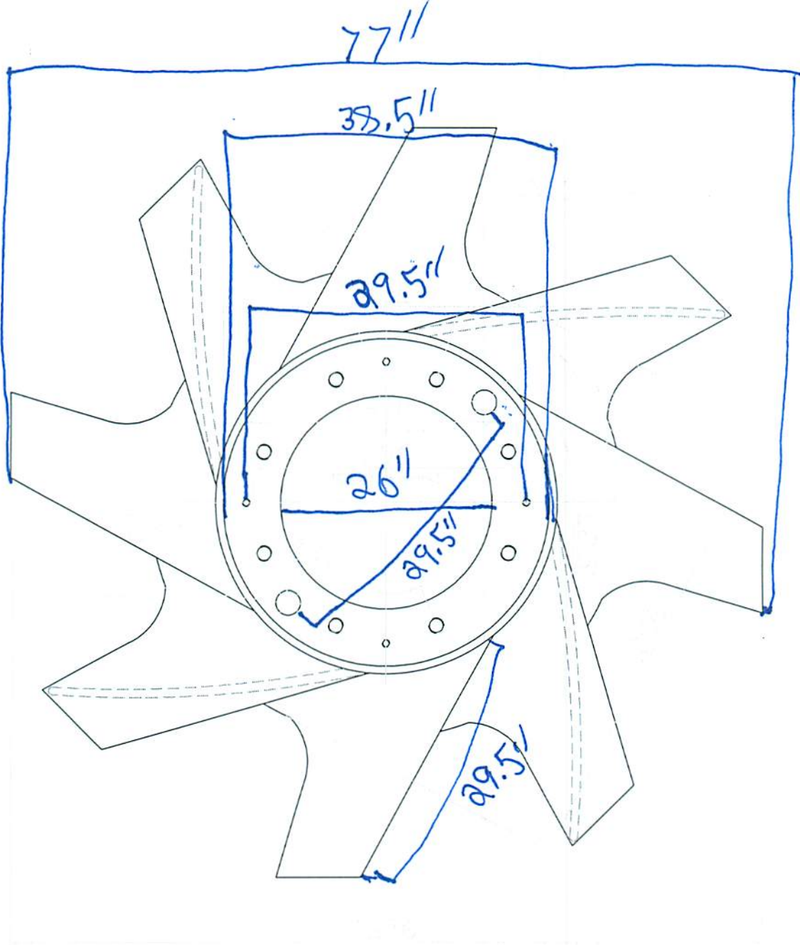
PULPER #4 VOKES ROTOR PLAN VIEW
