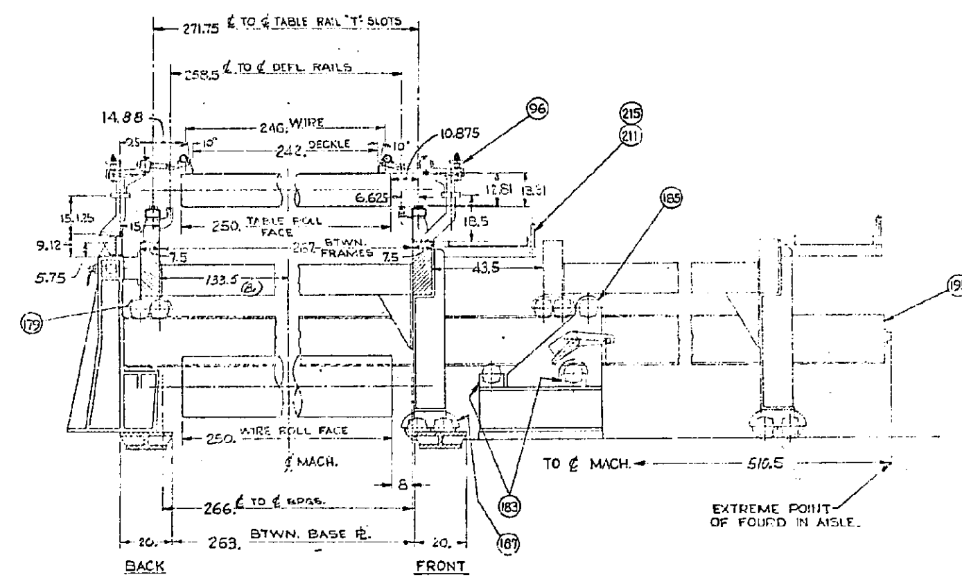
VIEW OF REMOVER BEAM FROM BREAST ROLL END
