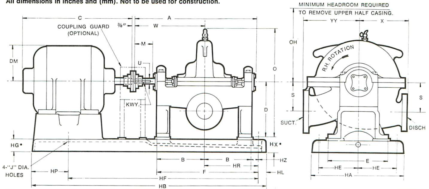
DIMENSIONS DETERMINED BY PUMP
