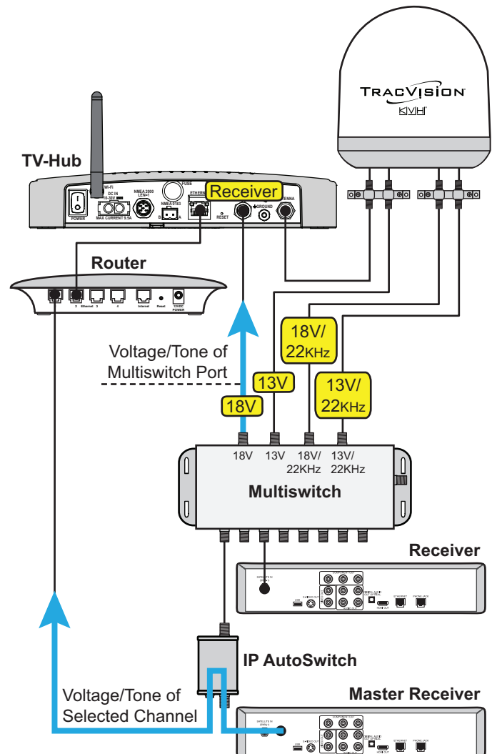
Figure 58: Linear Receivers with Multiswitch and IP AutoSwitch
