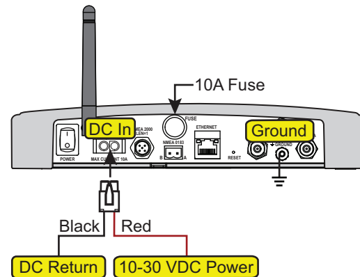
Figure 36: TracVision System Power
