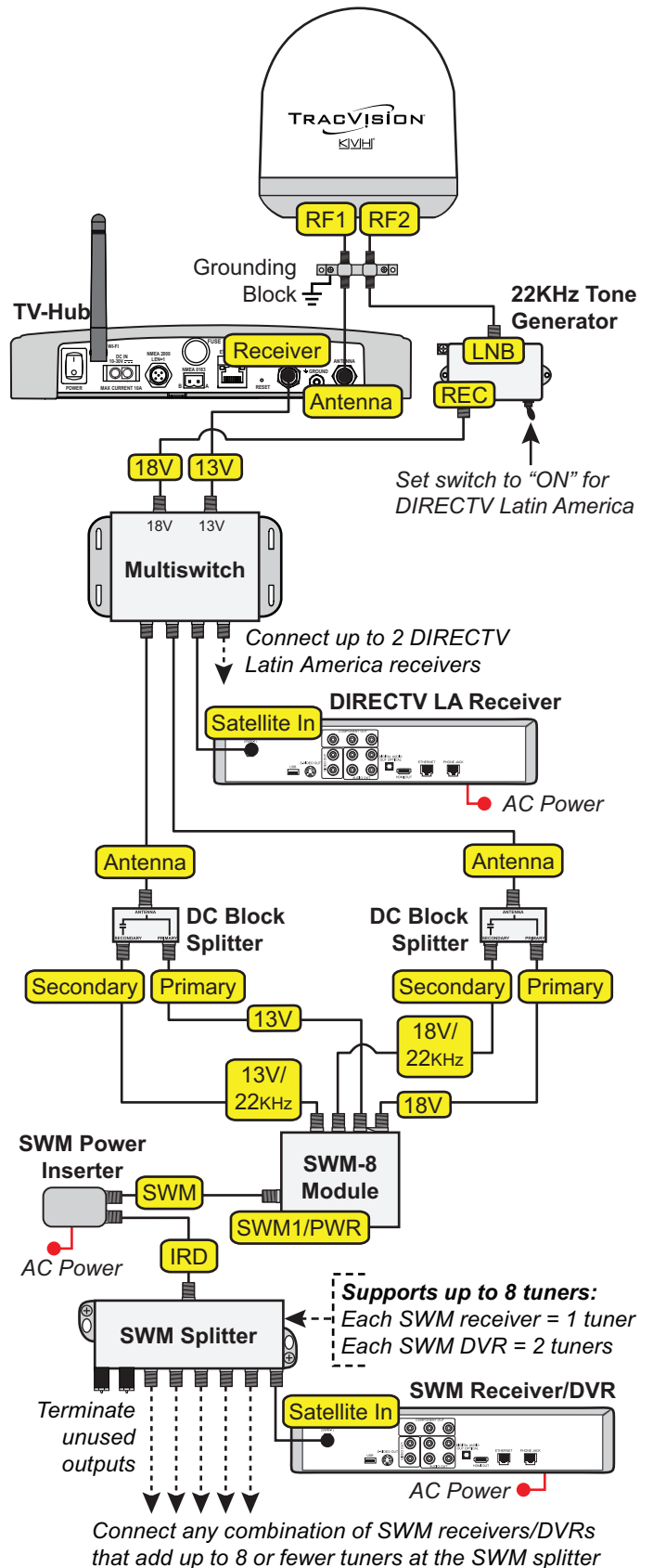
Figure 28: Wiring a Tri-Americas System
